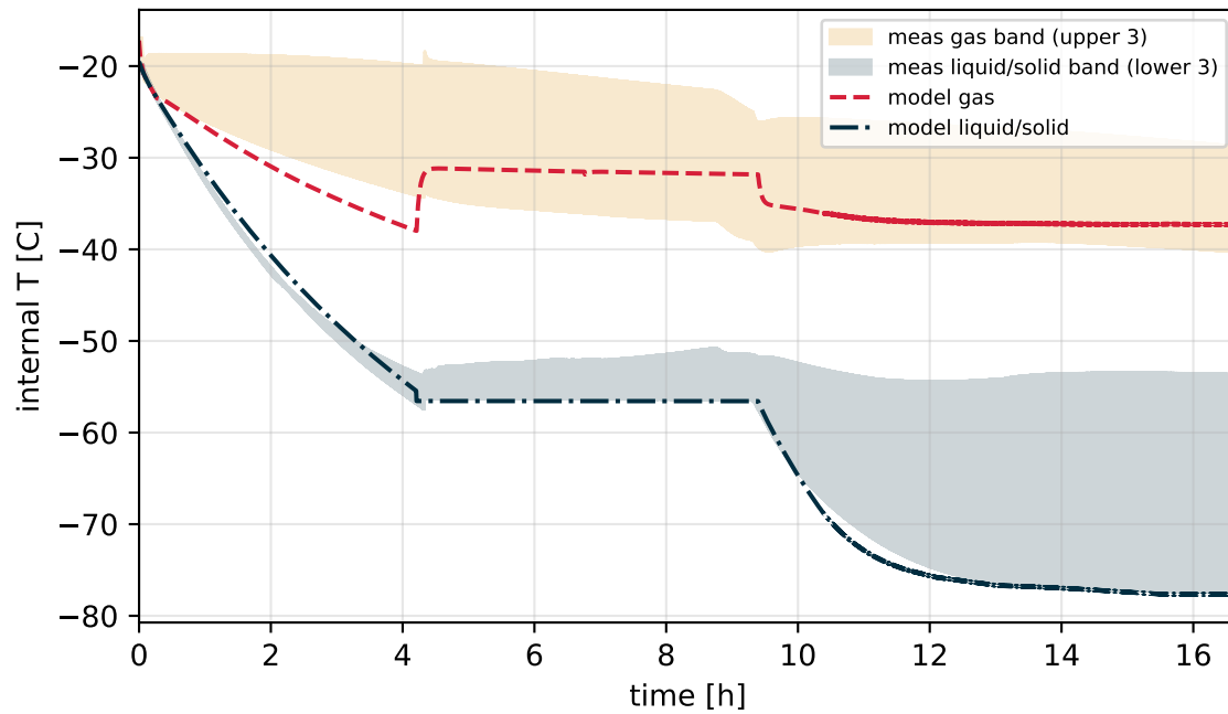
Internal temperature
