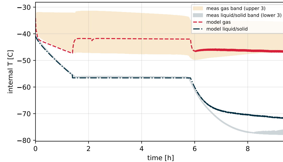
Internal temperature
