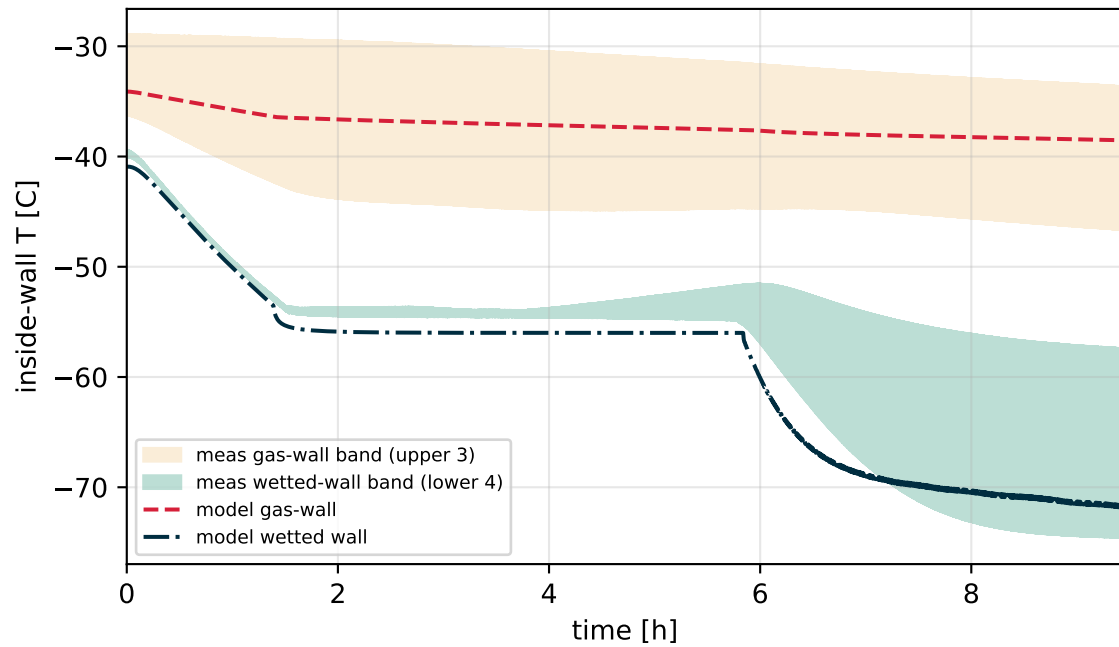
Wall temperature
