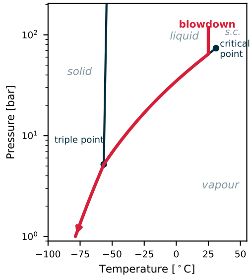
CO 2 phase diagram
