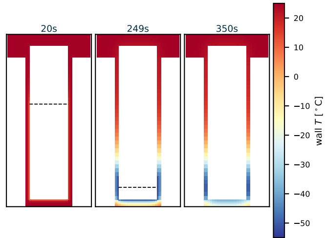
2-D wall temperature field
