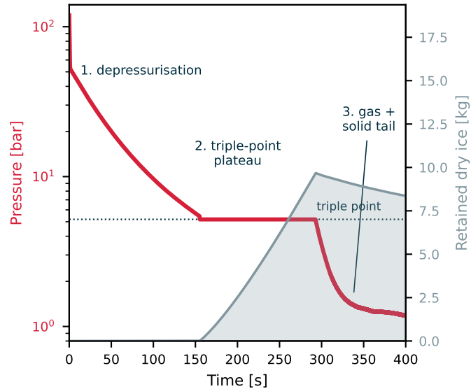
Gas-release blowdown fingerprint
