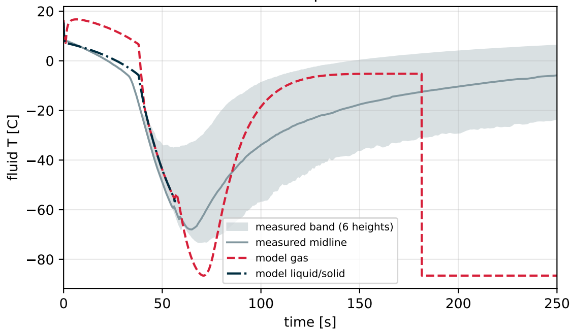
Fluid temperature
