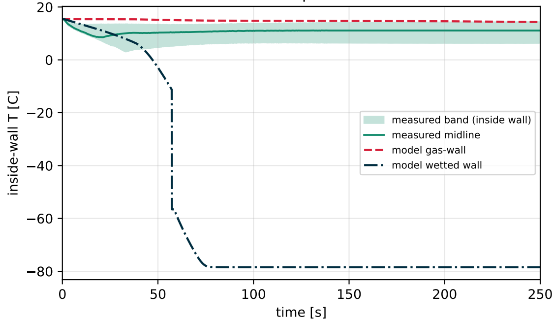
Wall temperature
