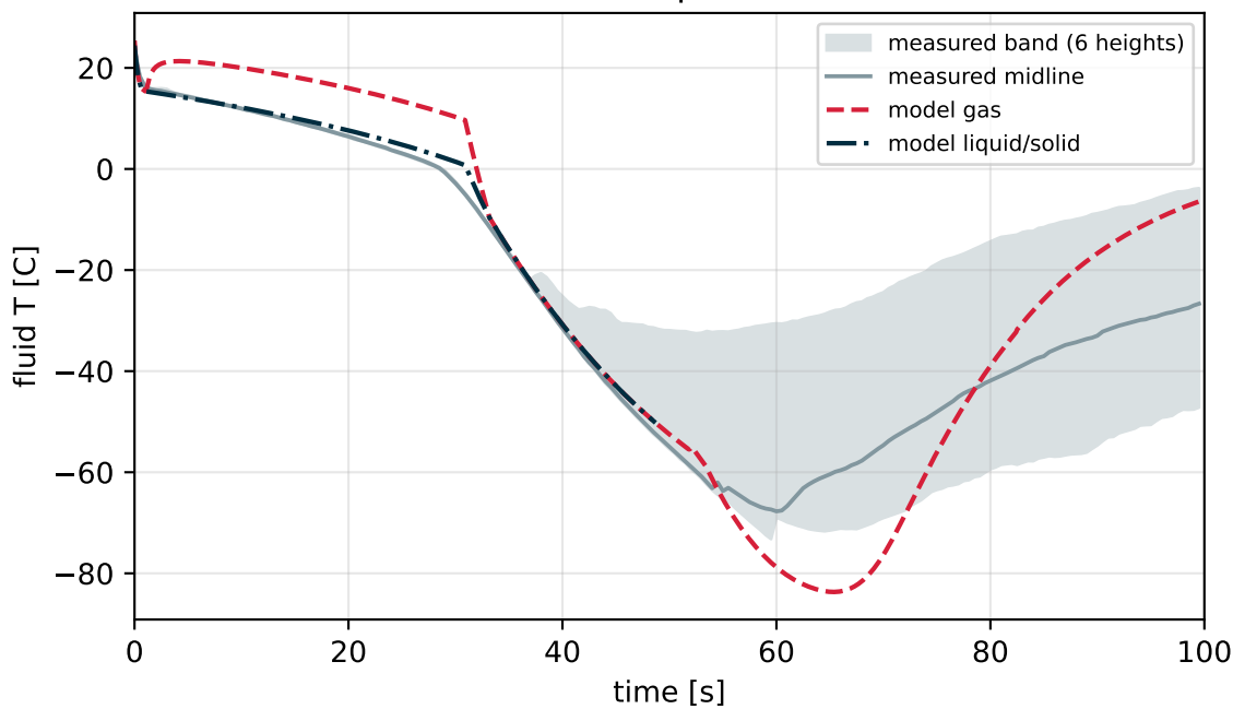
Fluid temperature
