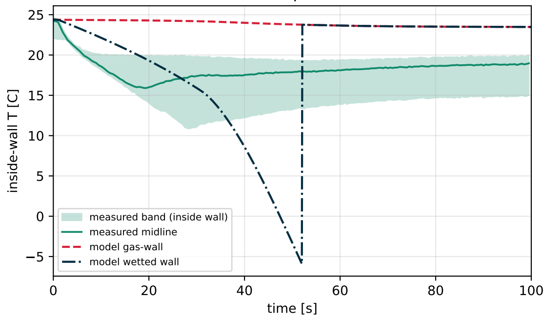
Wall temperature
