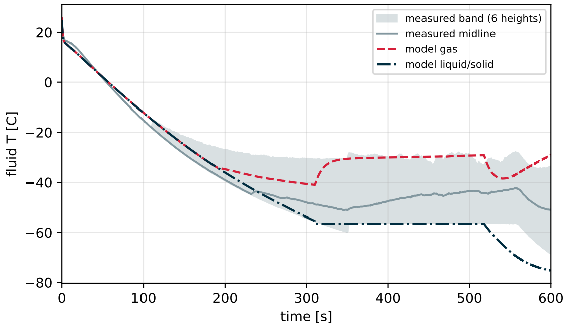
Fluid temperature
