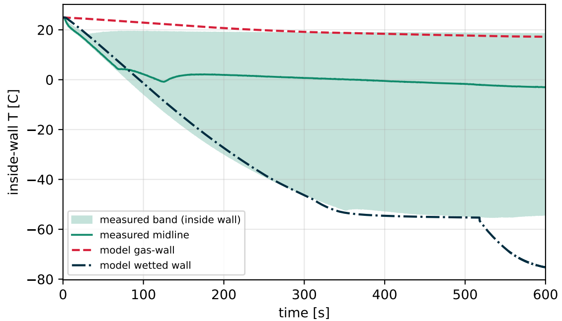
Wall temperature
