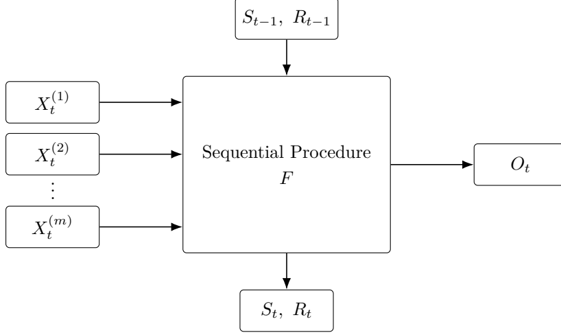
Figure 2: A procedure consumes logically distinct statistical inputs, any non-empty subset of which may be present at a step. It receives statistical inputs, not physical streams.
