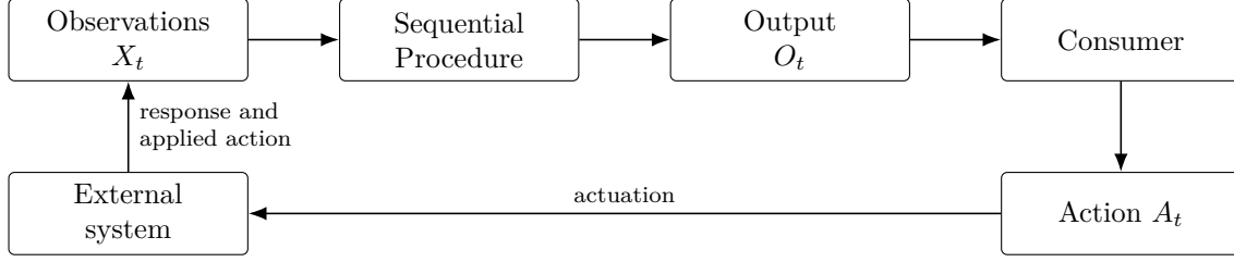
Figure 5: Inference and action are separated. The loop closes through the external system. An action that influences later observations is itself recorded.
