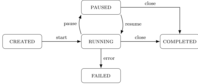
Figure 4: Run lifecycle. A run restored from a checkpoint starts in PAUSED, and attaching a runtime resumes it. A failed run is never continued in place; recovery restores an earlier checkpoint.
