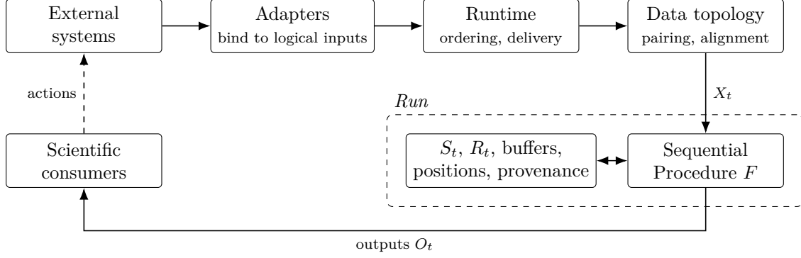
Figure 1: The data path. The run is not a stage on the path: it is the context that owns everything which must outlive the executing process. Actions return to the external world, never directly to the procedure.
