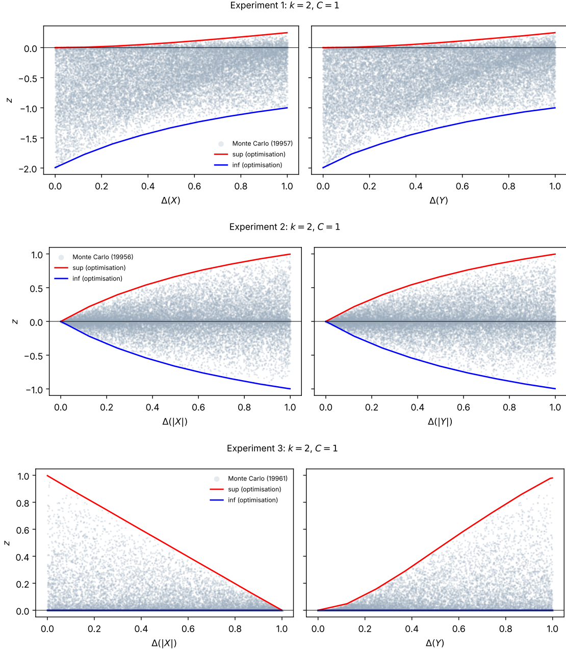
Figure 3: Envelopes from constrained optimisation versus sampling for the three trace functionals ( k = 2, C = 1 ; one row per experiment). Horizontal axis: Michelson contrast of the first operator (left) or of the second operator (right); vertical axis: z for operators normalised to \lambda_{\max} = 1 . Grey: the Monte Carlo samples of [1]; red and blue: the upper and lower envelopes found by constrained optimisation, the other contrast being free. In this smallest case the samples come close to the envelopes (the samples outside after re-optimisation are counted in Table 9), which is no longer so for two sectors or larger blocks (Tables 8 and 9). In Exp. 1 the region z > 0 (violation of |\text{Tr}(XUY)| \leq \text{Tr}(XY) ) extends to the value of \sup z in Table 9; in Exp. 3 the lower envelope is the proven bound z \geq 0 .
