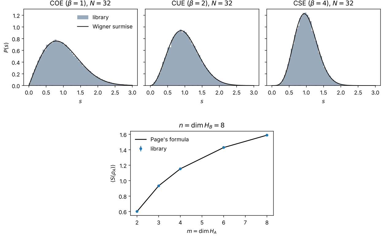
Figure 1: Top: nearest-neighbour spacings of COE, CUE and CSE eigenphases generated by the library ( n = 32 , 2000 matrices per ensemble), against the Wigner surmise. Bottom: mean entanglement entropy of random pure states against Page's formula (5000 states per point) (error bars: two standard errors).
