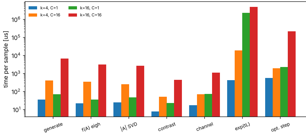
Figure 6: Time per sample (logarithmic axis) of the operations of Table 13, one bar per configuration (k, C) .
