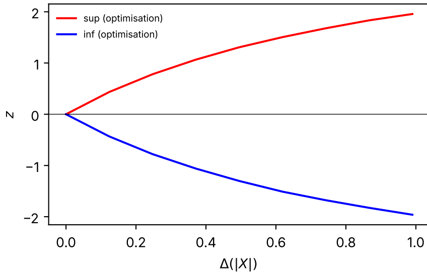
Experiment 2: k = 4, C = 1
