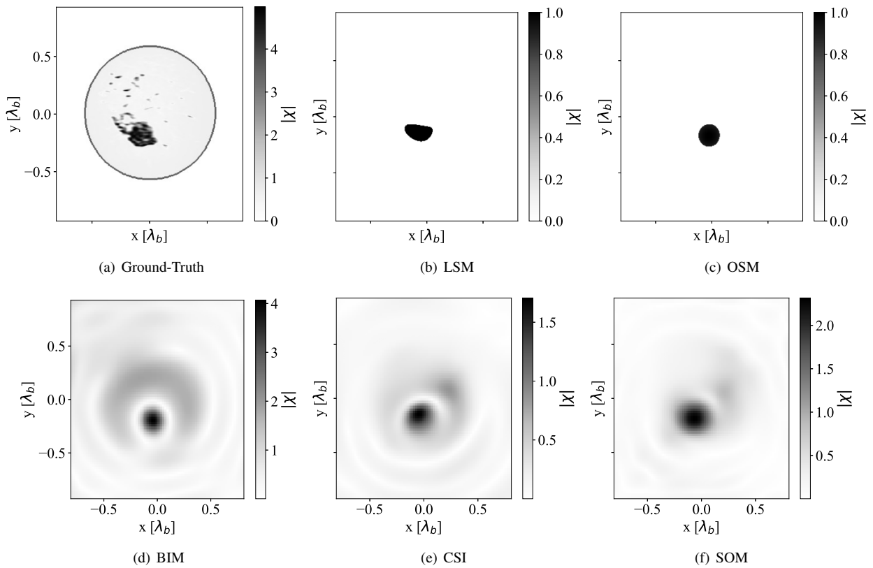
FIGURE 11. Breast phantom study: ground-truth and reconstructed images by each algorithm.
