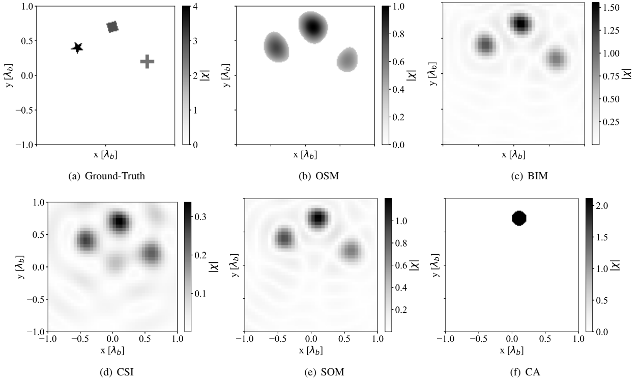
FIGURE 8. Position detection study, multiple scatterer: ground-truth and reconstructed images by each algorithm.
