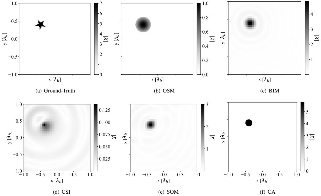
FIGURE 7. Position detection study, single scatterer: ground-truth and reconstructed images by each algorithm.
