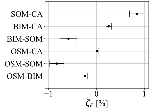
FIGURE 10. Position detection study, average performance: Confidence intervals (95%) for the position error indicator \zeta_P for each pair of algorithms.
