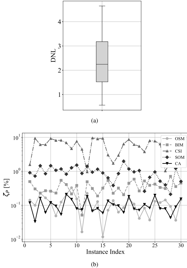
FIGURE 9. Position detection study, average performance: (a) Degree of Nonlinearity (DNL) for each scatterer; (b) position error indicator \zeta_P for each algorithm in each instance.
