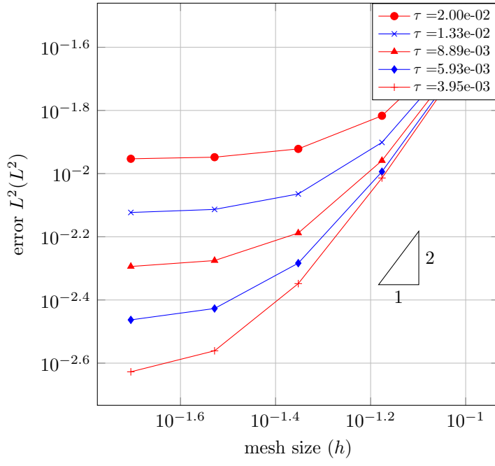
Space convergence
