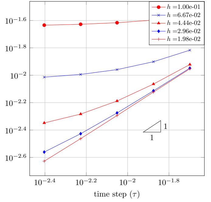
Time convergence
