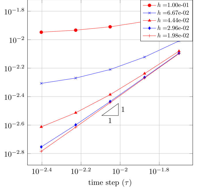
Time convergence
