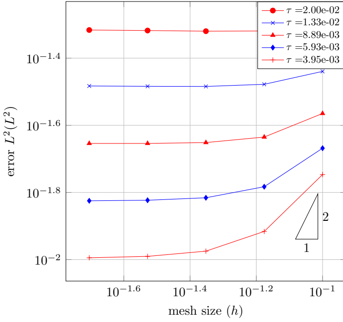
Space convergence
