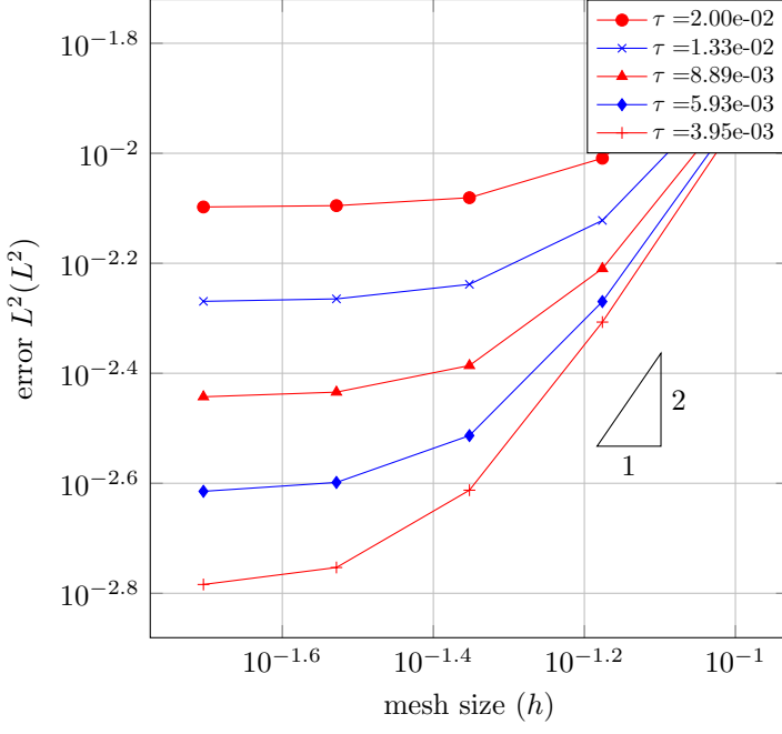
Space convergence
