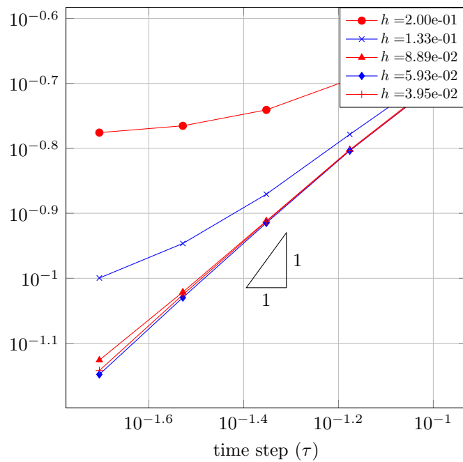
Time convergence
