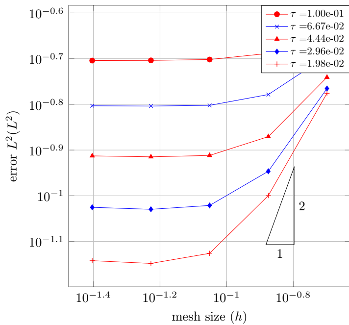
Space convergence
