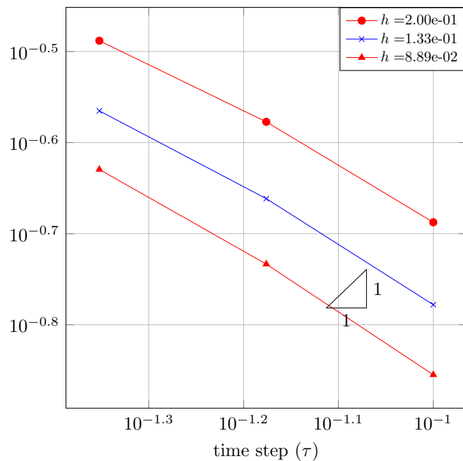
Time convergence
