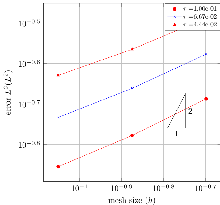
Space convergence
