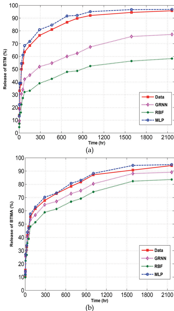
Fig. 18. Estimated release profiles and experimental release profiles of (a) BTM (b) BTMA for one sample.
