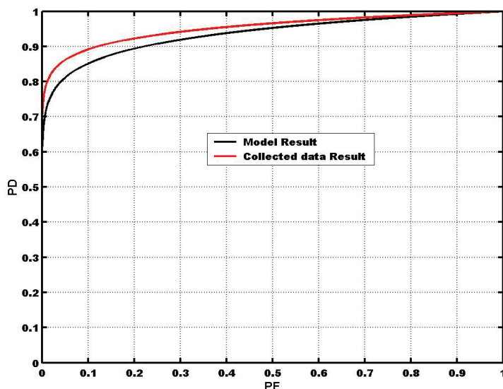
Fig. 9. ROC curves for Vulgar diagnosis
