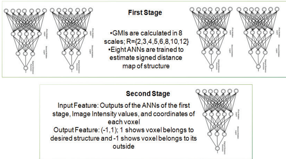
Fig. 6. A flowchart of the two-stage method.
