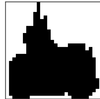
Reconstructed
