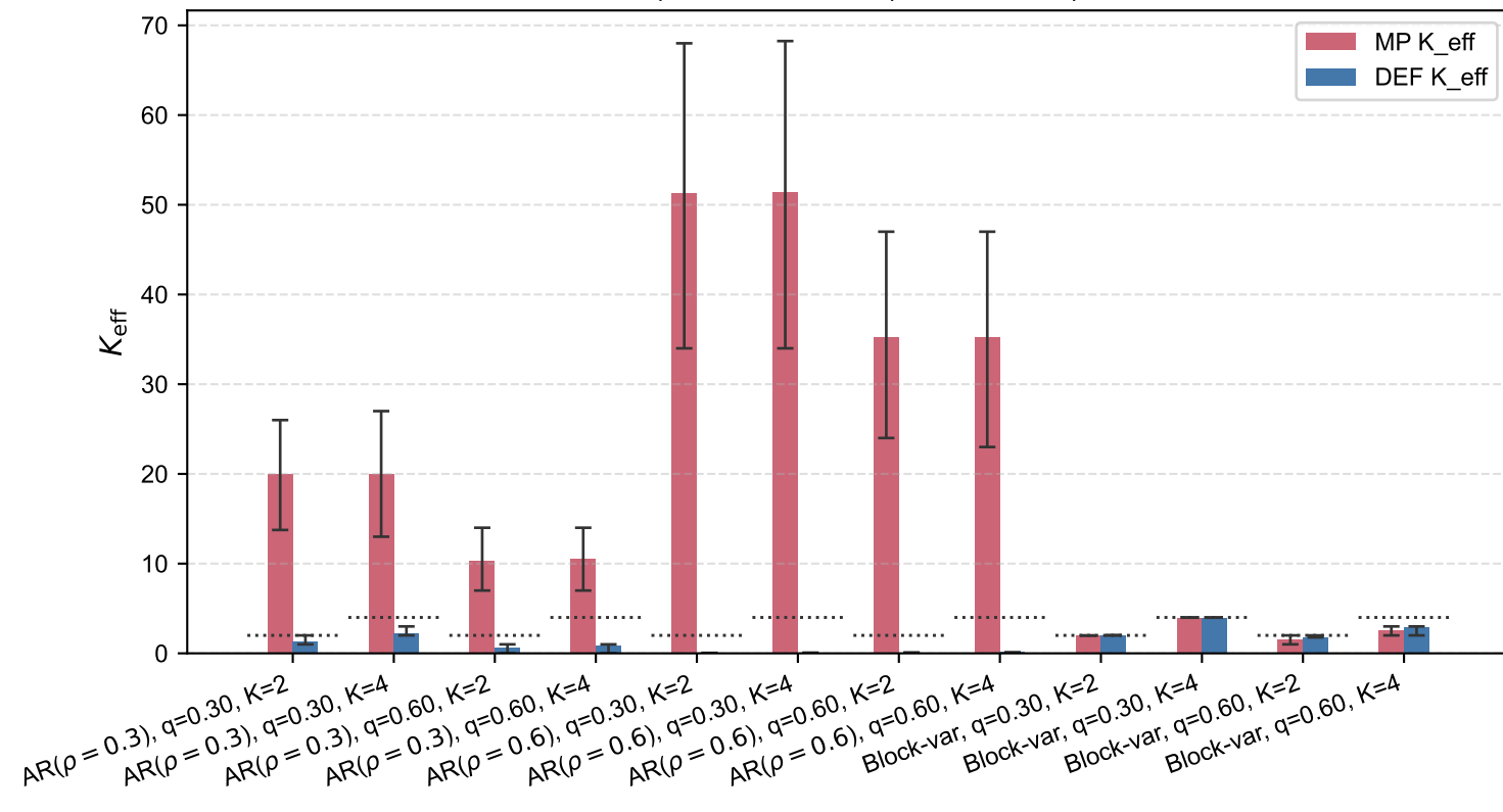
9C) Effective rank (mean \pm IQR)
