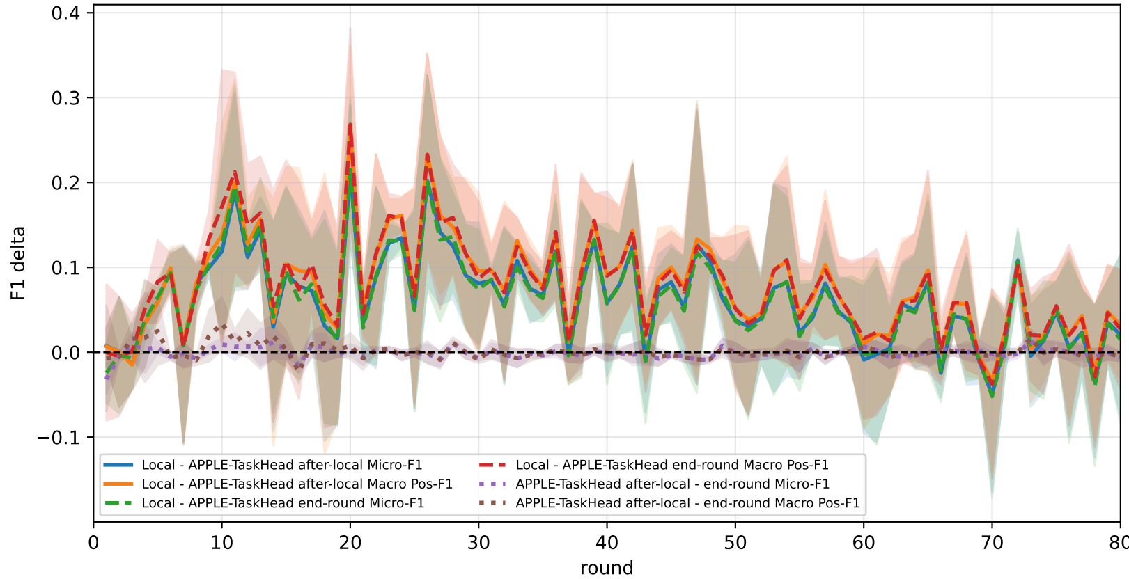
Delta diagnostics: Local gap and APPLE-TaskHead mismatch gap
