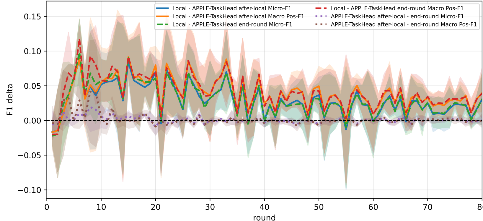
Delta diagnostics: Local gap and APPLE-TaskHead mismatch gap
