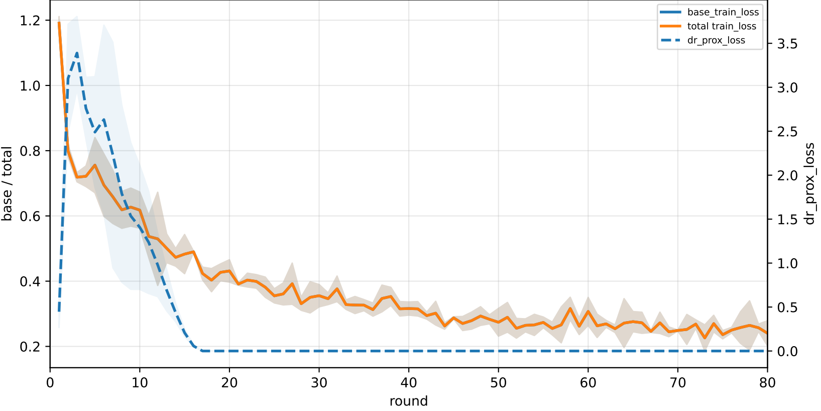
q_task_cycle6 | graph_id=3000004
