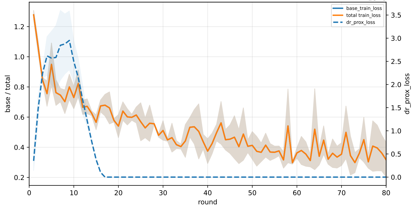
q_task_cycle6 | graph_id=3000014
