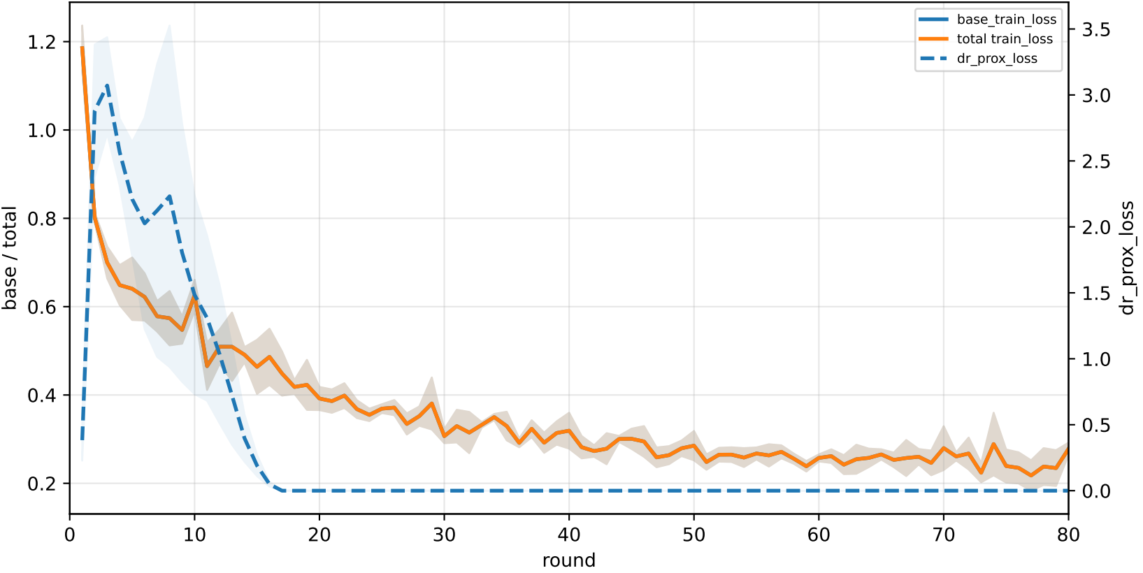
q_task_cycle2 | graph_id=3000000
