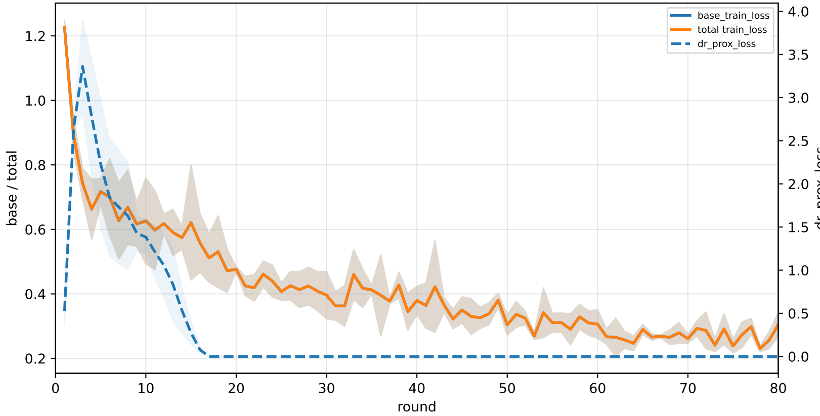
q_task_cycle3 | graph_id=3000006
