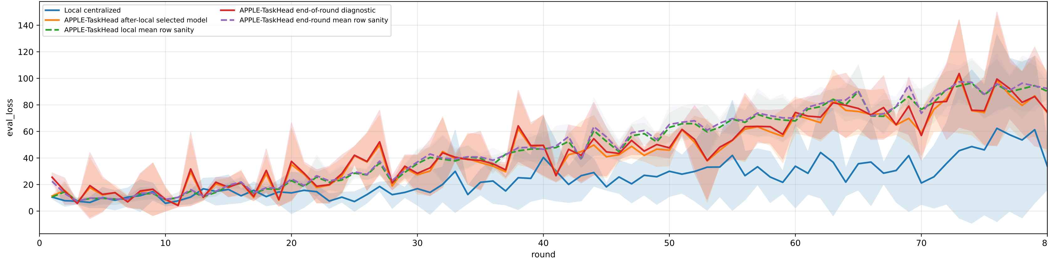
Validation loss: selected APPLE-TaskHead vs end-of-round mismatch (rounds=80)
