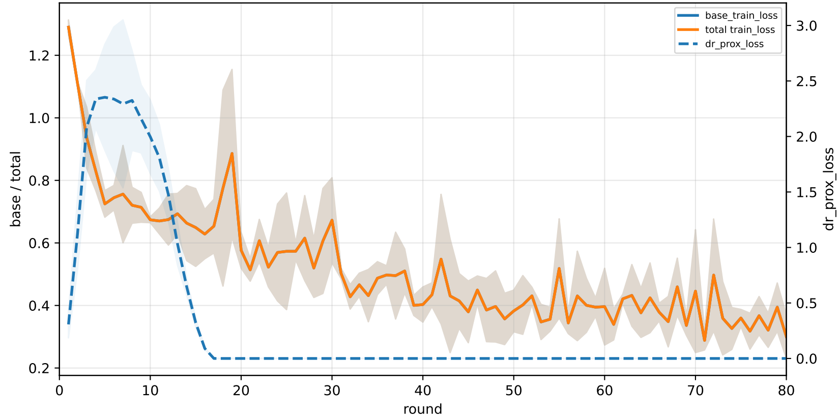
q_task_cycle4 | graph_id=3000012
