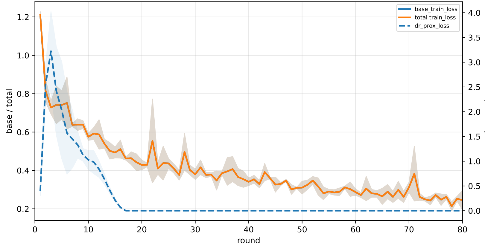
q_task_cycle4 | graph_id=3000007
