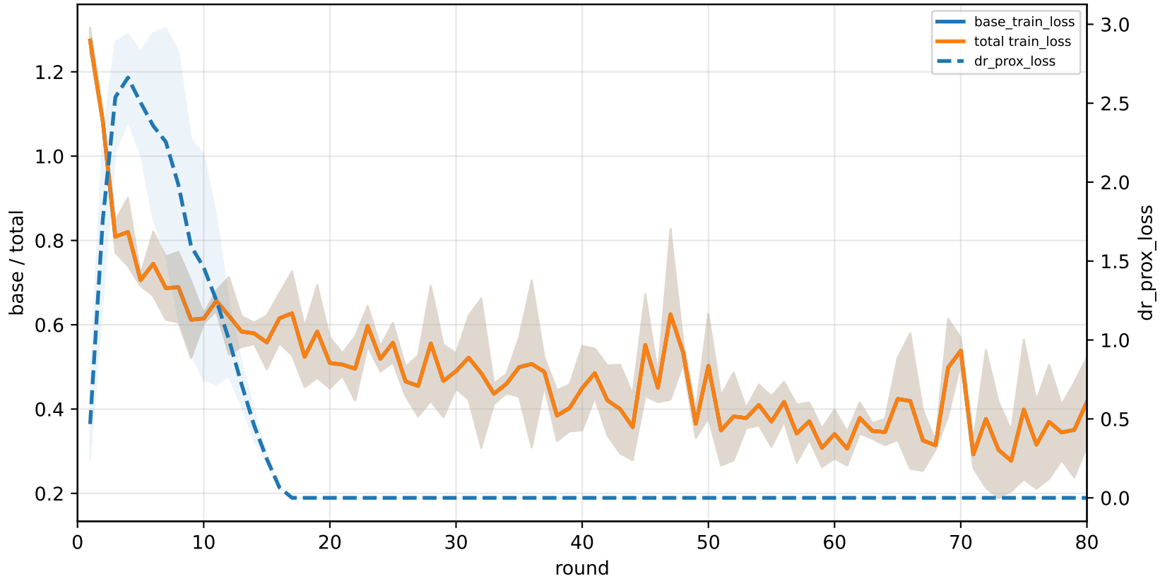
q_task_cycle3 | graph_id=3000011
