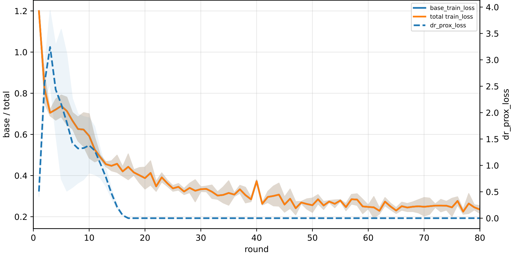
q_task_cycle5 | graph_id=3000003
