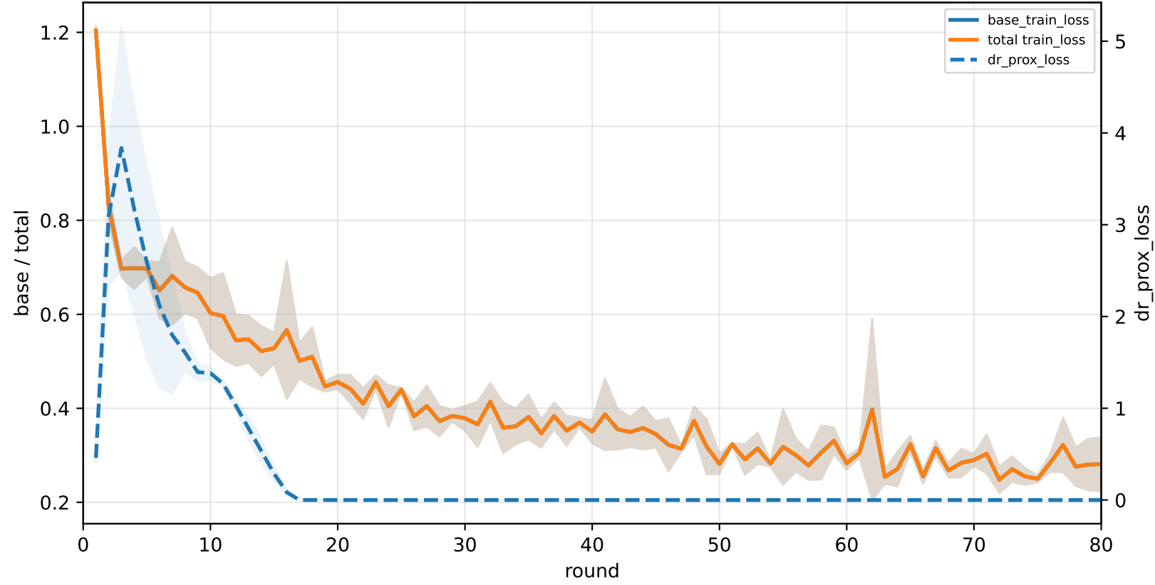
q_task_cycle6 | graph_id=3000009
