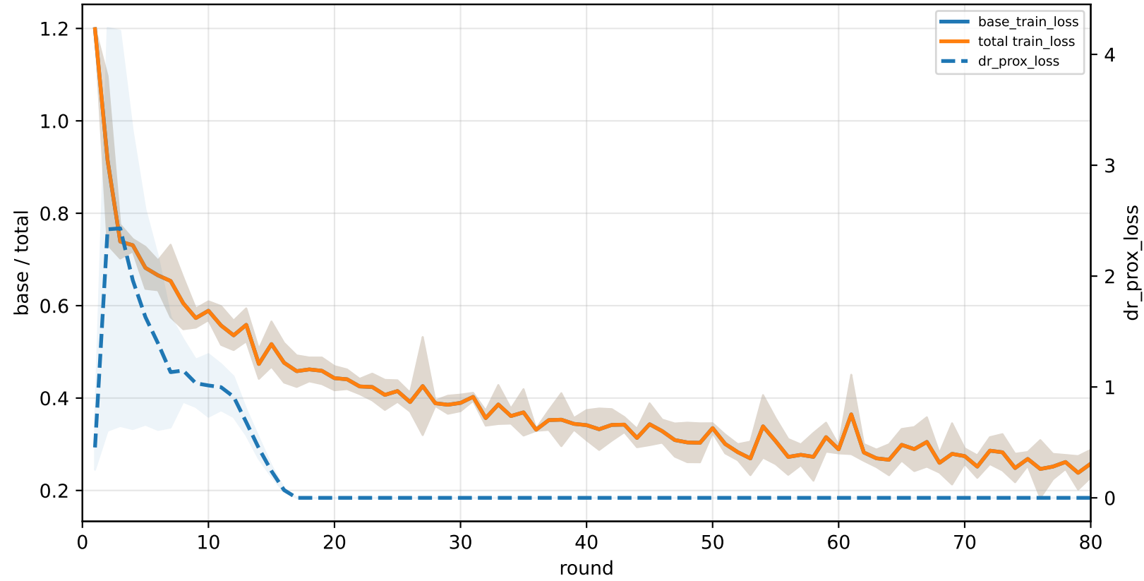
q_task_cycle2 | graph_id=3000005
