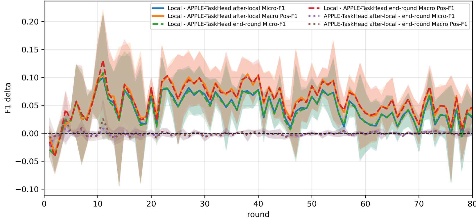
Delta diagnostics: Local gap and APPLE-TaskHead mismatch gap
