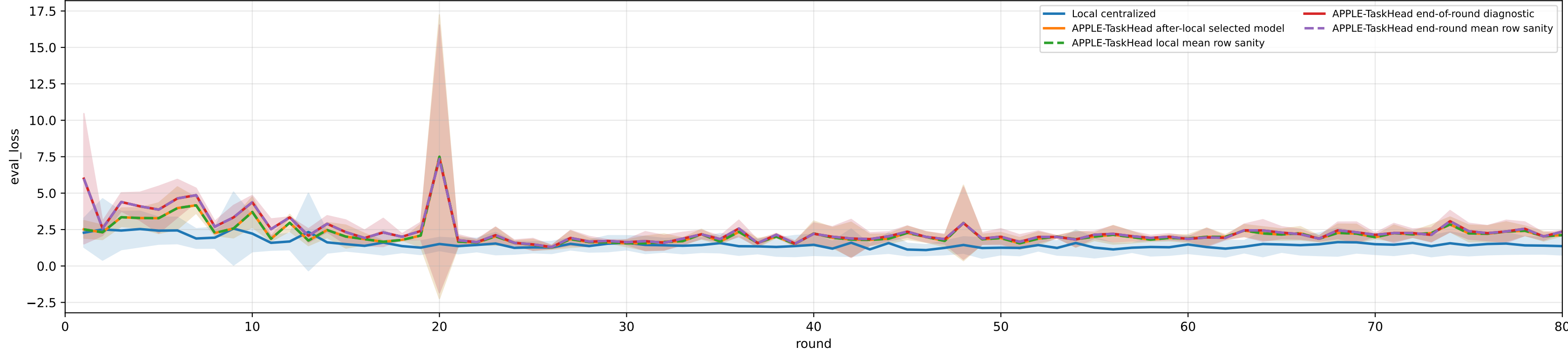
Validation loss: selected APPLE-TaskHead vs end-of-round mismatch (rounds=80)
