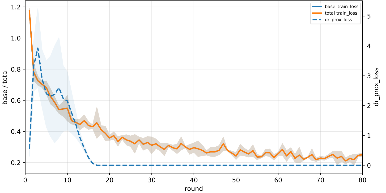
q_task_cycle3 | graph_id=3000001
