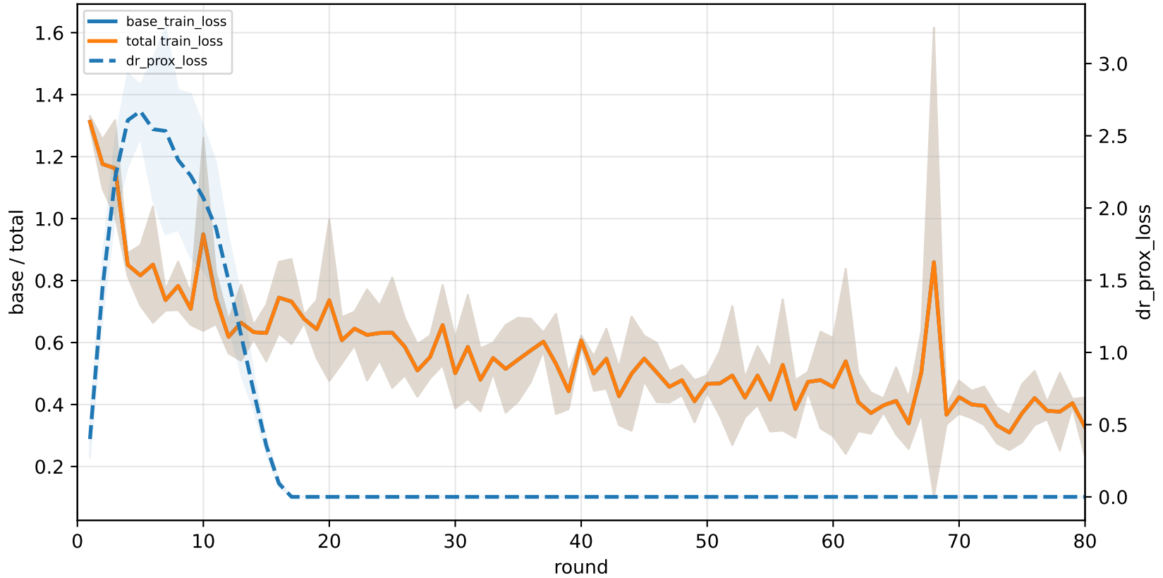
q_task_cycle5 | graph_id=3000013
