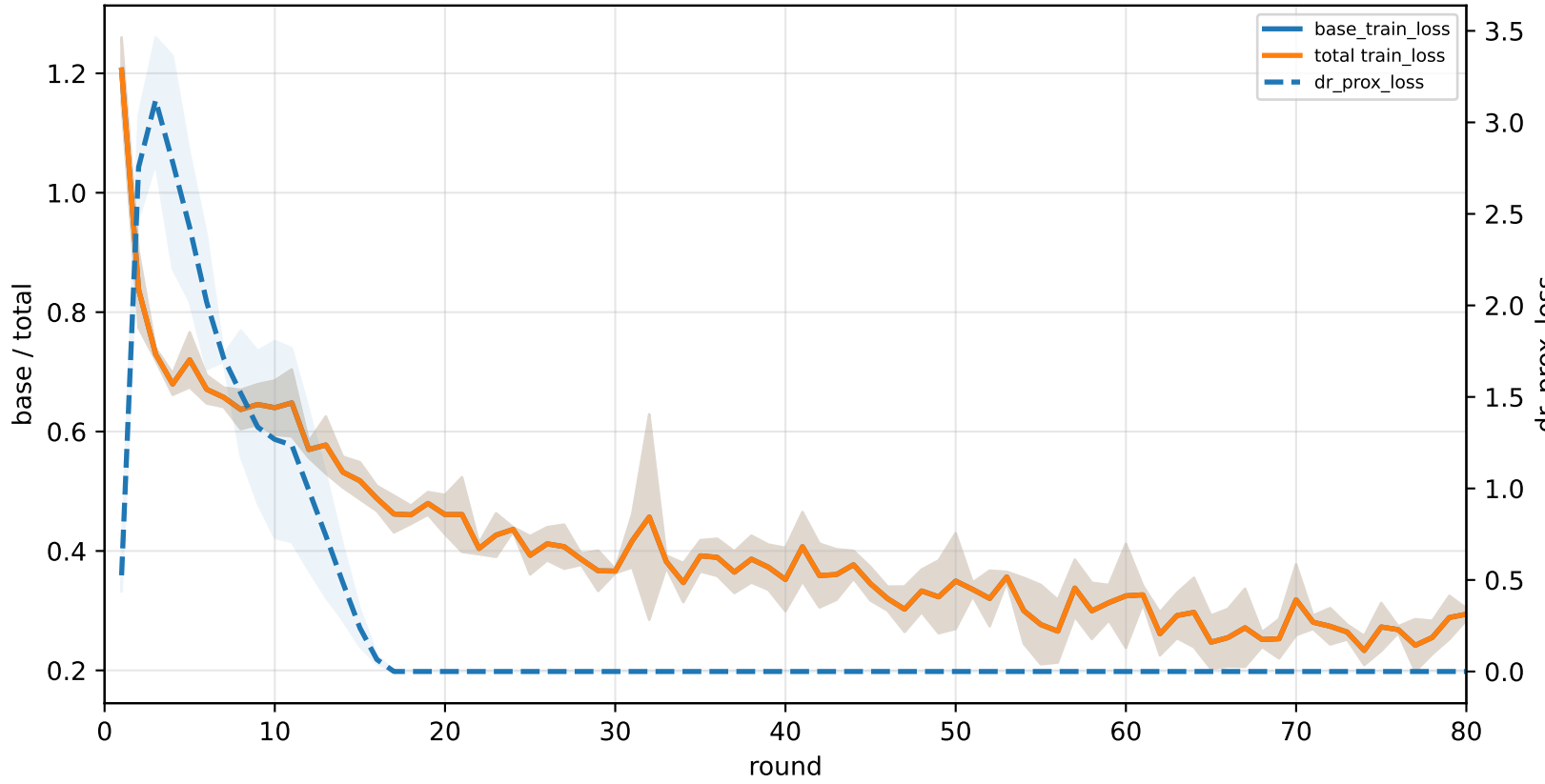
q_task_cycle5 | graph_id=3000008
