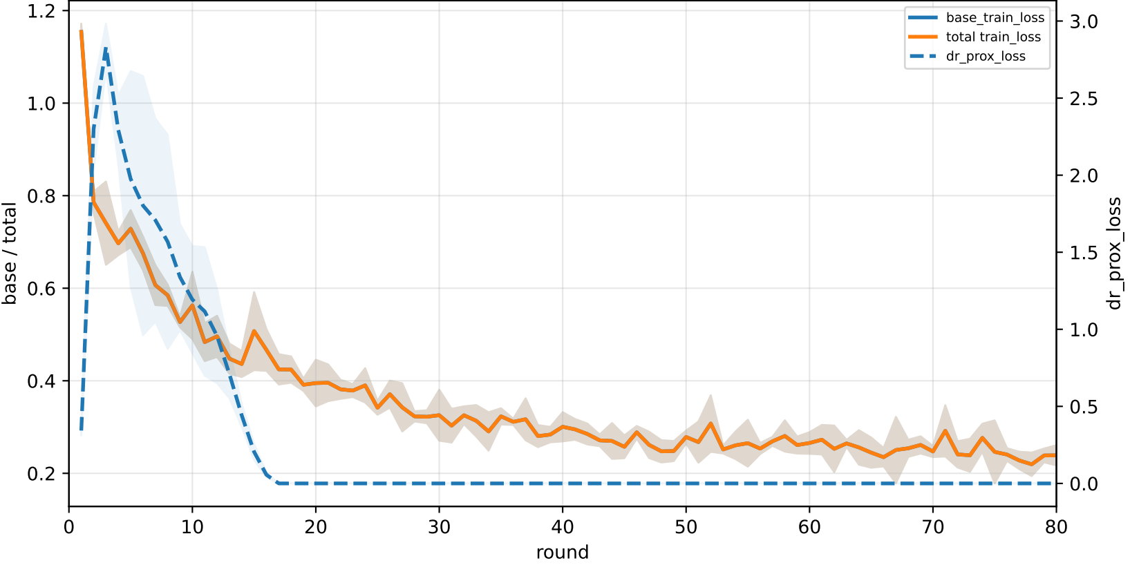
q_task_cycle4 | graph_id=3000002
