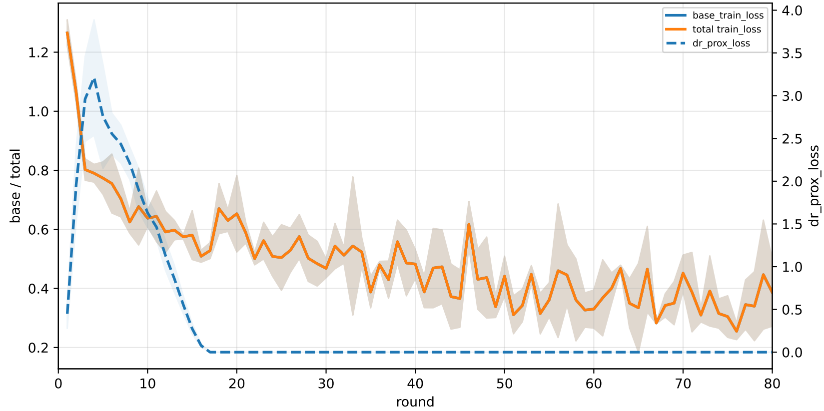
q_task_cycle2 | graph_id=3000010
