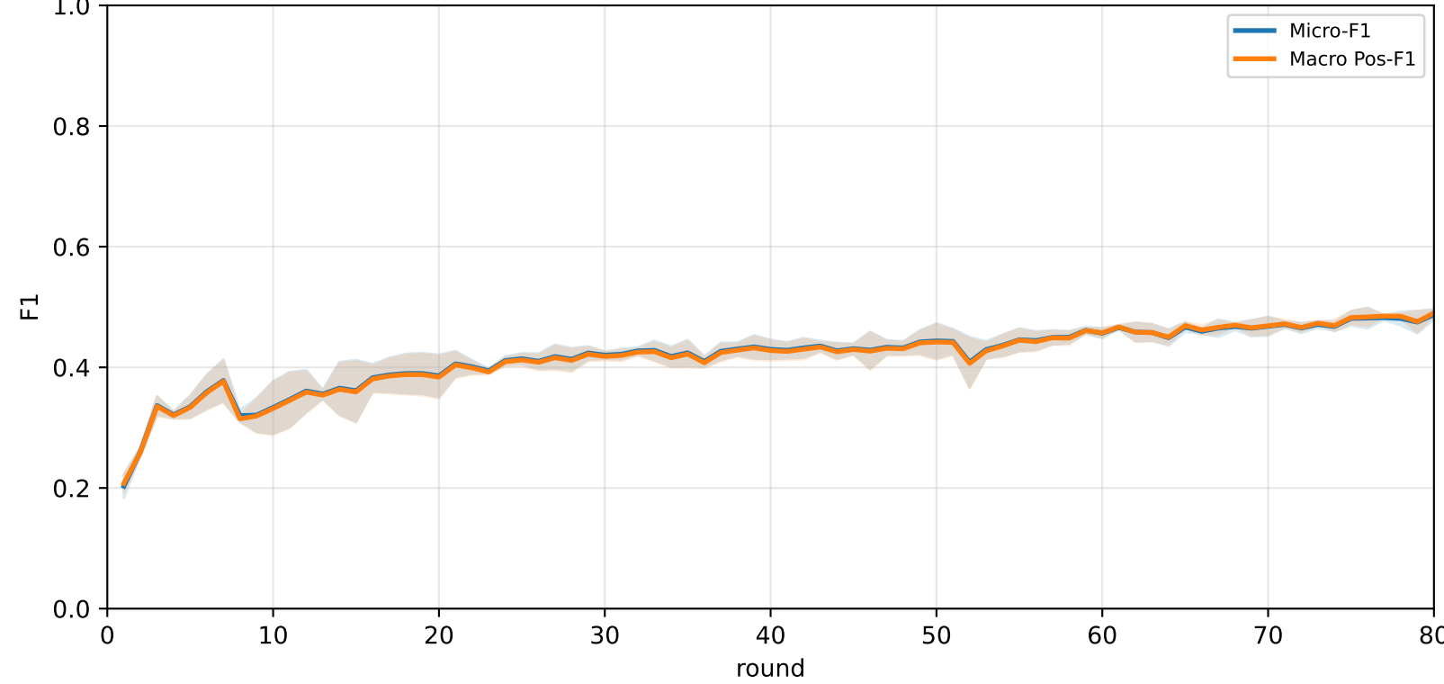
Pooled APPLE micro / macro F1 (after-local selected model)
