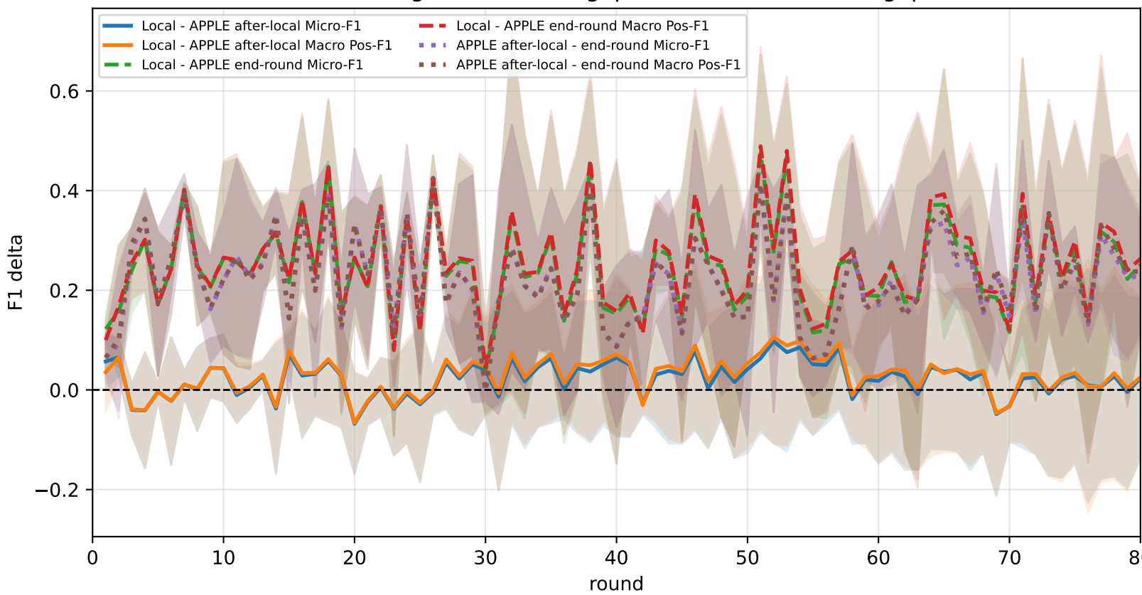
Delta diagnostics: Local gap and APPLE mismatch gap
