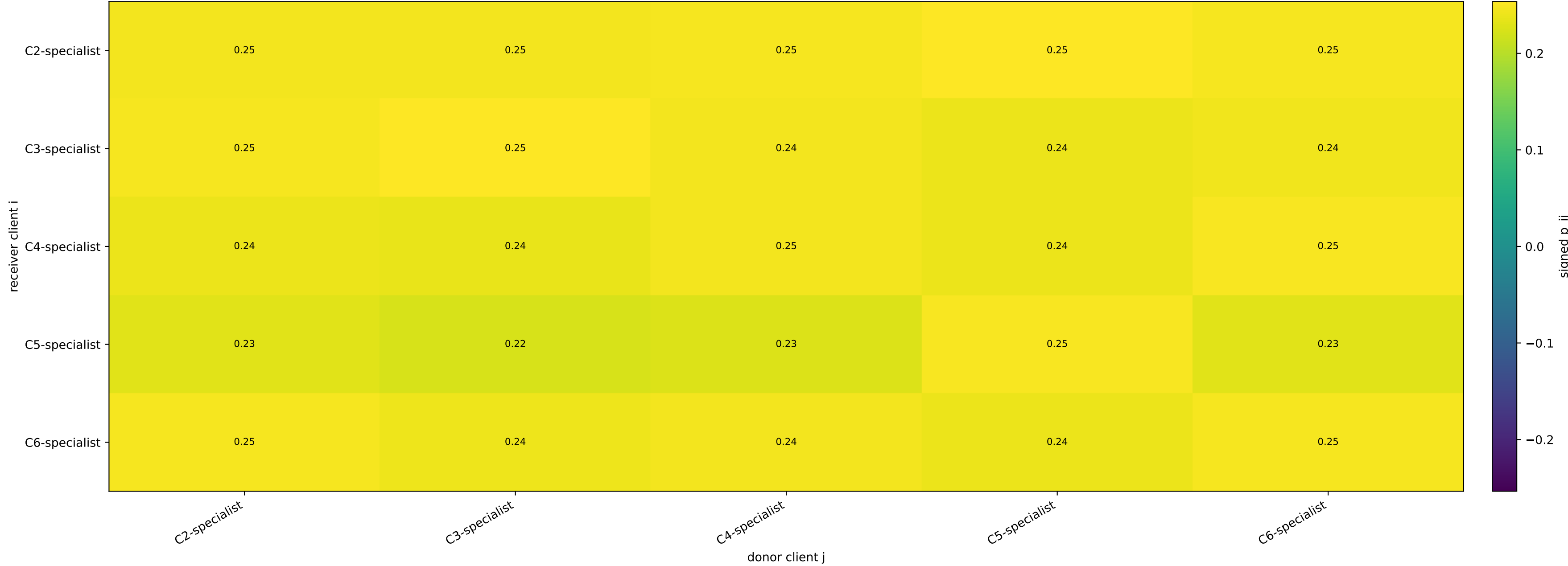
Selected-best-round APPLE DR coefficients p_{ij} , mean over seeds
