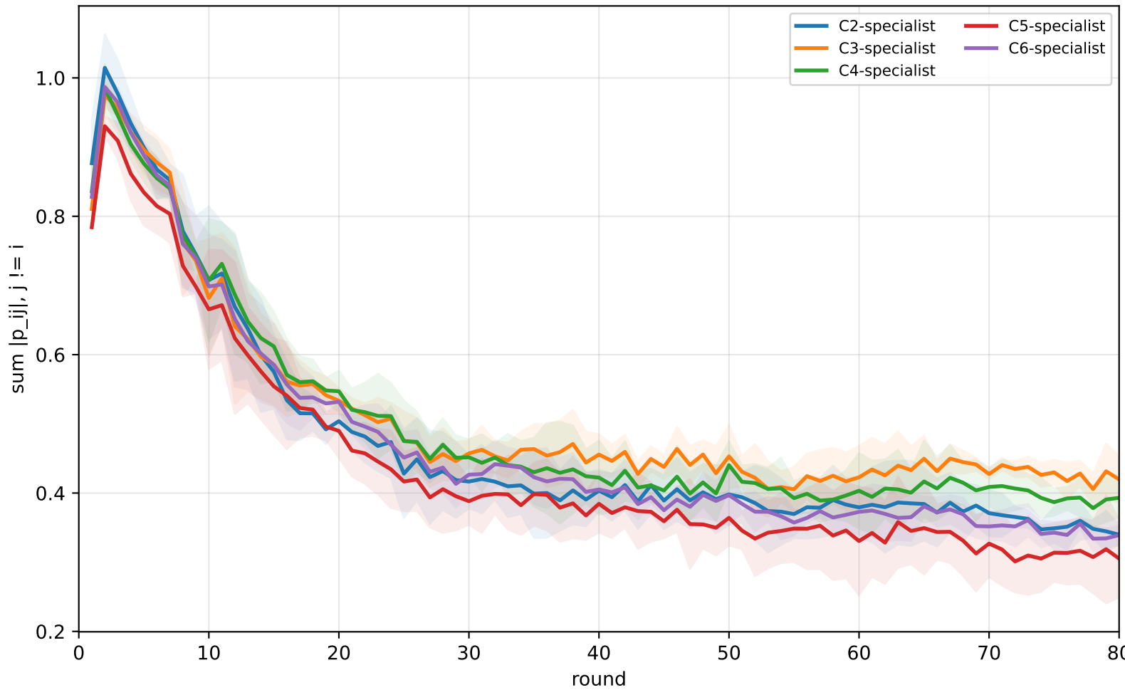
APPLE off-diagonal absolute mass over rounds
