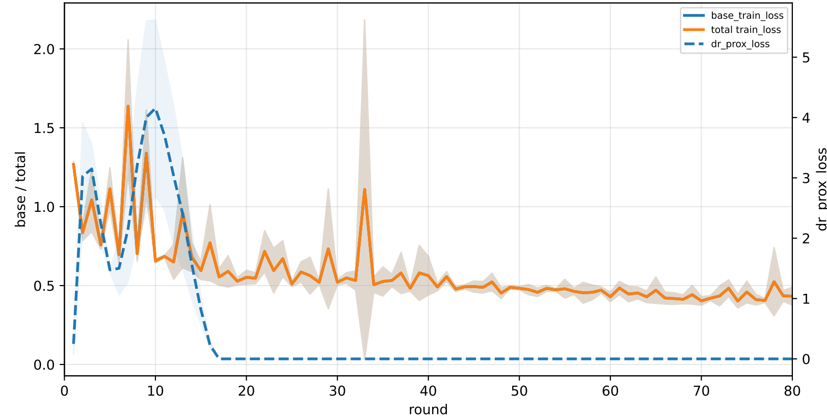
C5-specialist | graph_id=3000003
