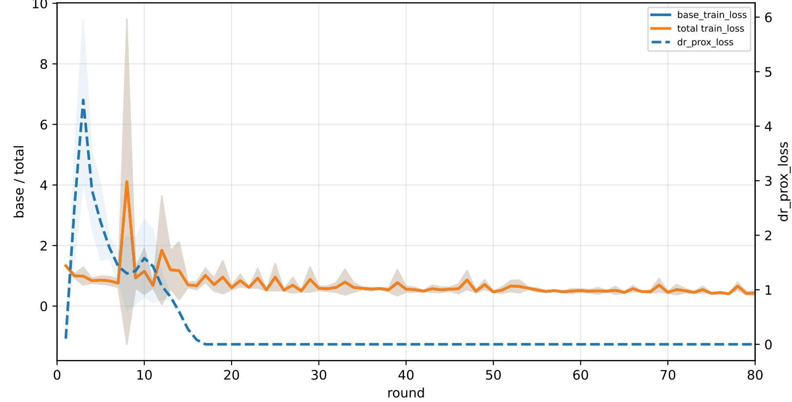
C4-specialist | graph_id=3000012
