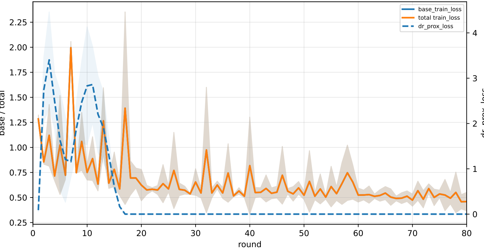
C5-specialist | graph_id=3000008
