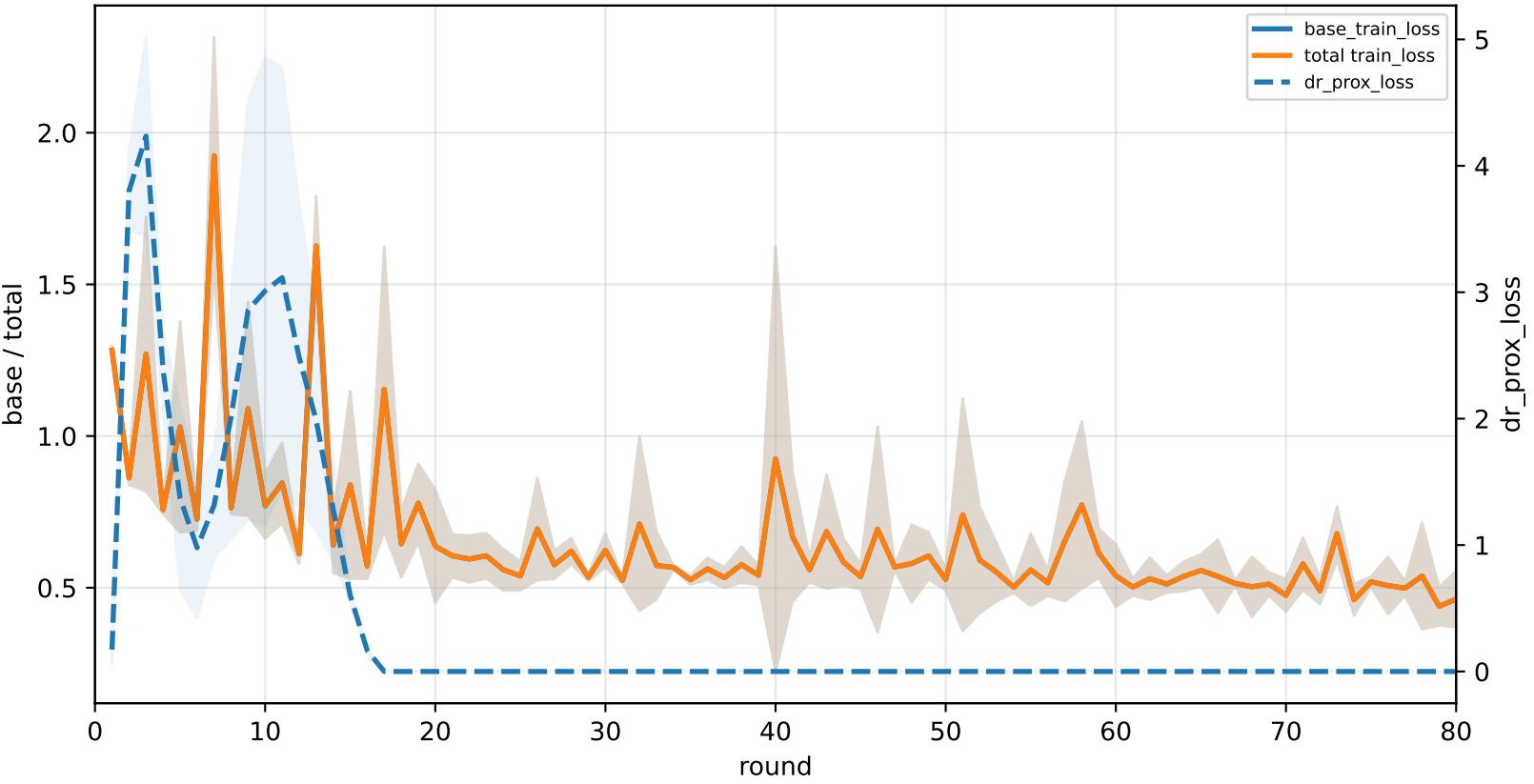
C4-specialist | graph_id=3000007
