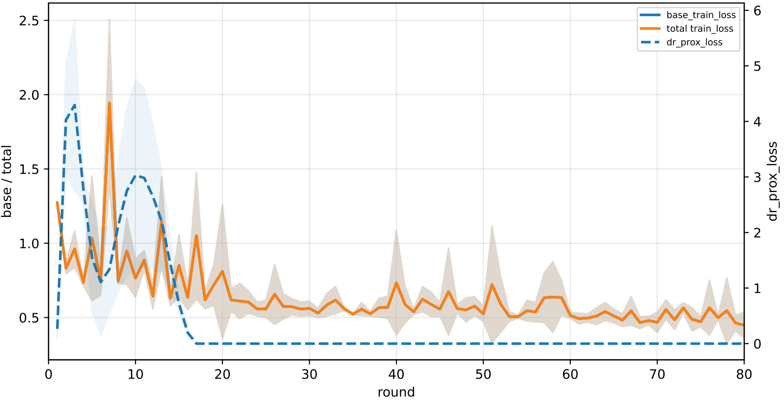
C2-specialist | graph_id=3000005
