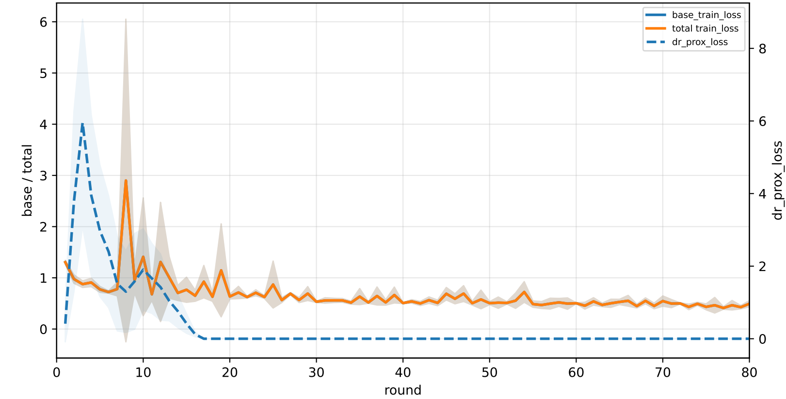
C2-specialist | graph_id=3000010
