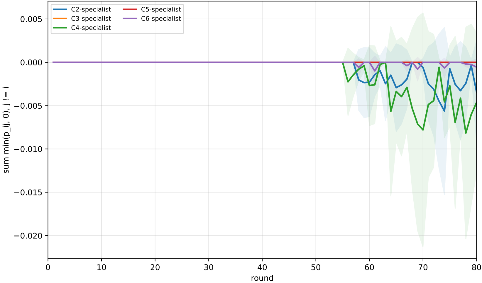
APPLE off-diagonal negative mass over rounds
