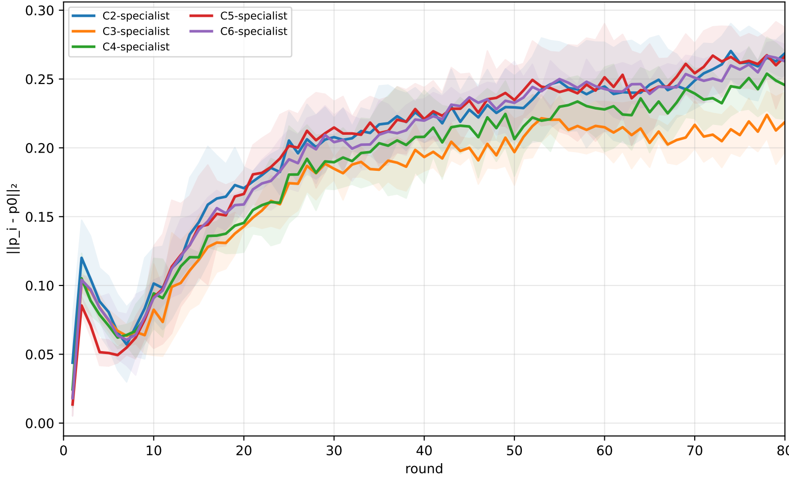
APPLE DR movement away from p_0
