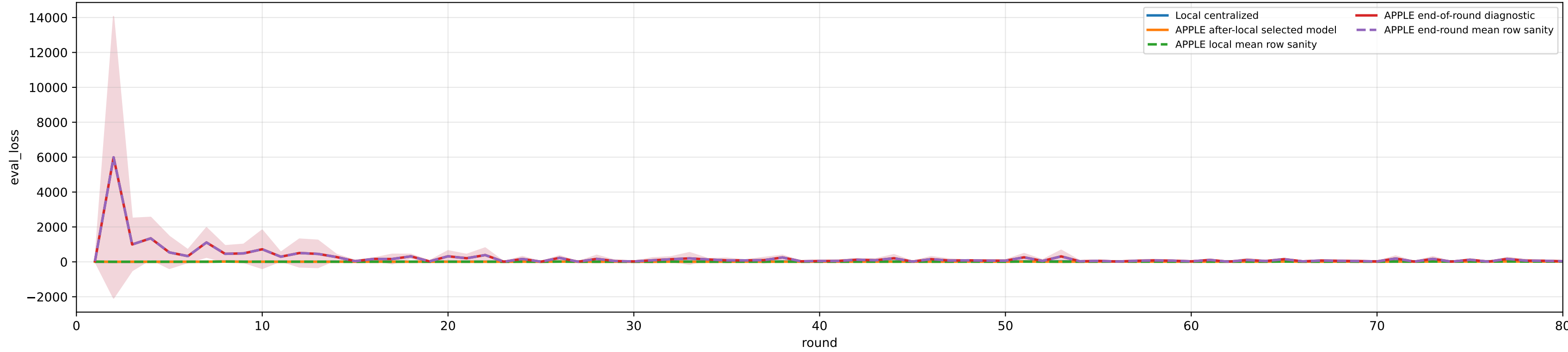
Validation loss: selected APPLE vs end-of-round mismatch (rounds=80)
