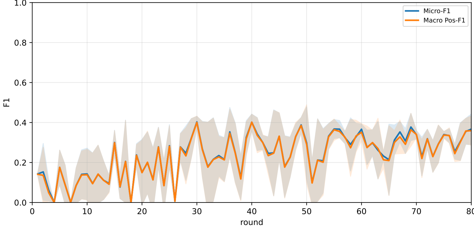
Pooled APPLE micro / macro F1 (end-of-round diagnostic only)
