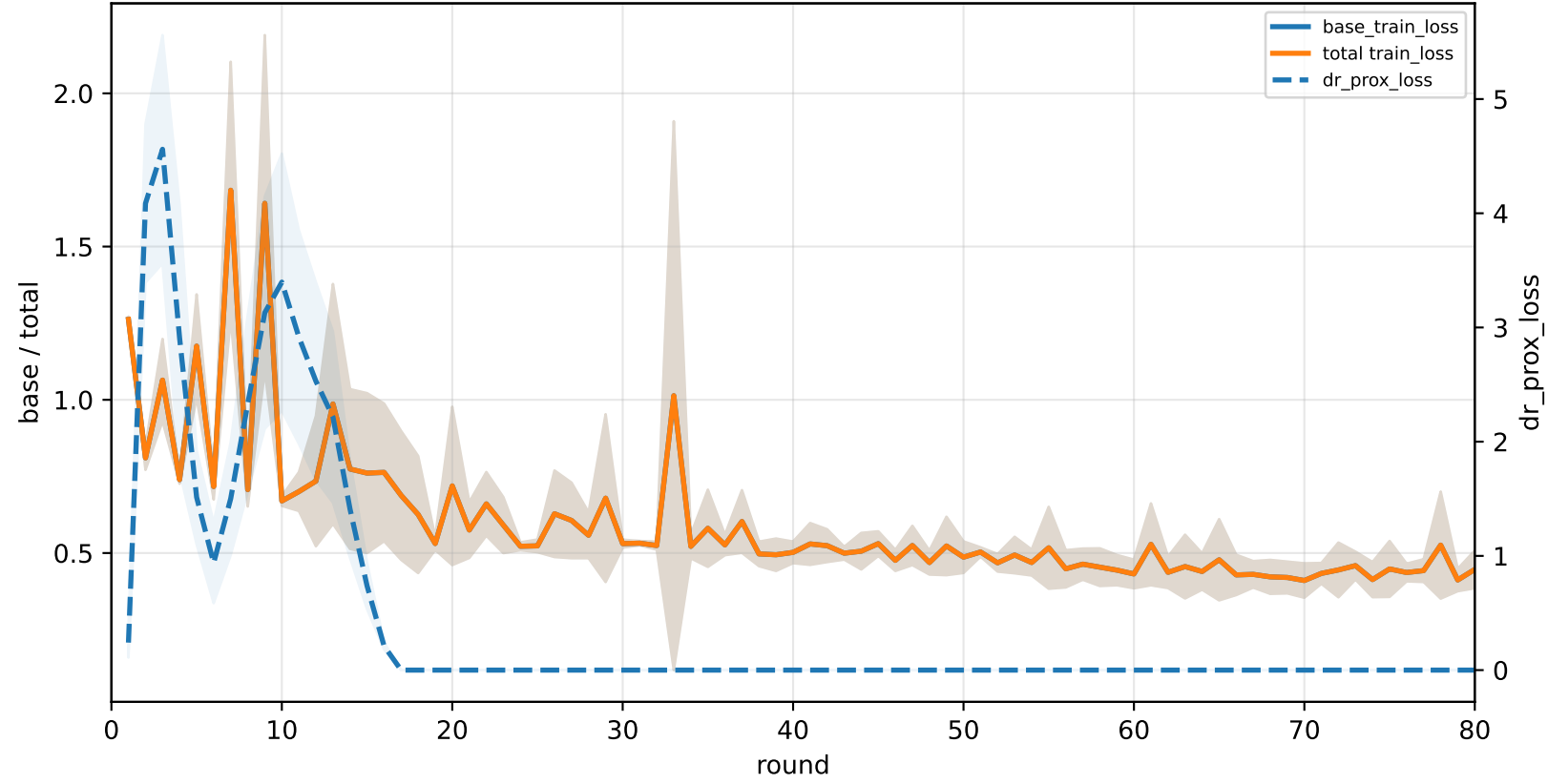
C6-specialist | graph_id=3000004
