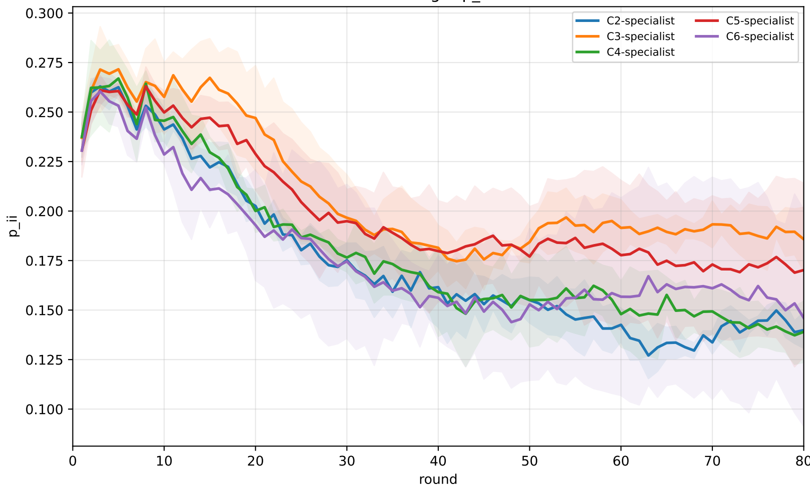
APPLE DR self-weight p_{ii} over rounds
