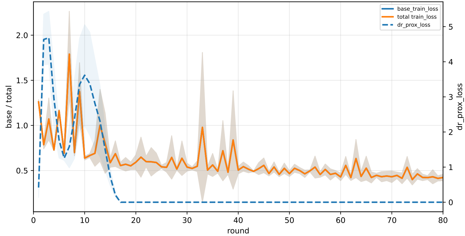
C2-specialist | graph_id=3000000
