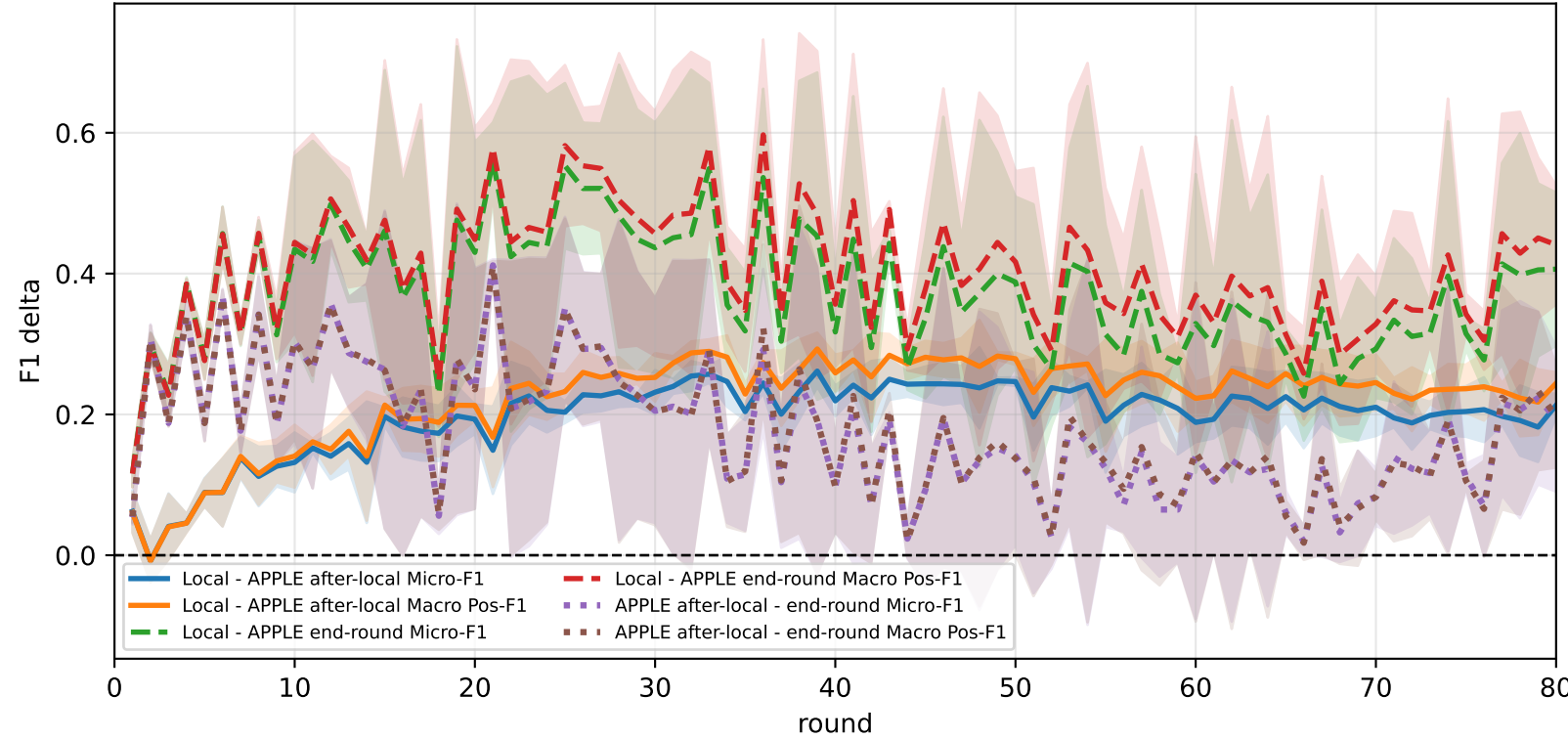
Delta diagnostics: Local gap and APPLE mismatch gap
