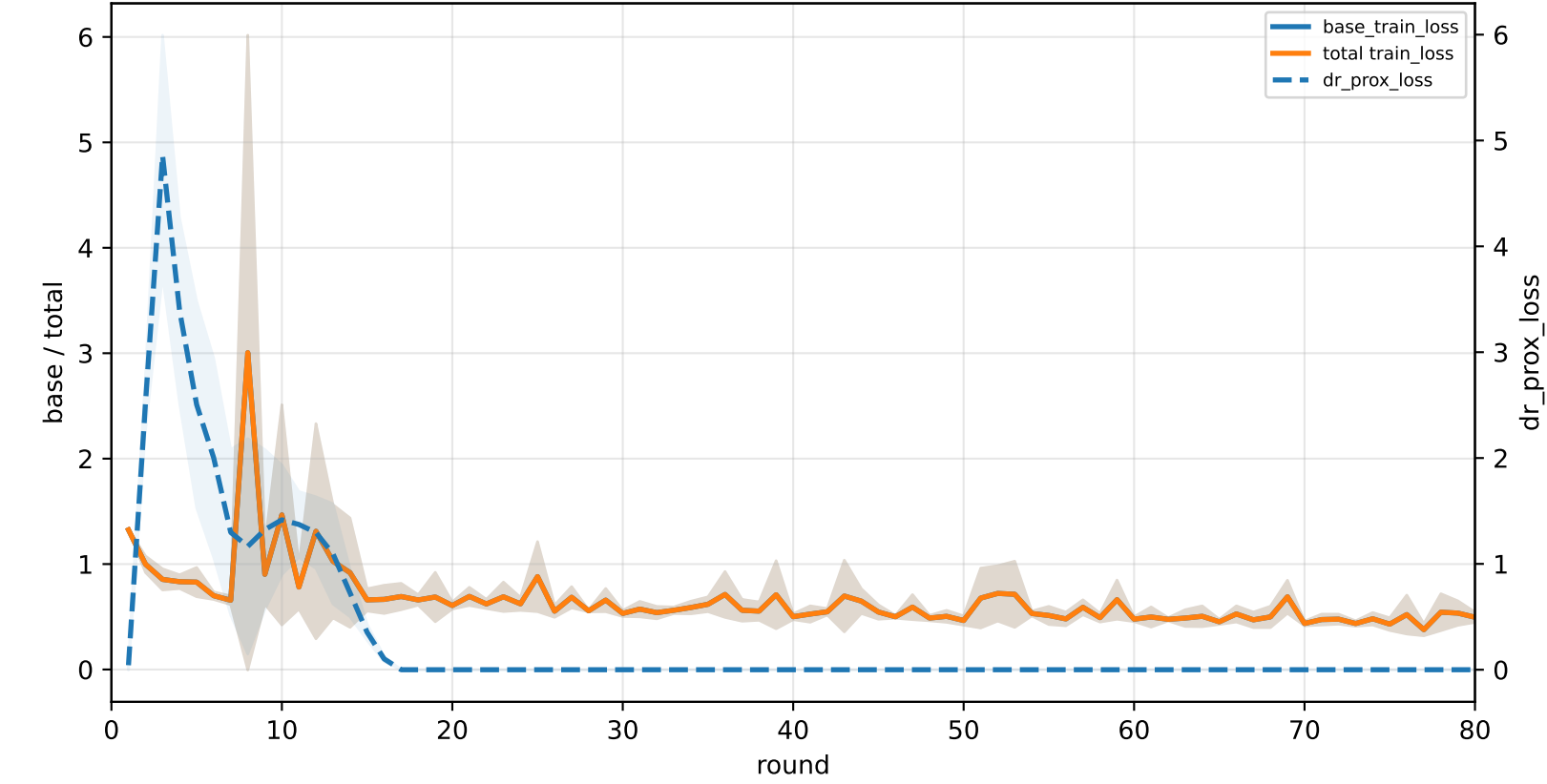
C6-specialist | graph_id=3000014
