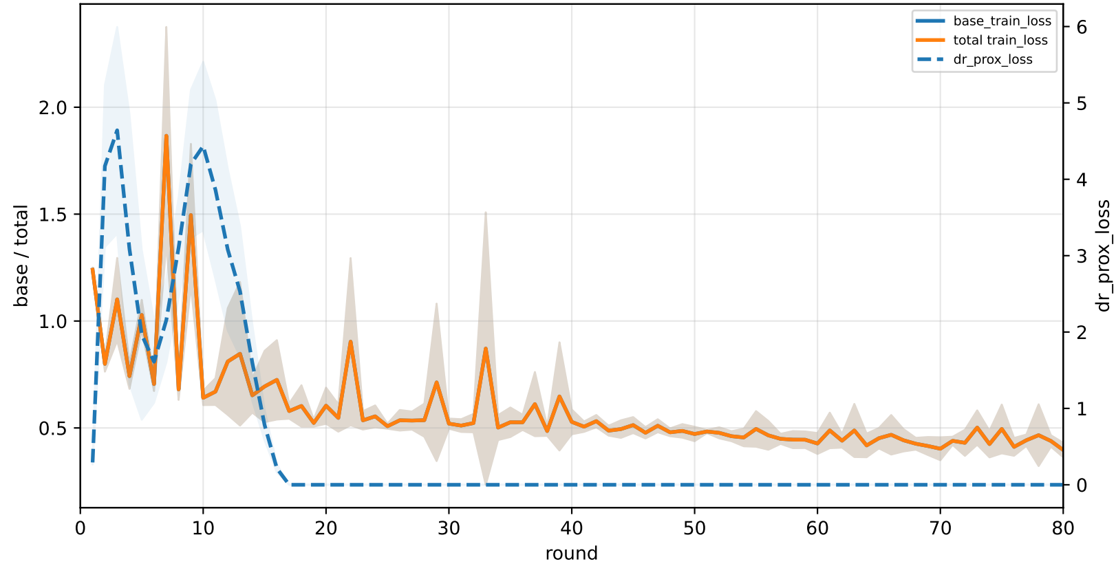
C4-specialist | graph_id=3000002
