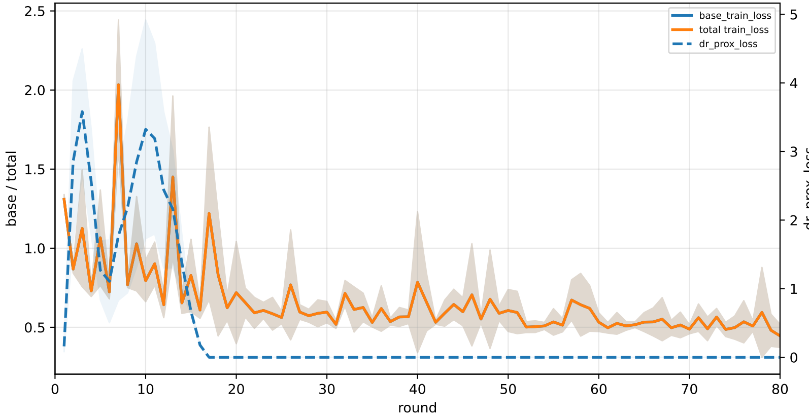
C3-specialist | graph_id=3000006
