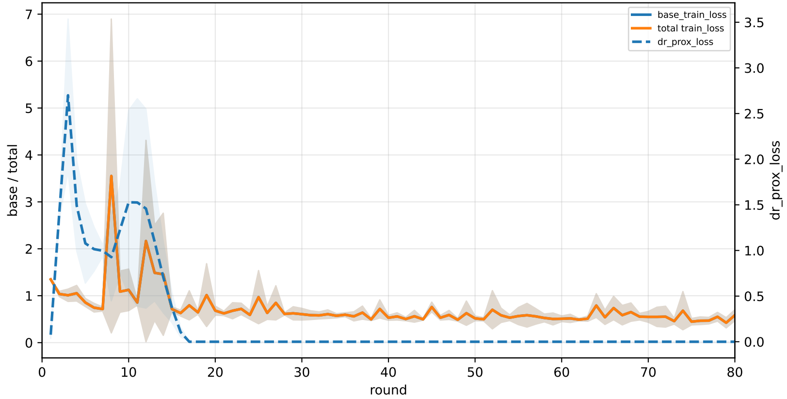
C5-specialist | graph_id=3000013
