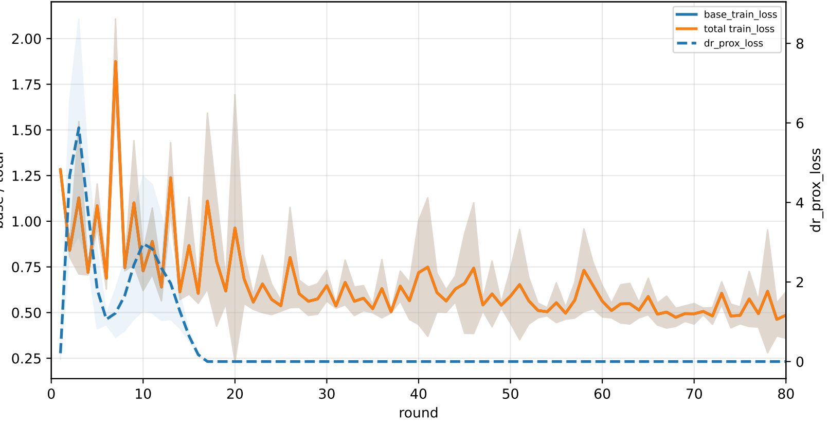
C6-specialist | graph_id=3000009
