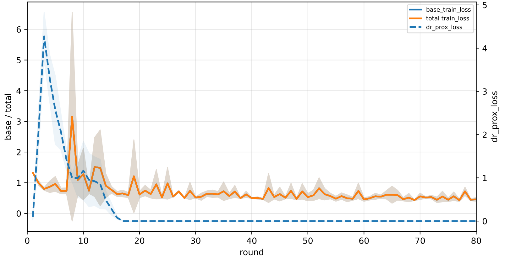
C3-specialist | graph_id=3000011
