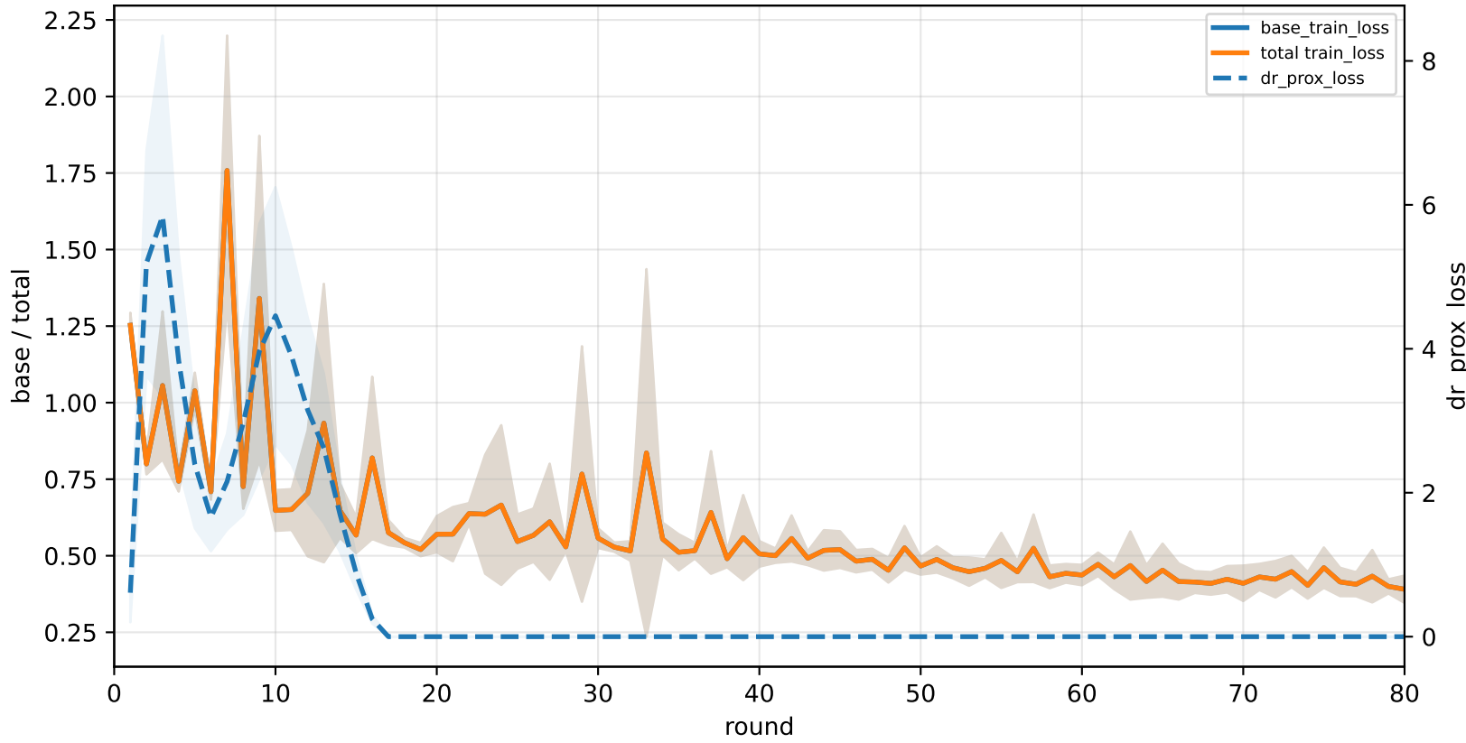
C3-specialist | graph_id=3000001
