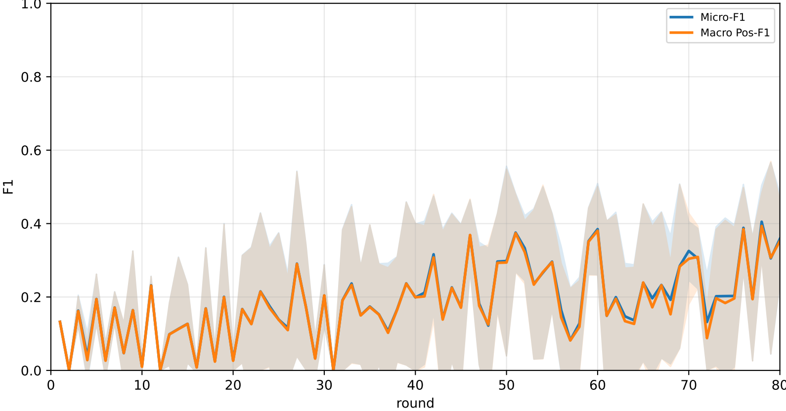
Pooled APPLE micro / macro F1 (end-of-round diagnostic only)
