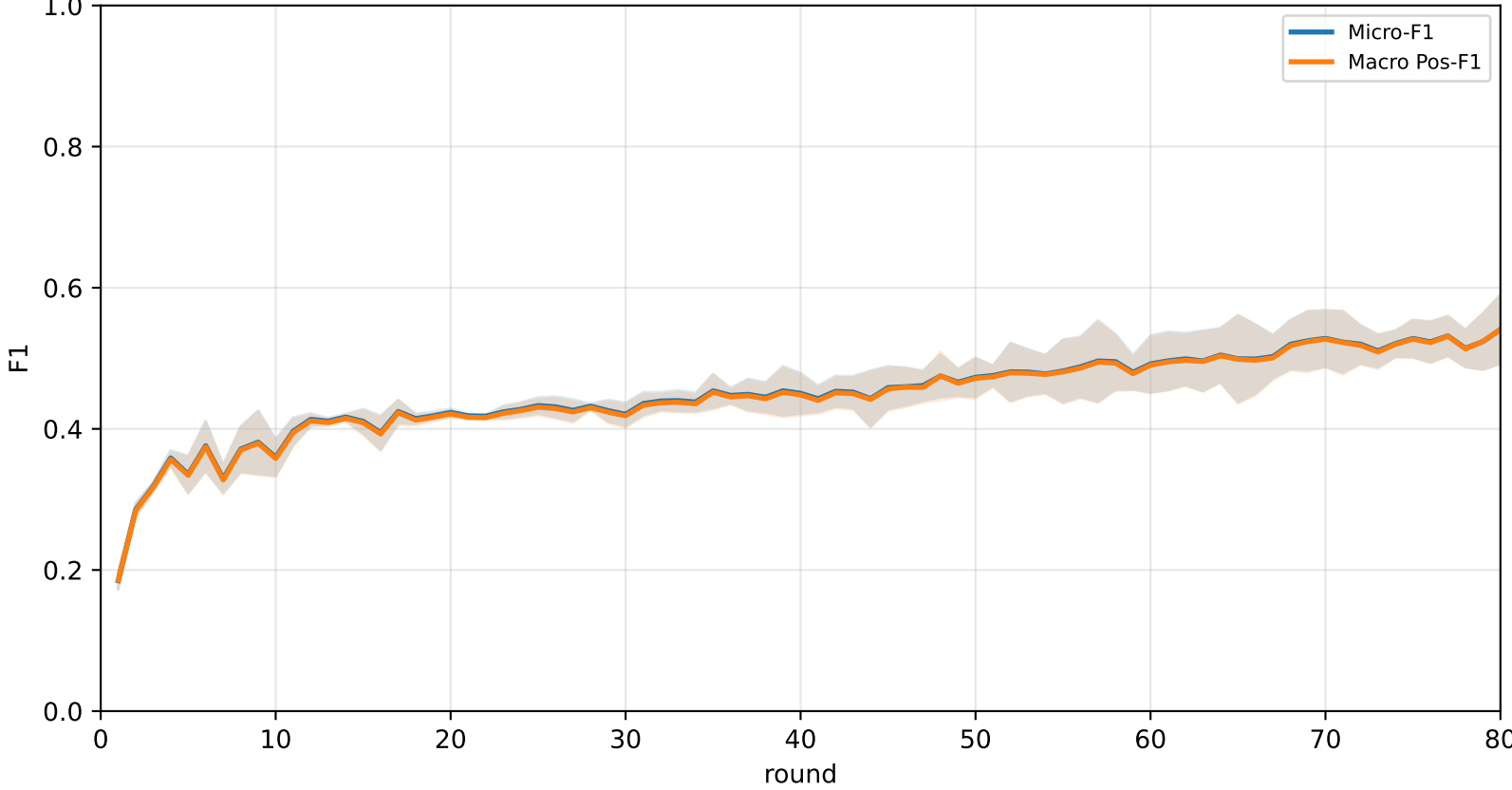
Pooled APPLE micro / macro F1 (after-local selected model)
