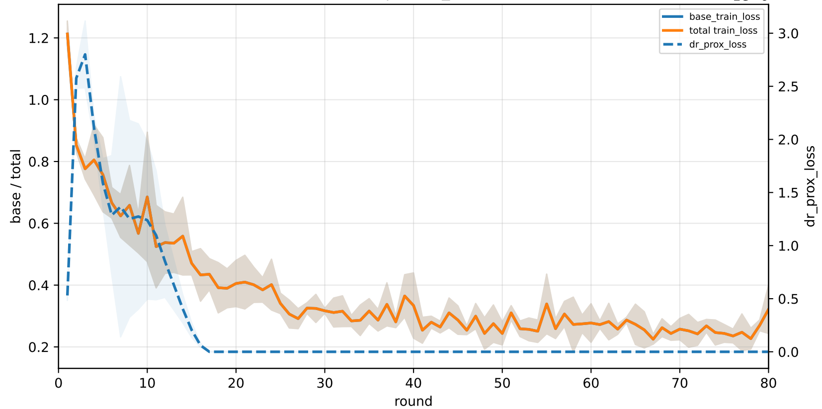
C5-specialist | graph_id=3000008
