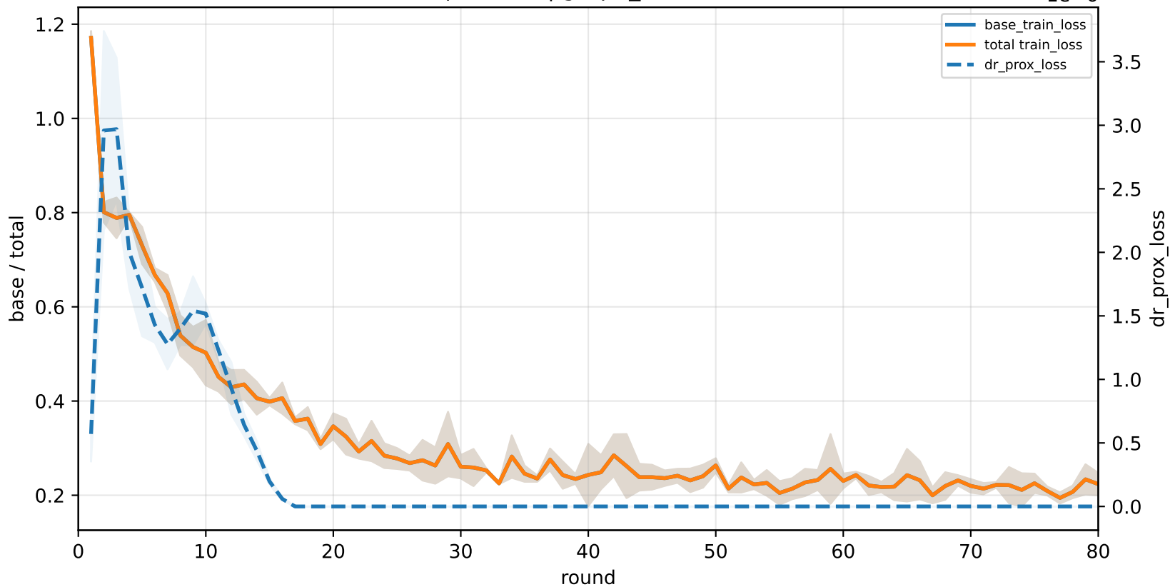
C3-specialist | graph_id=3000001
