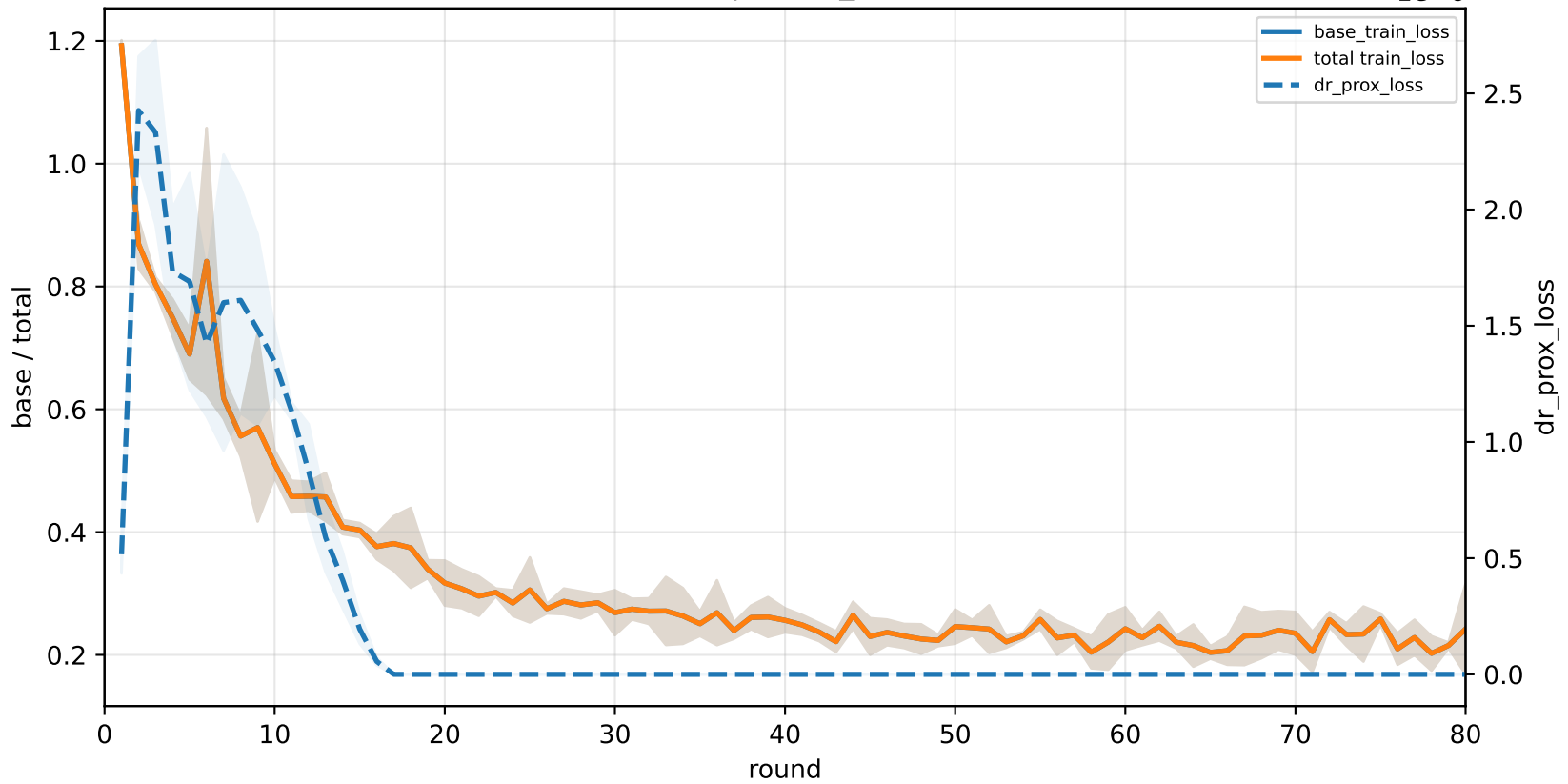
C5-specialist | graph_id=3000003
