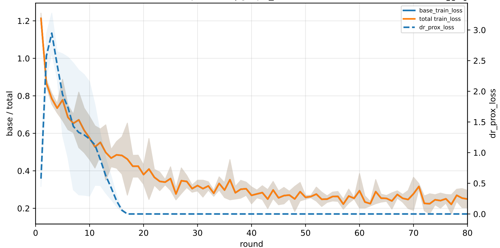
C3-specialist | graph_id=3000006
