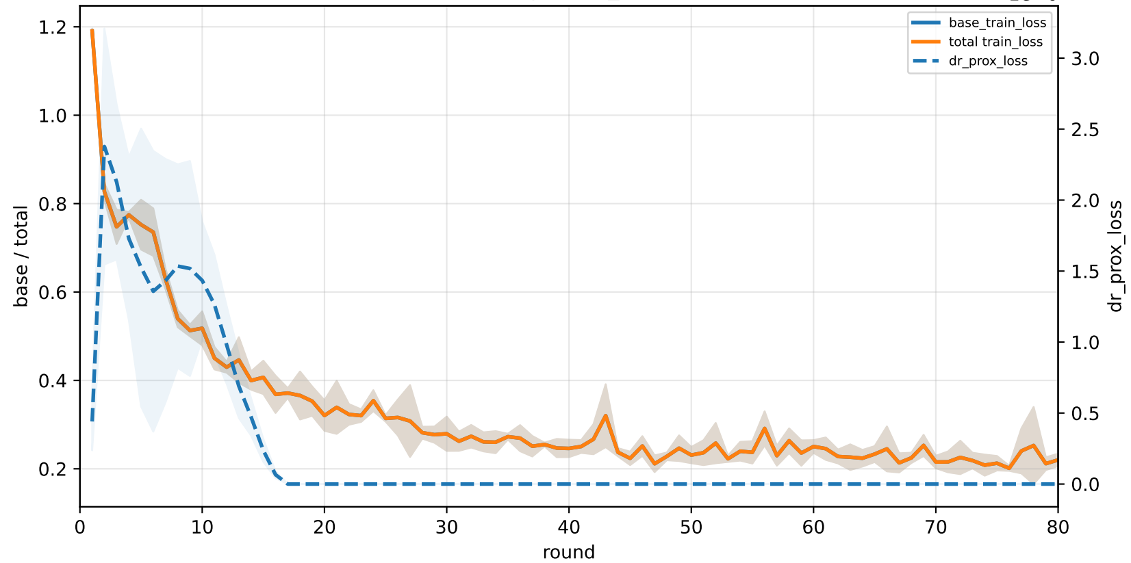
C6-specialist | graph_id=3000004
