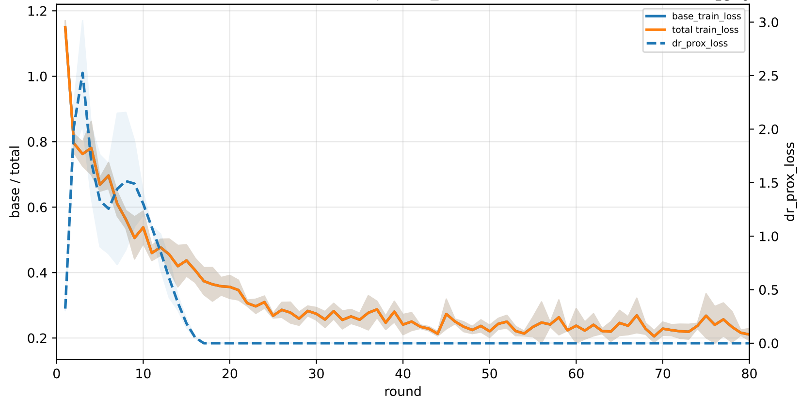
C4-specialist | graph_id=3000002
