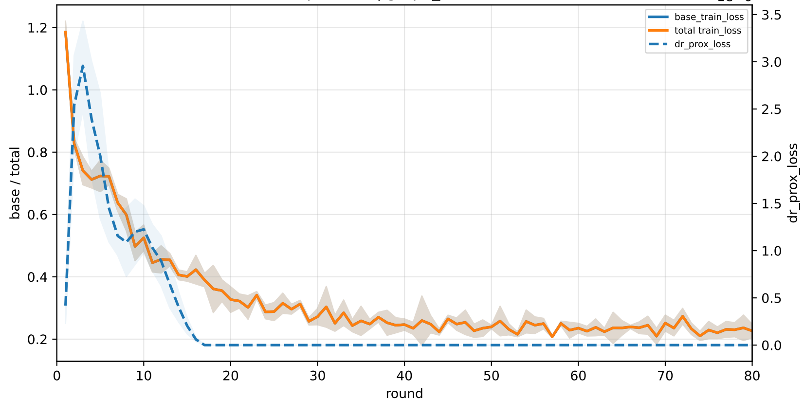
C2-specialist | graph_id=3000000
