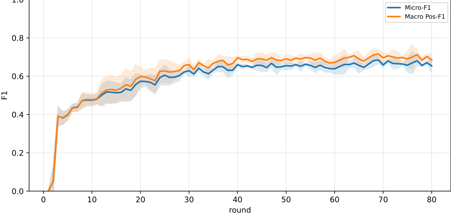
Pooled GCFL+ micro / macro F1 (post-aggregation)
