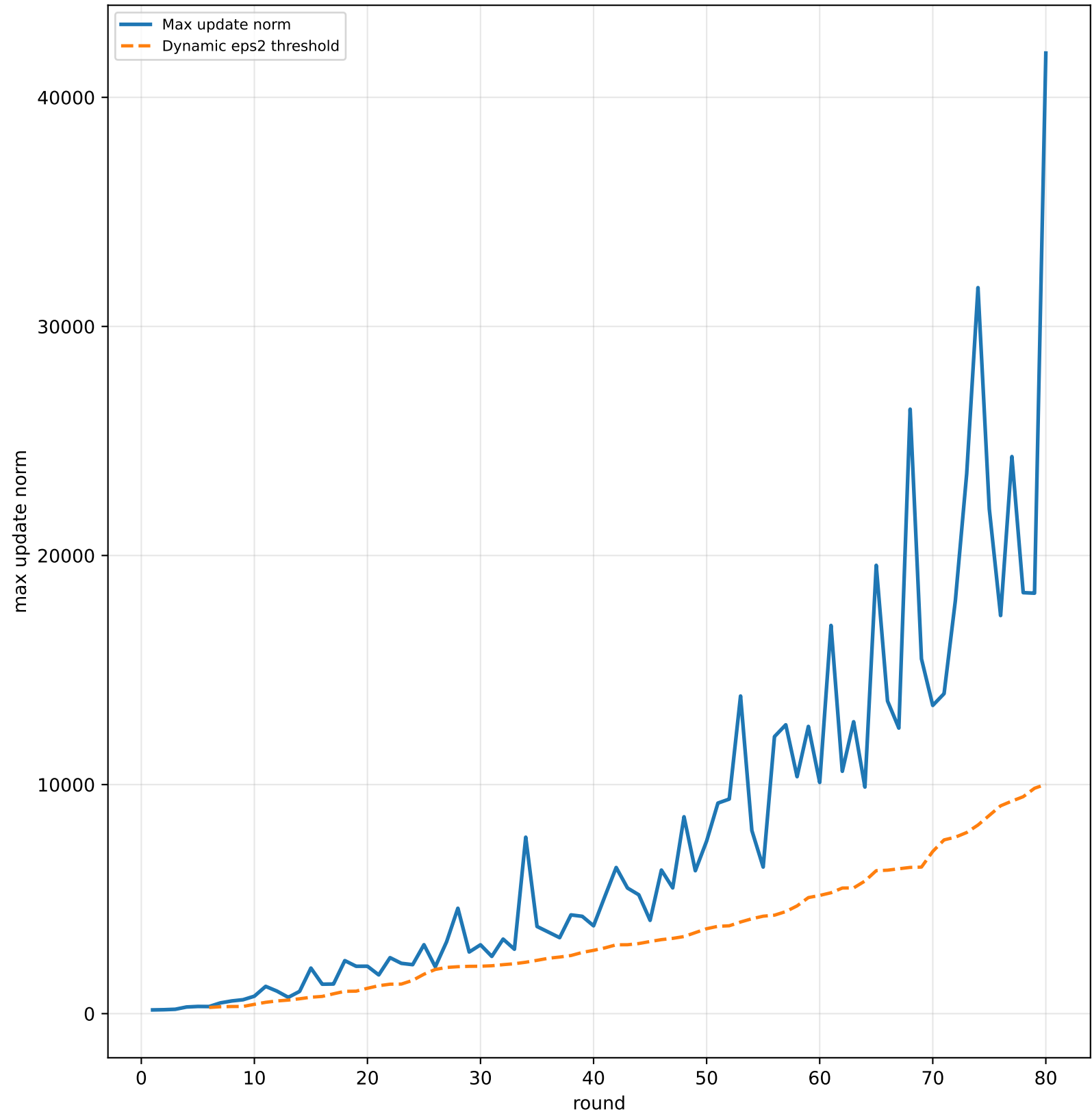
Cluster 0 | Max update norm
