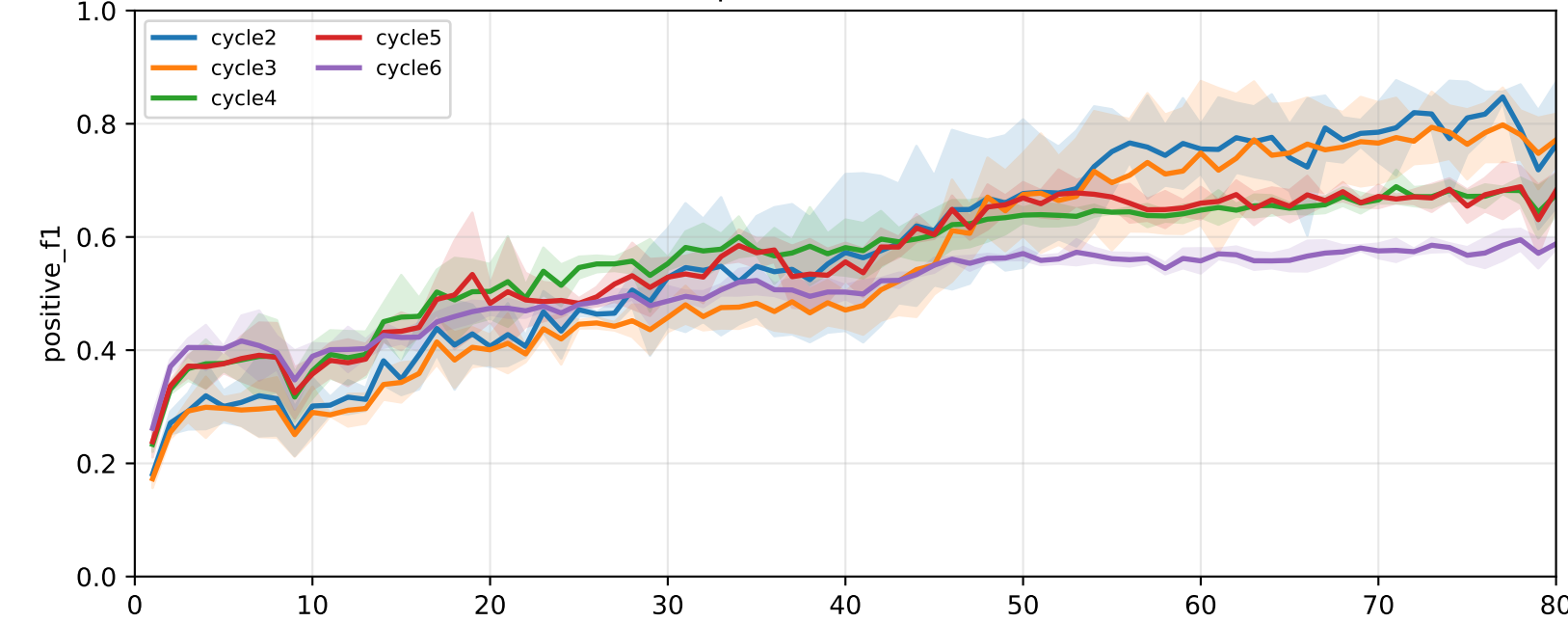
Pooled APPLE-Backbone-TaskHead positive F1 (after-local selected model, rounds=80)
