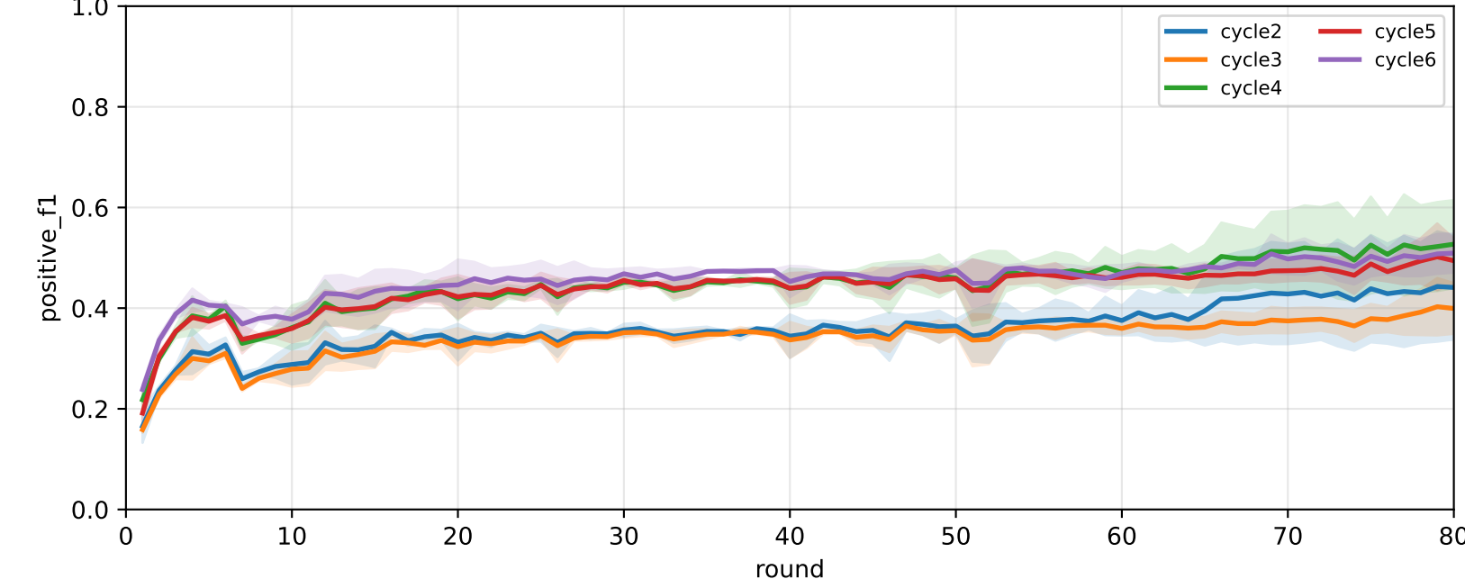
Pooled APPLE positive F1 (after-local selected model, rounds=80)
