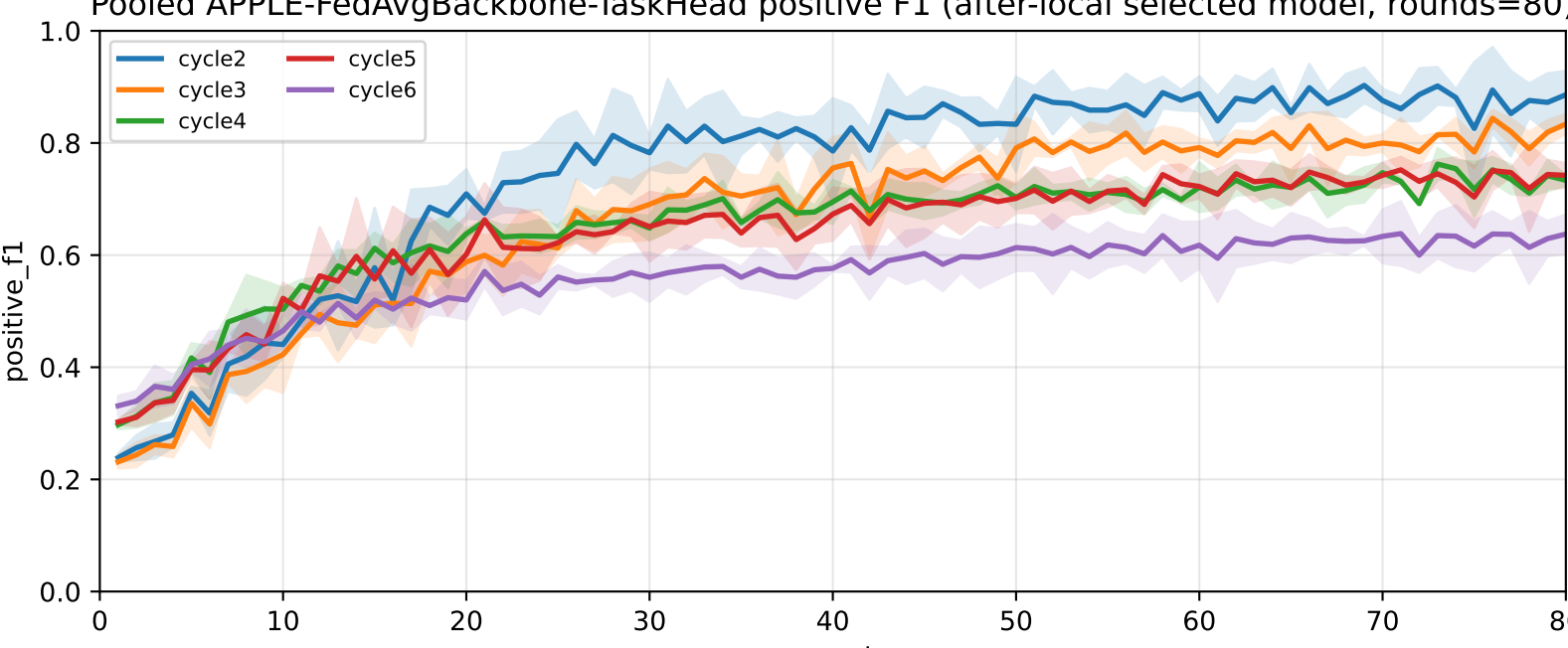
Pooled APPLE-FedAvgBackbone-TaskHead positive F1 (after-local selected model, rounds=80)
