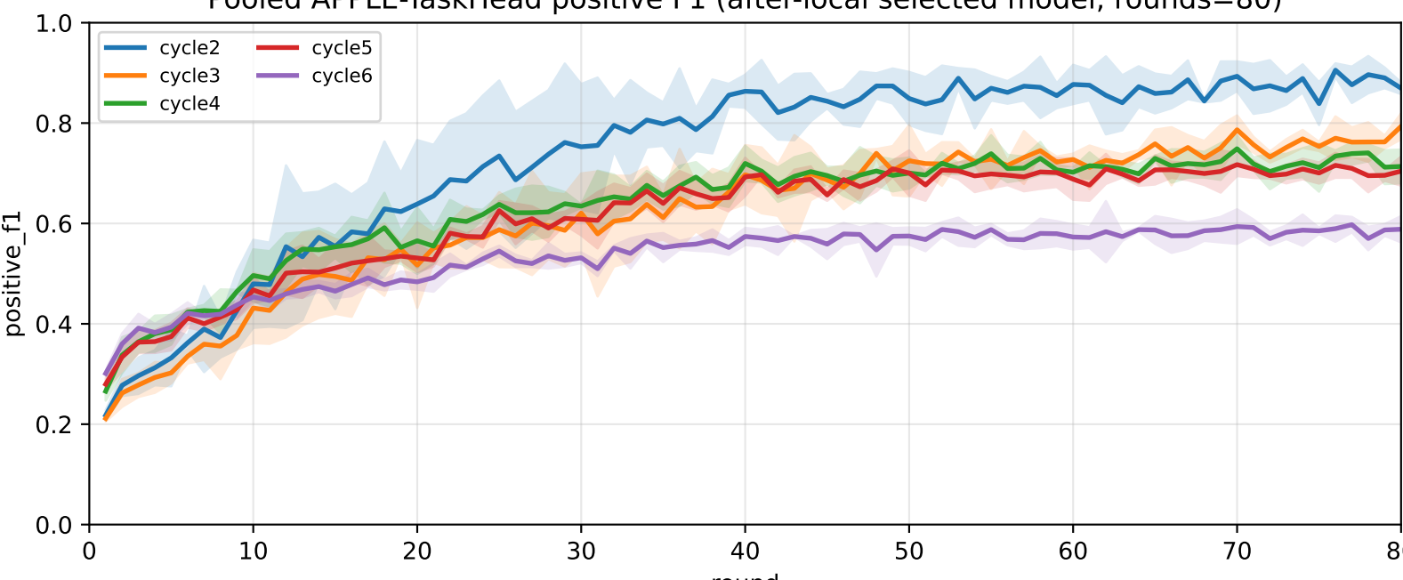
Pooled APPLE-TaskHead positive F1 (after-local selected model, rounds=80)
