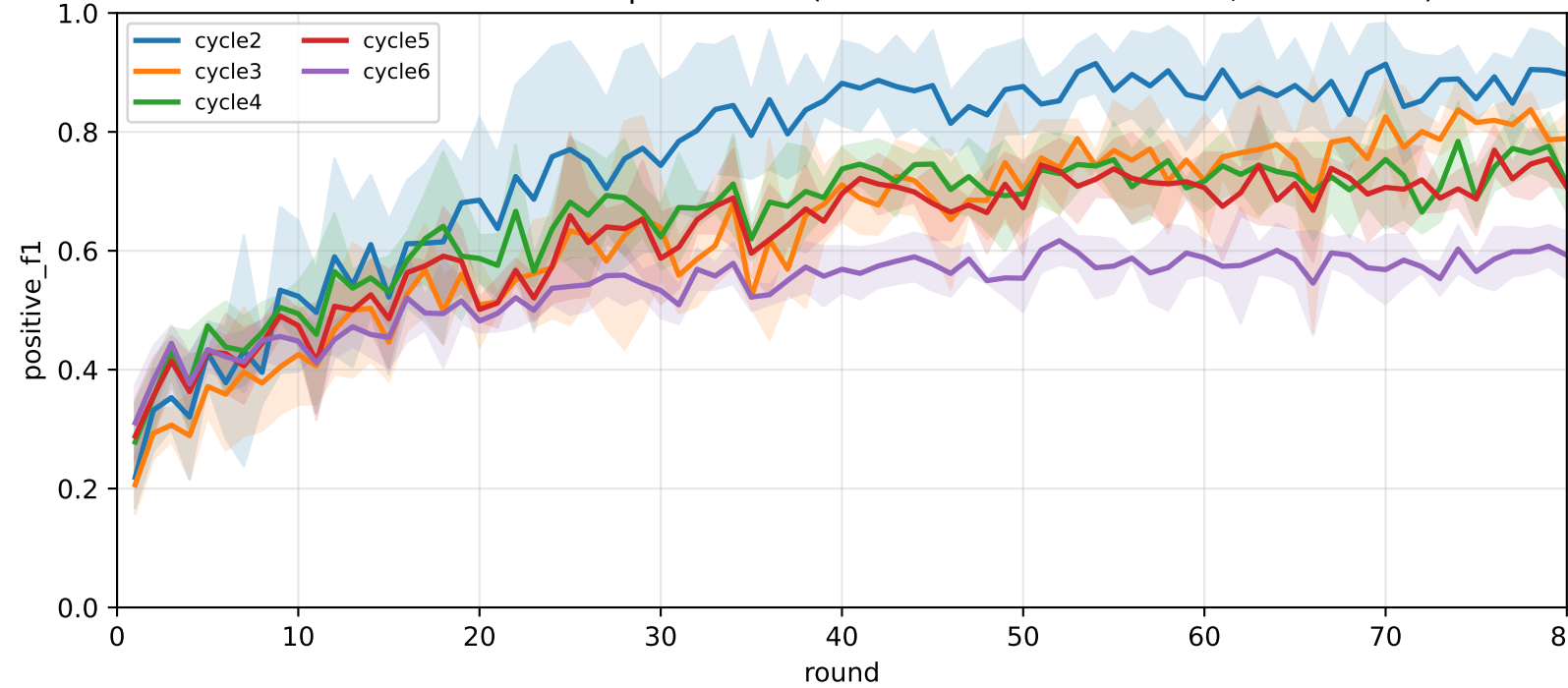
Pooled APPLE-TaskHead positive F1 (after-local selected model, rounds=80)
