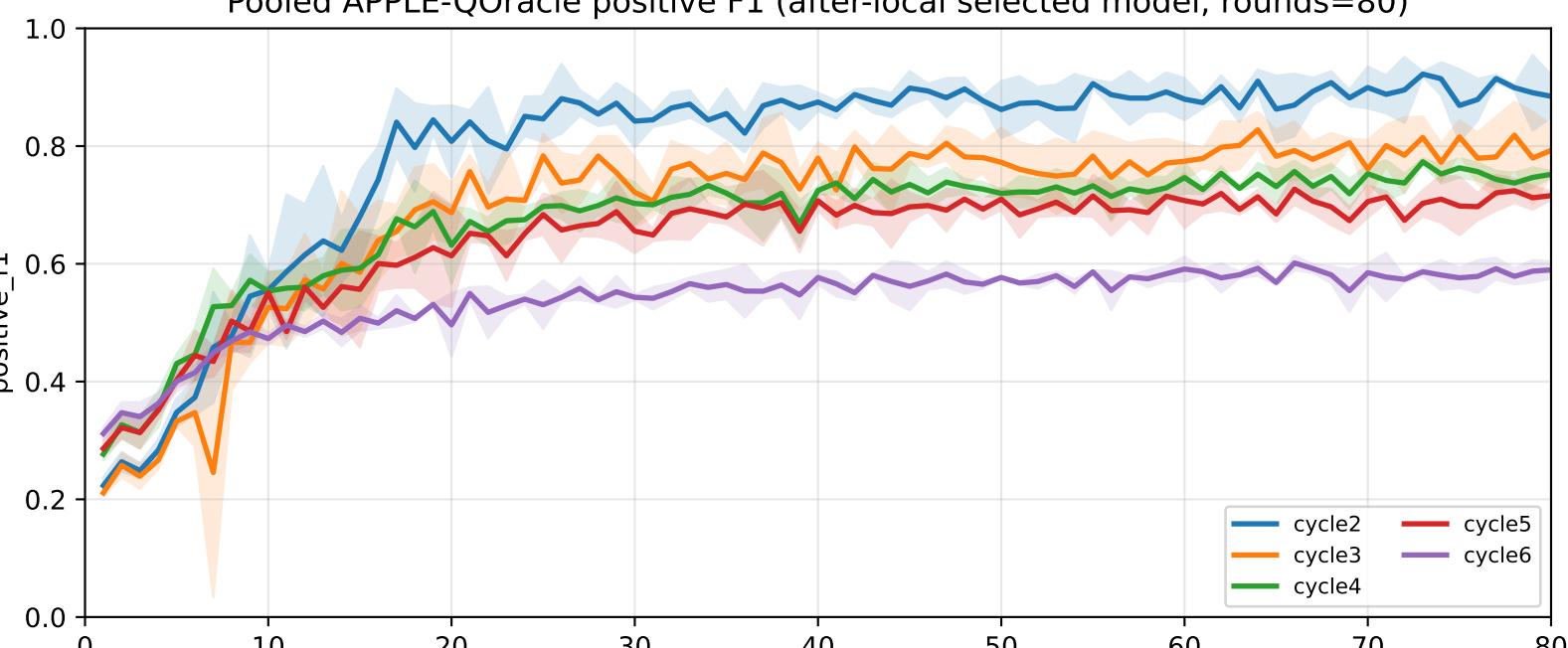
Pooled APPLE-QOracle positive F1 (after-local selected model, rounds=80)
