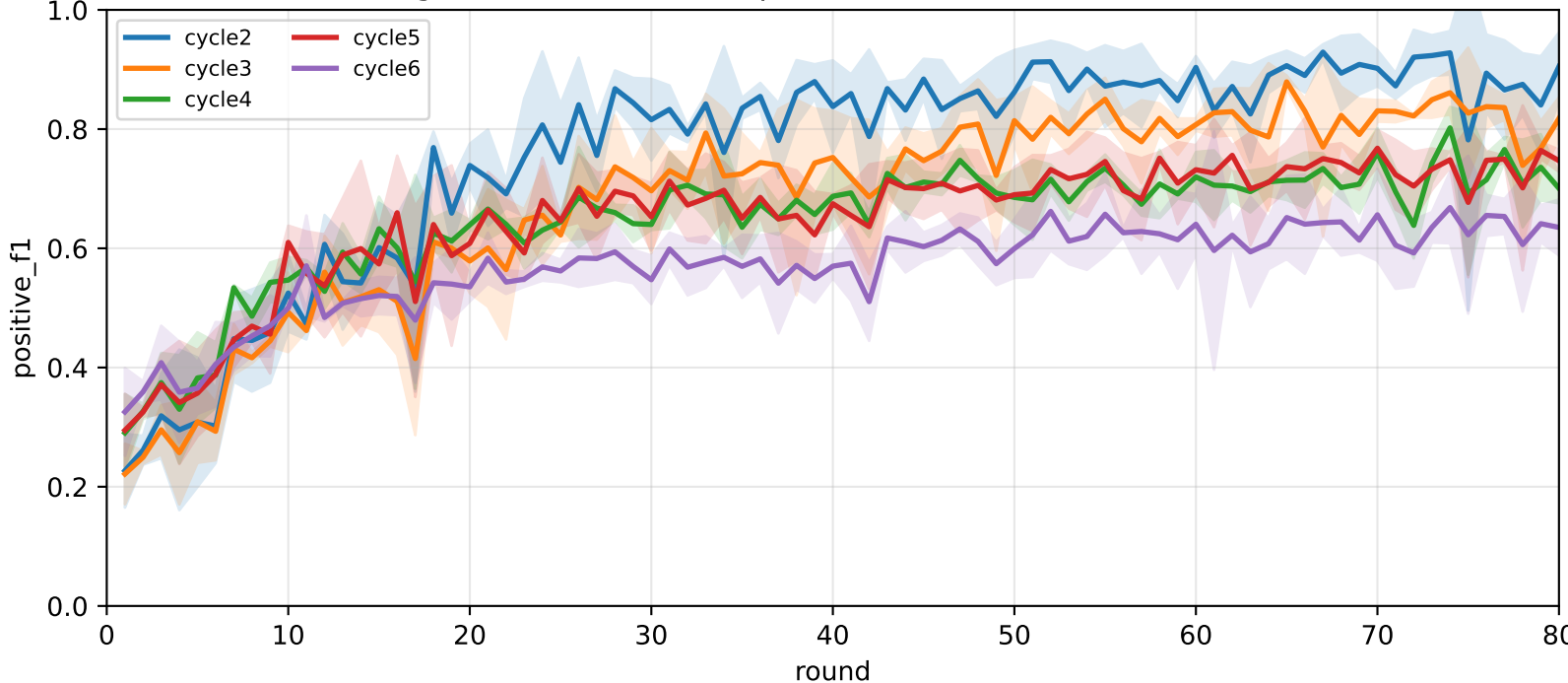
Pooled APPLE-FedAvgBackbone-TaskHead positive F1 (after-local selected model, rounds=80)
