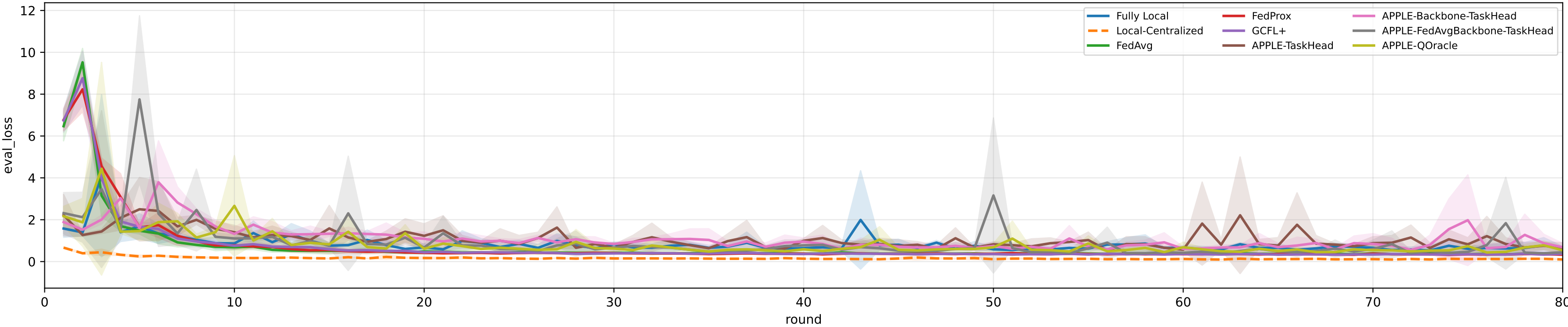
Validation loss comparison (APPLE family: rounds=80, dr_lr=0.001, mu=0.001, Lfrac=0.2)
