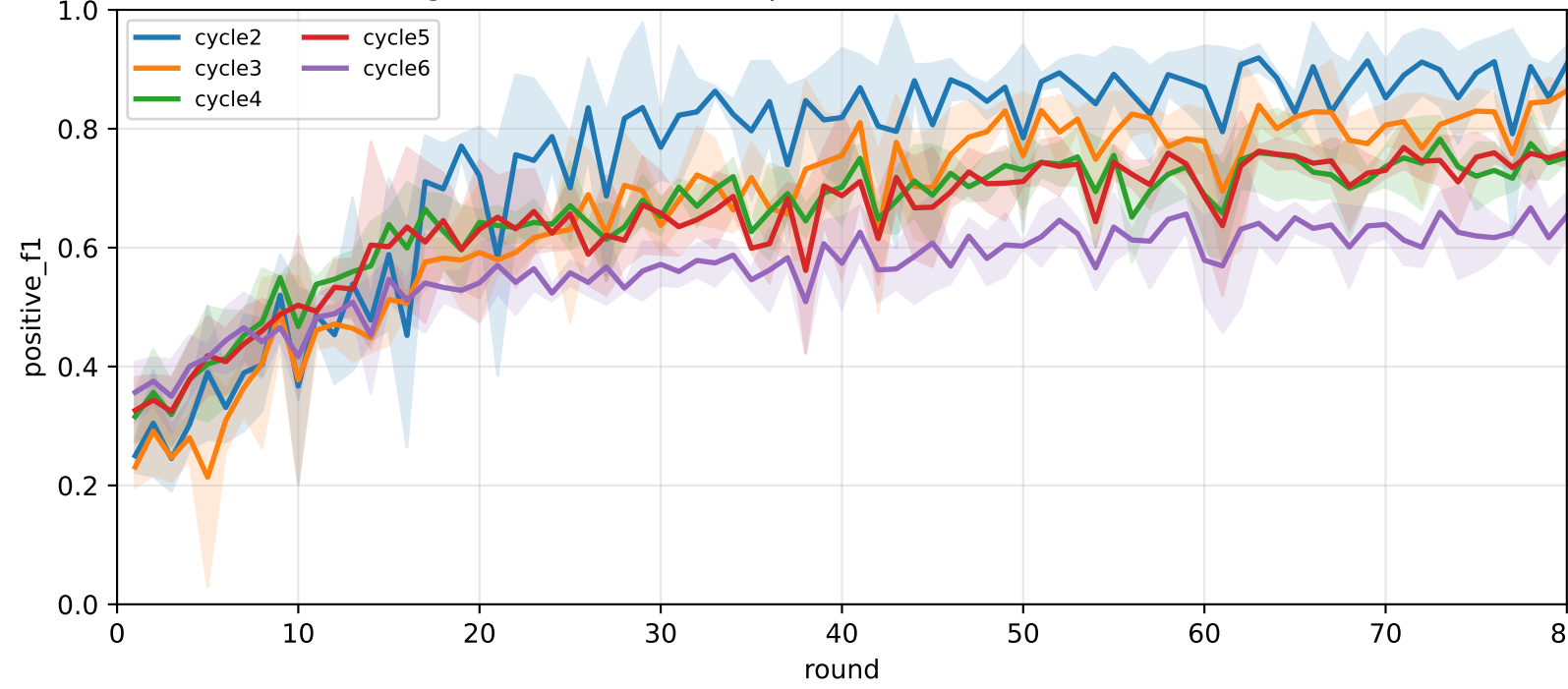
Pooled APPLE-FedAvgBackbone-TaskHead positive F1 (after-local selected model, rounds=80)
