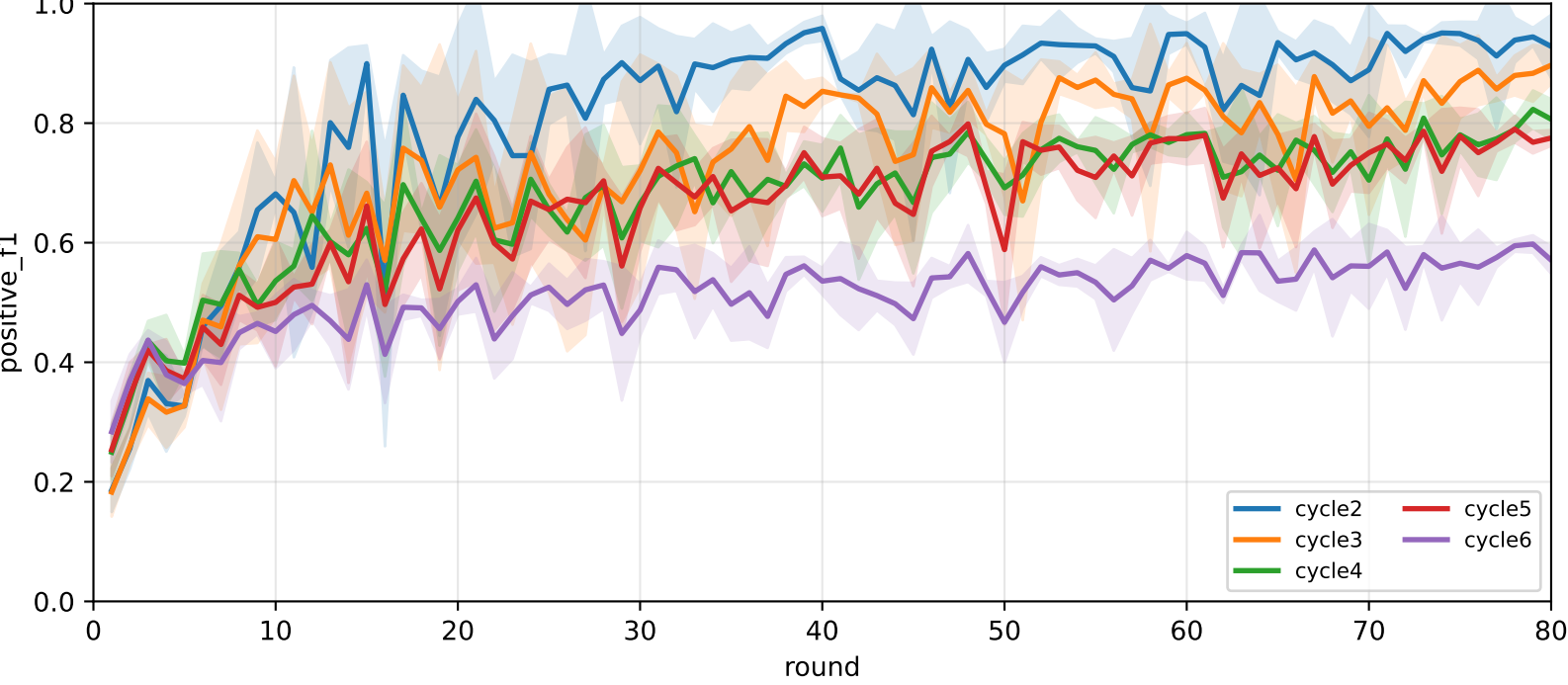
Pooled Fully Local positive F1
