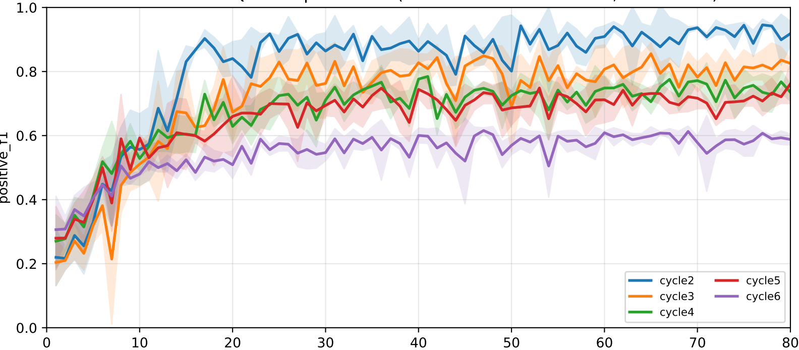
Pooled APPLE-QOracle positive F1 (after-local selected model, rounds=80)
