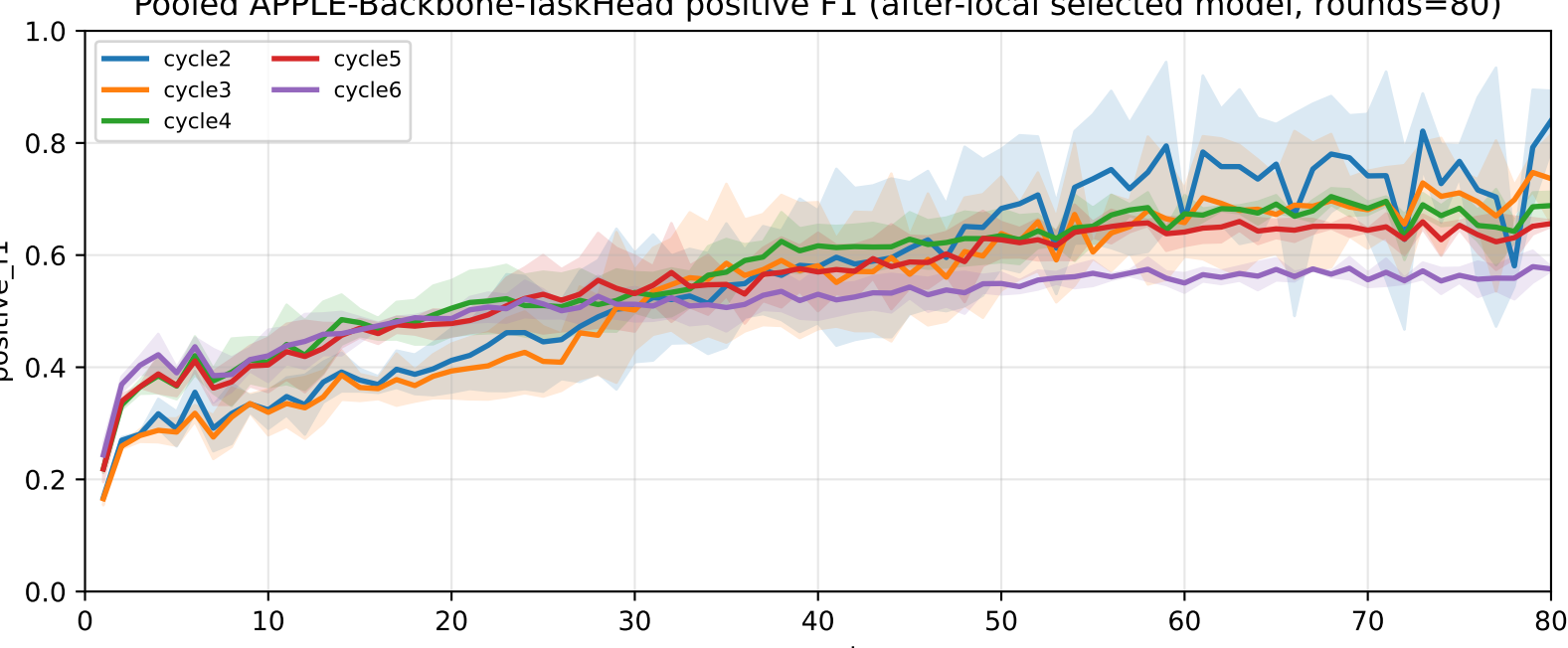
Pooled APPLE-Backbone-TaskHead positive F1 (after-local selected model, rounds=80)
