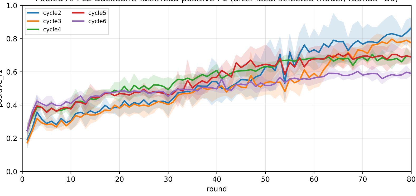
Pooled APPLE-Backbone-TaskHead positive F1 (after-local selected model, rounds=80)
