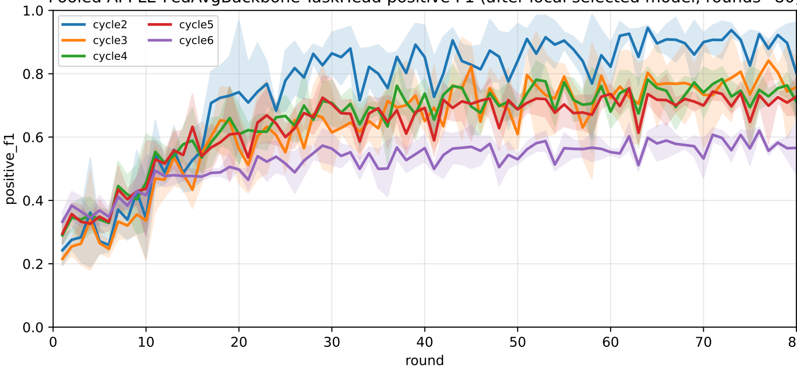
Pooled APPLE-FedAvgBackbone-TaskHead positive F1 (after-local selected model, rounds=80)
