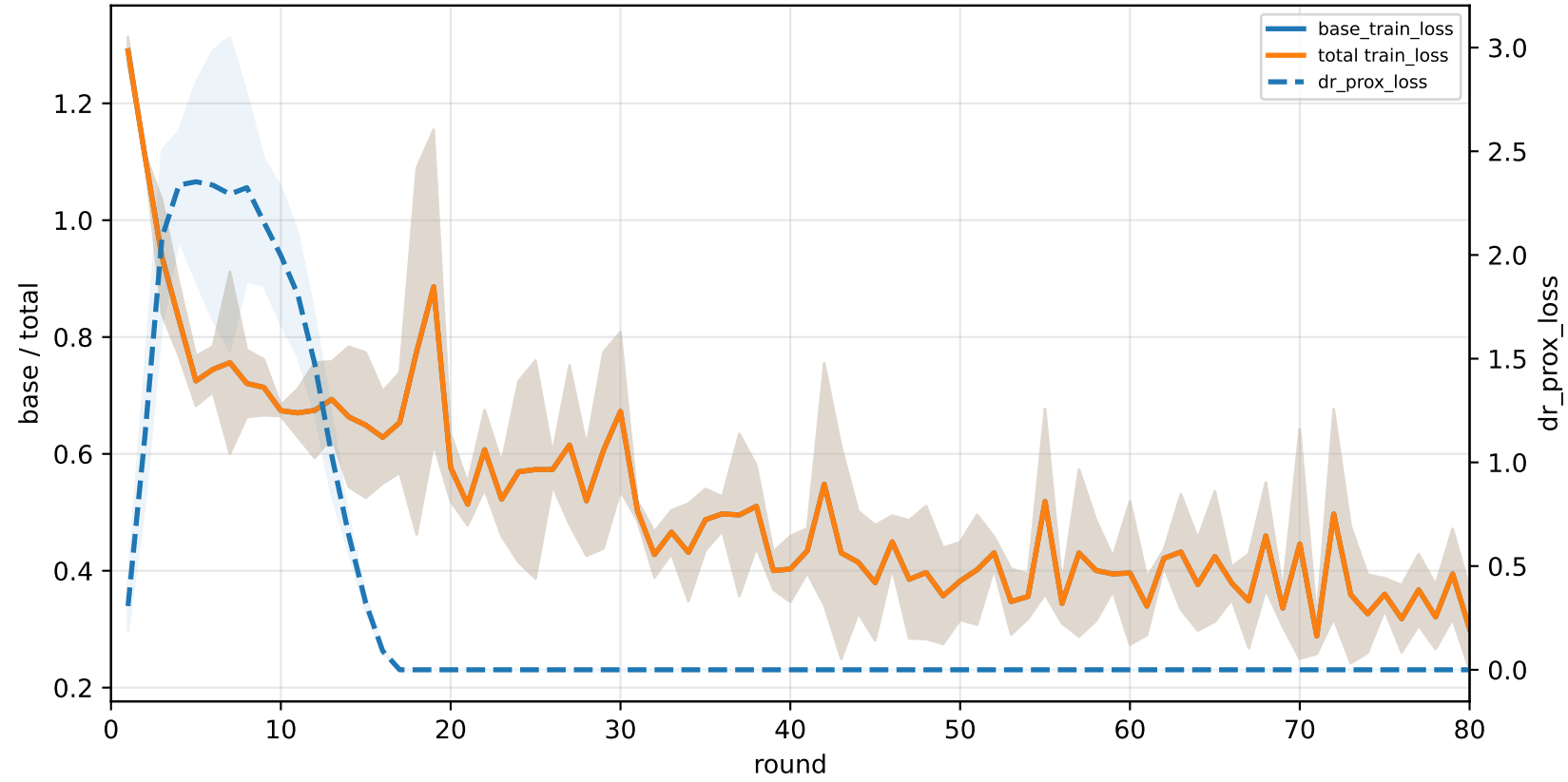
q_task_cycle4 | graph_id=3000012
