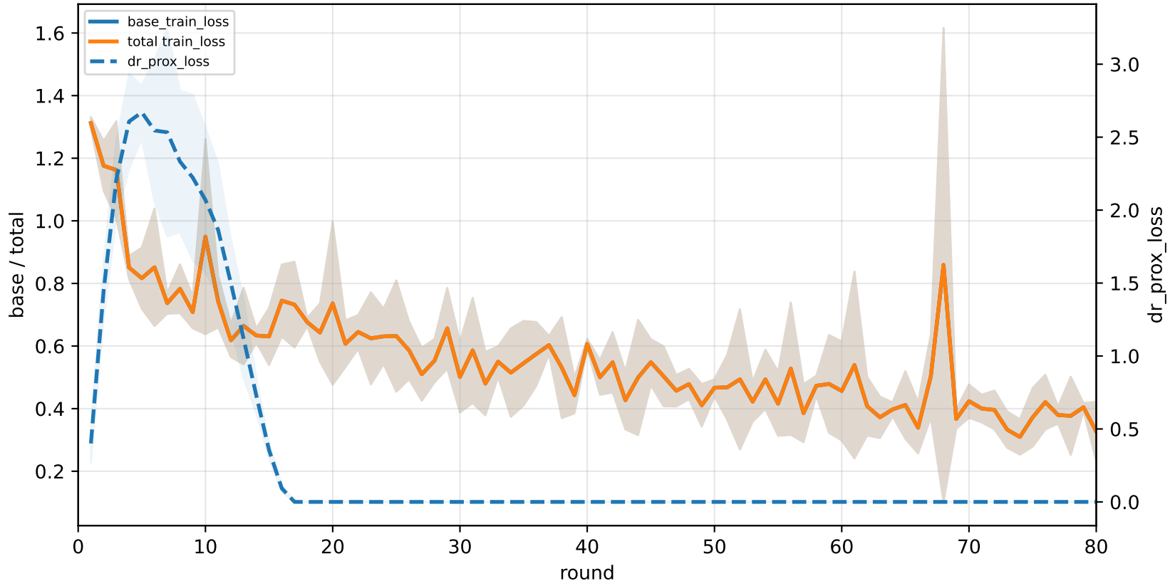
q_task_cycle5 | graph_id=3000013
