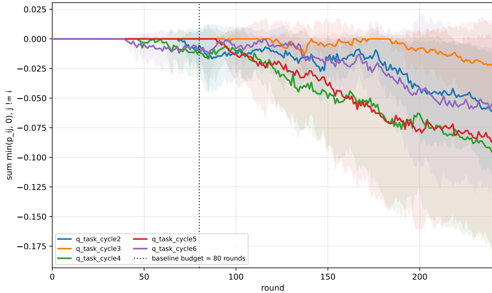
APPLE off-diagonal negative mass over rounds
