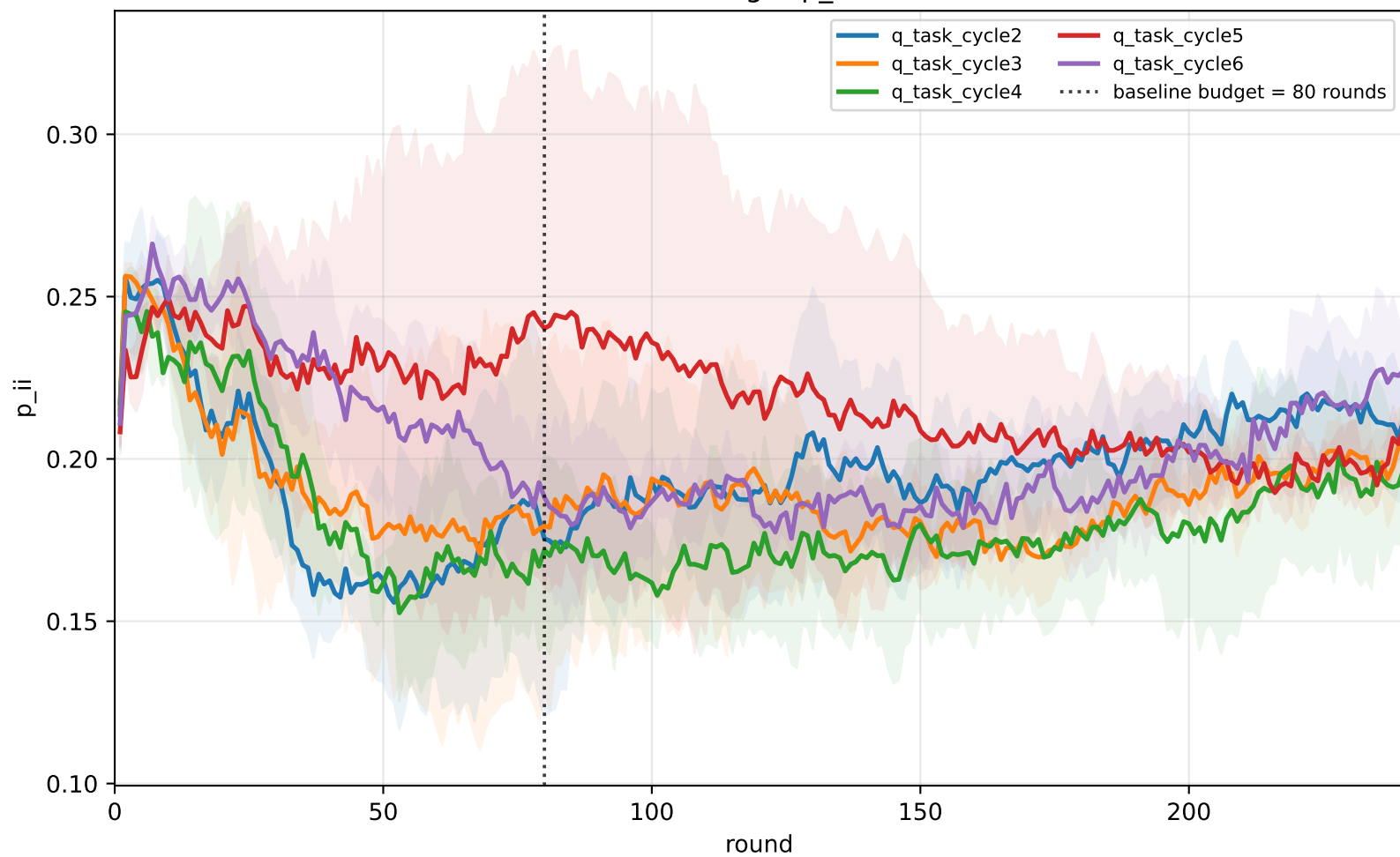
APPLE DR self-weight p_{ii} over rounds
