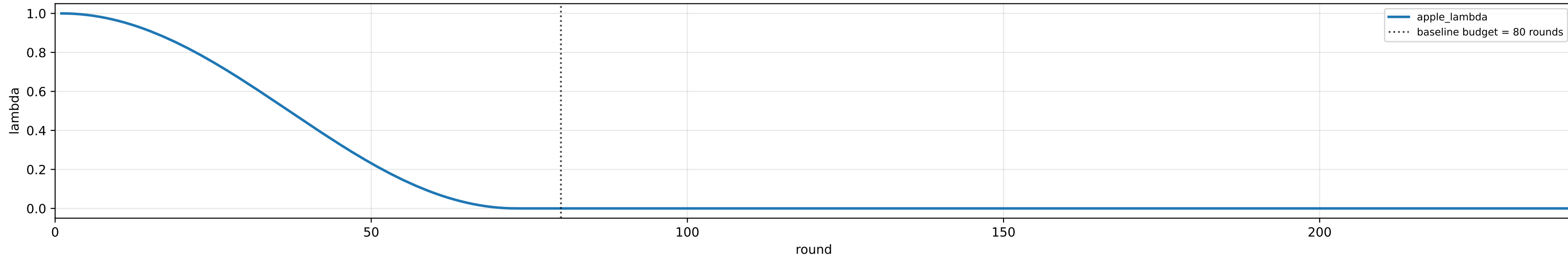
APPLE lambda scheduler | apple_mu=0.01
