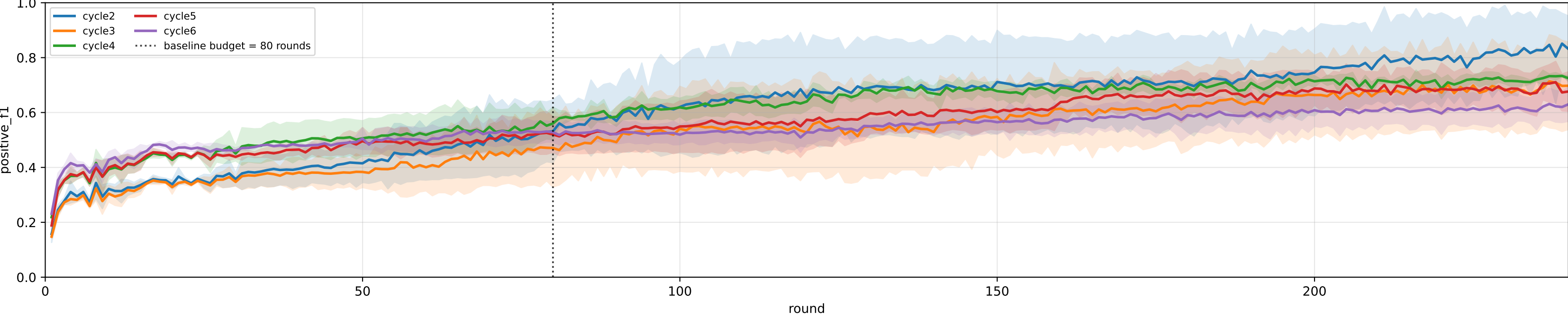
Pooled APPLE positive F1 (after-local selected model, equal 240-round budget)
