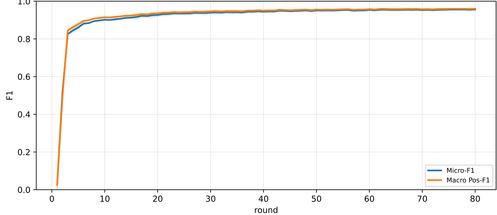
Pooled FedAvg micro / macro F1 (post-aggregation)
