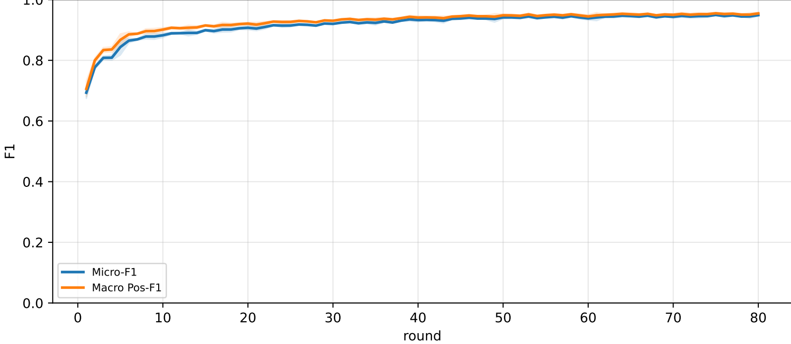
Pooled FedAvg micro / macro F1 (pre-aggregation)
