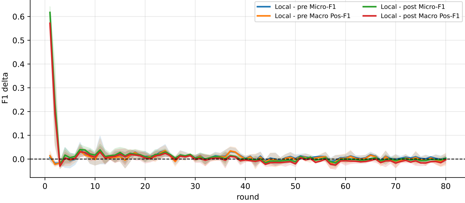
Delta vs FedAvg (local minus pre / post)
