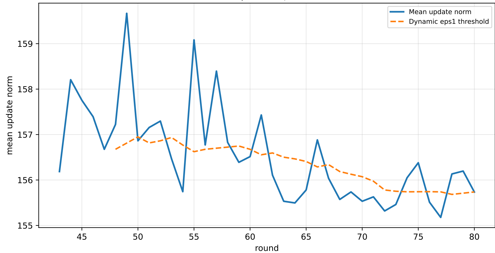
Cluster 8 | Mean update norm
