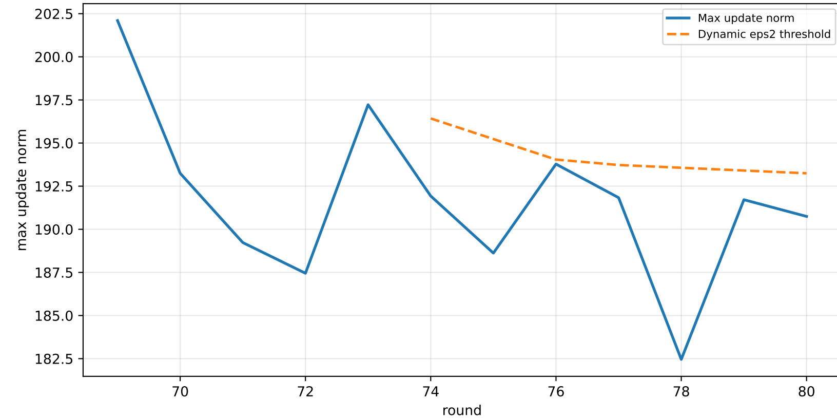
Cluster 8 | Max update norm
