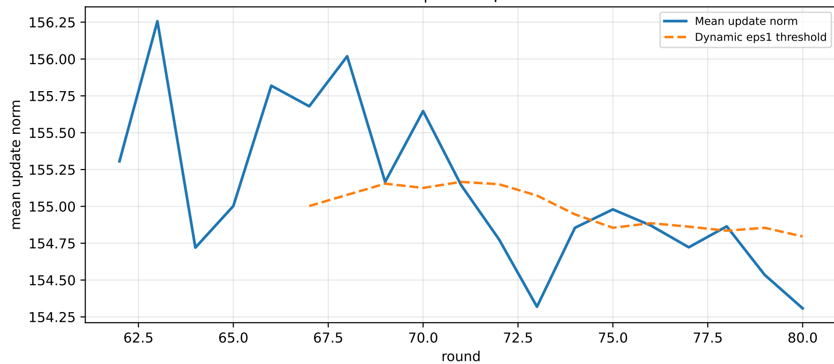
Cluster 14 | Mean update norm
