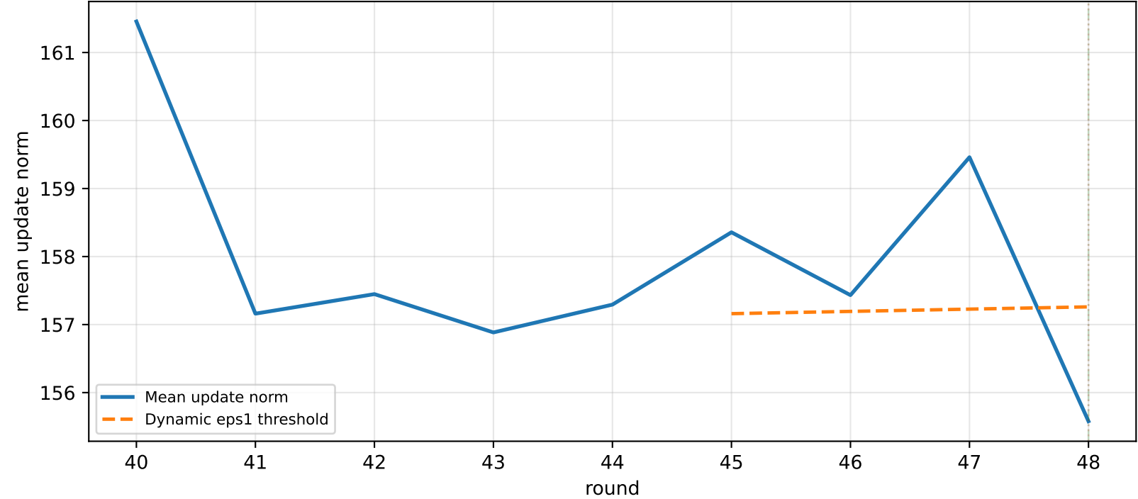
Cluster 8 | Mean update norm
