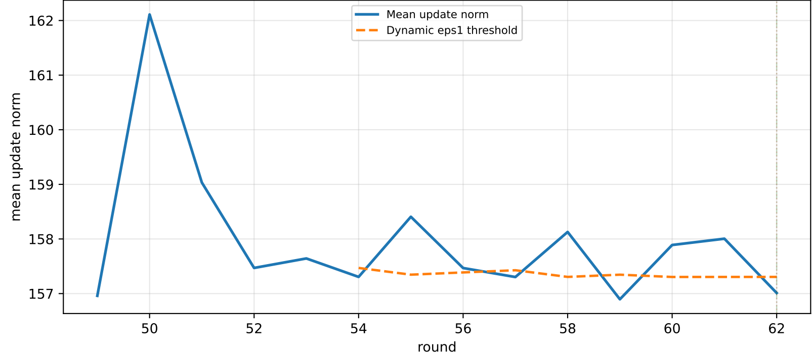
Cluster 10 | Mean update norm
