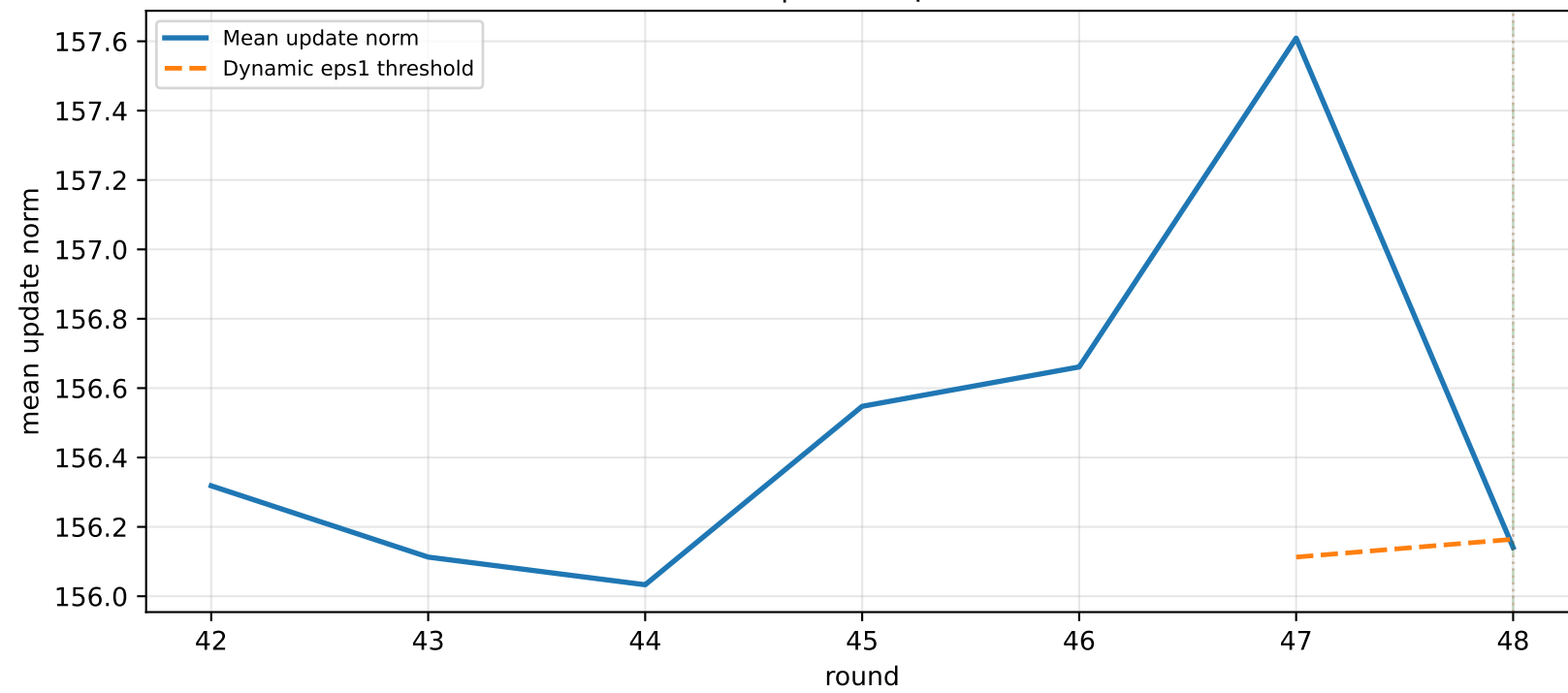
Cluster 8 | Mean update norm
