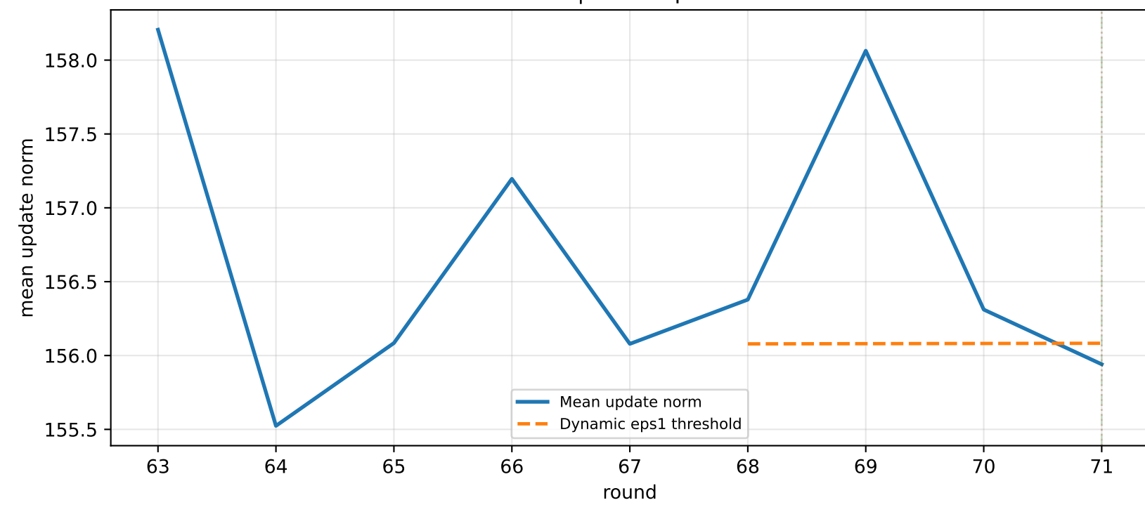
Cluster 12 | Mean update norm
