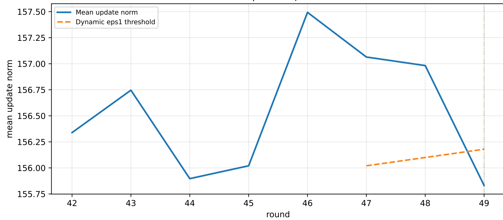
Cluster 8 | Mean update norm
