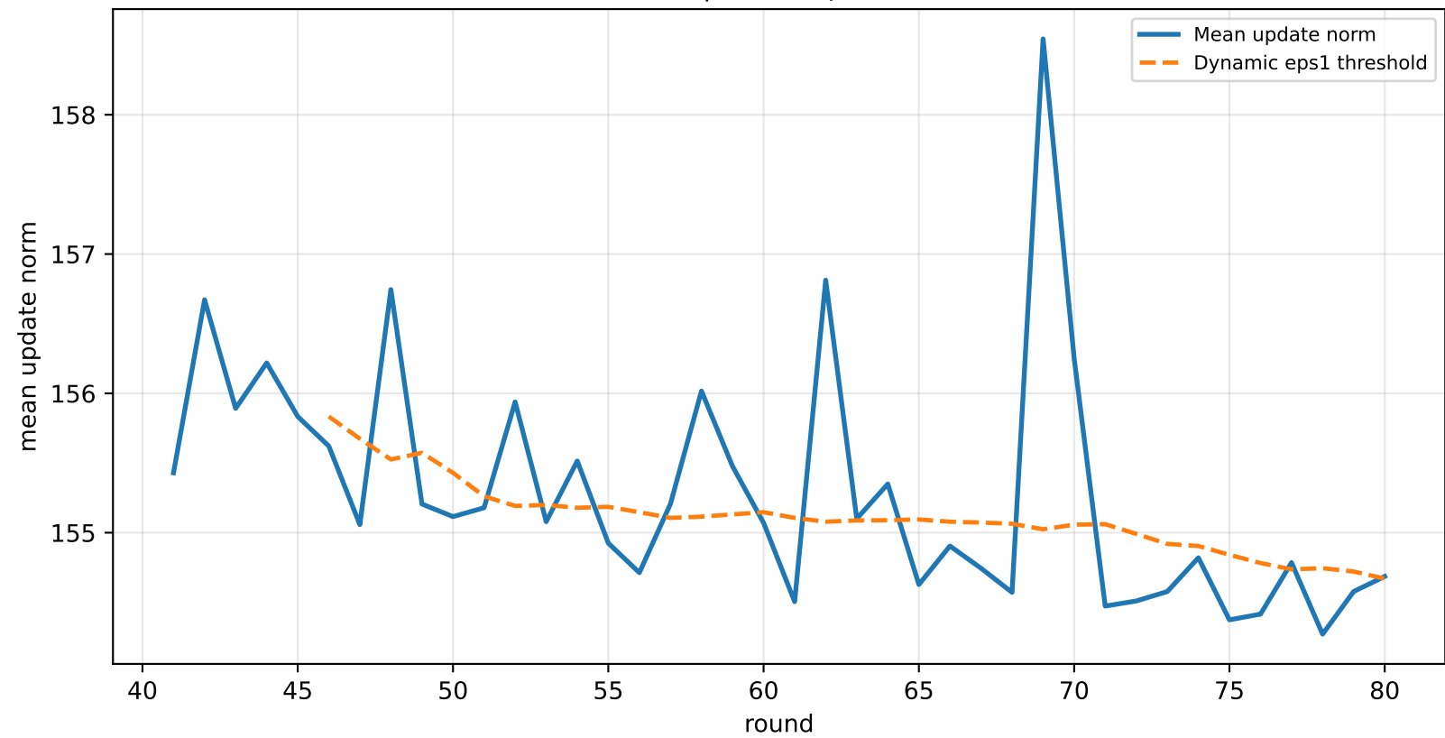
Cluster 4 | Mean update norm
