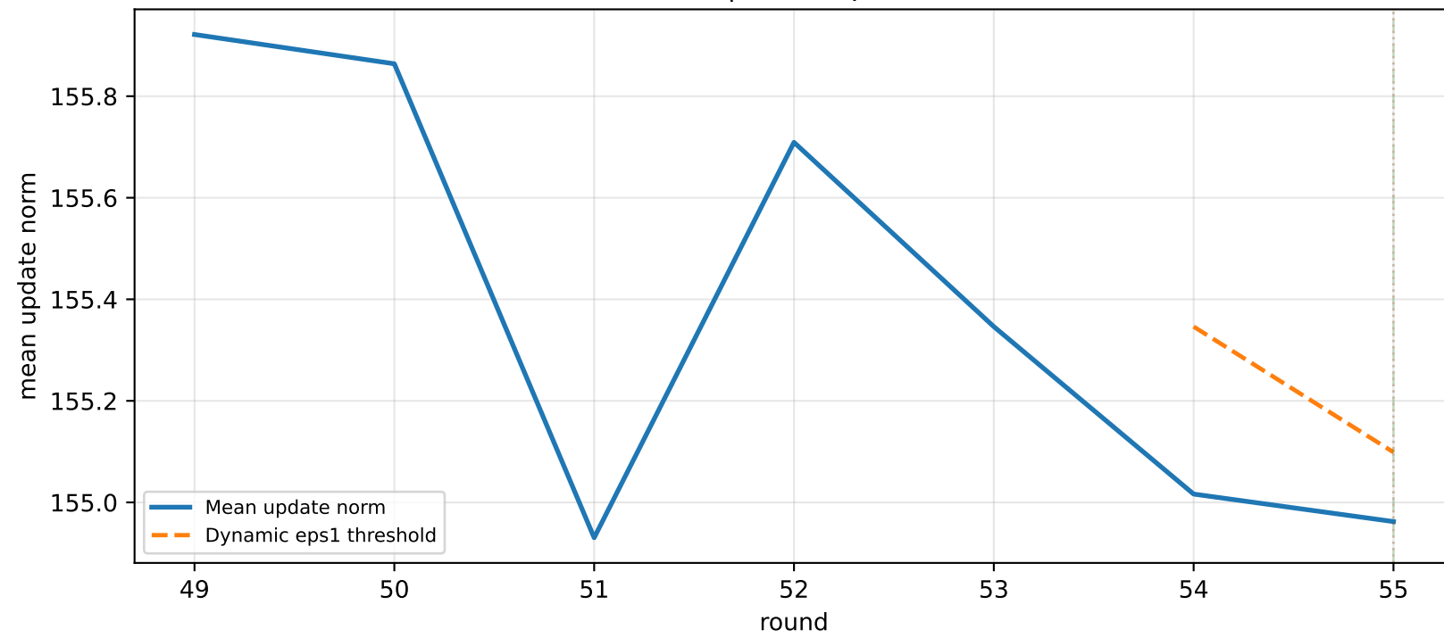
Cluster 10 | Mean update norm
