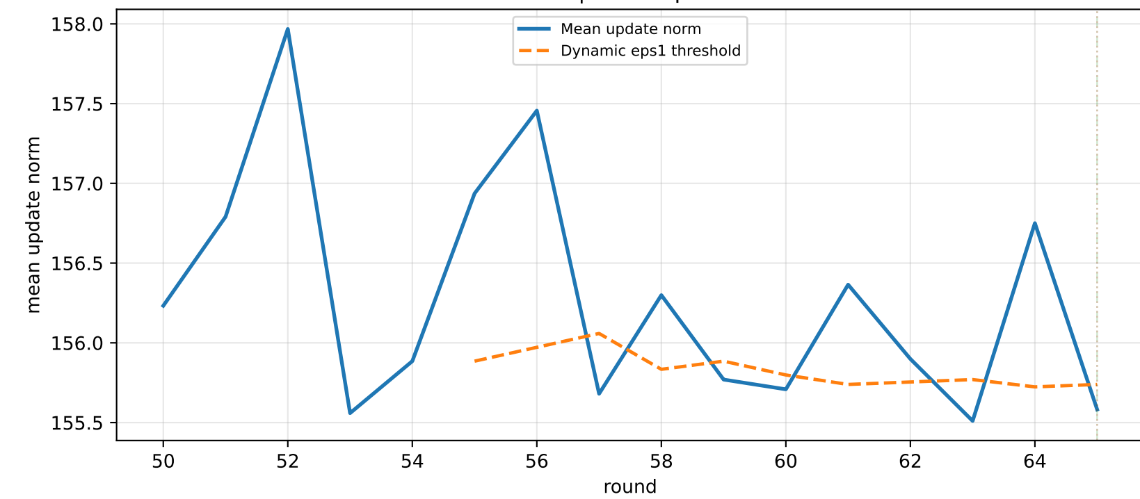
Cluster 10 | Mean update norm
