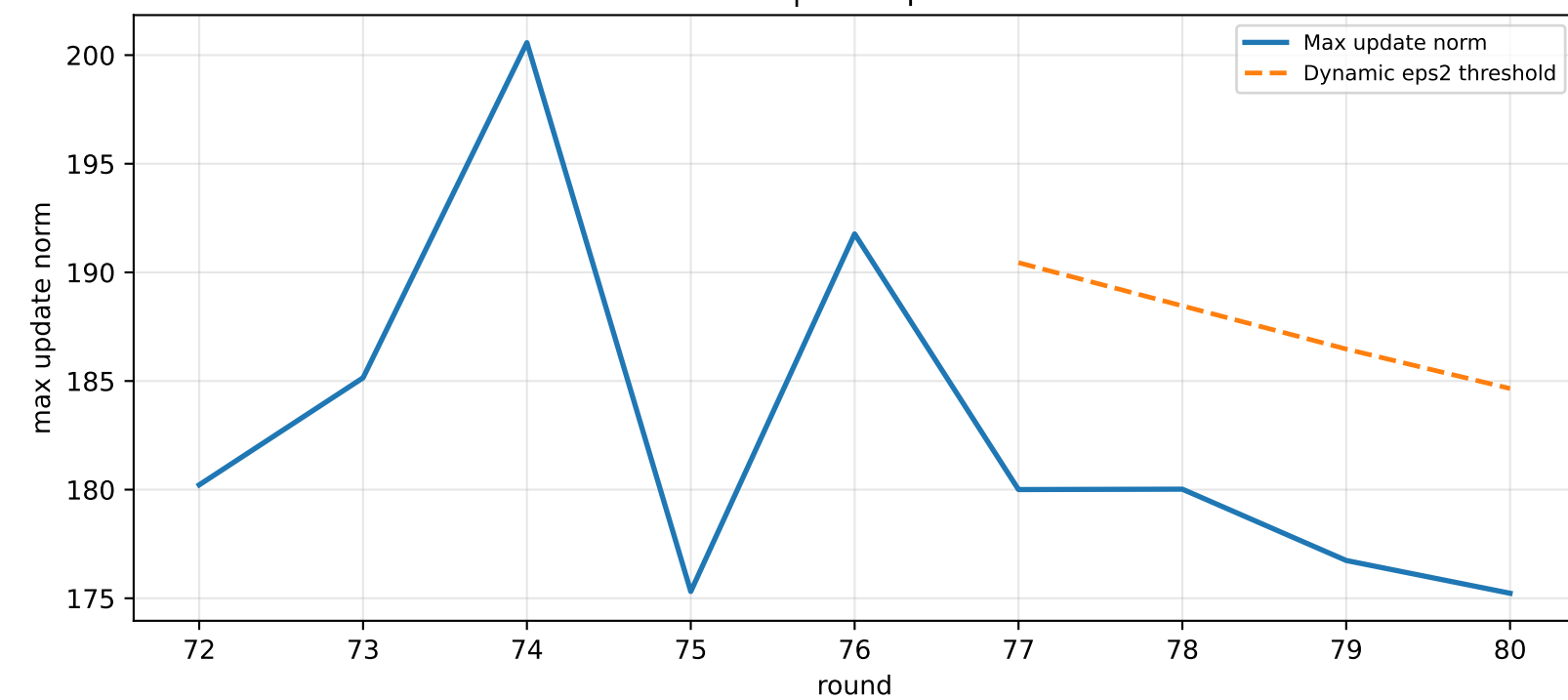
Cluster 14 | Max update norm
