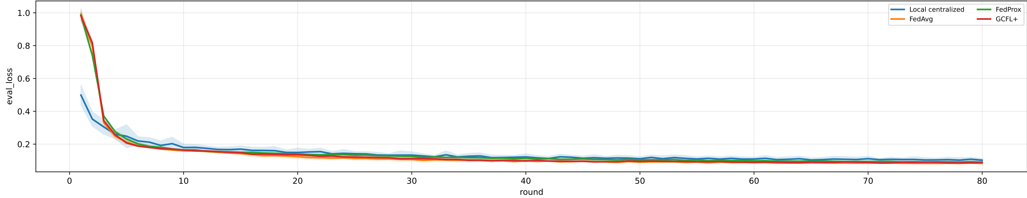
Validation loss comparison
