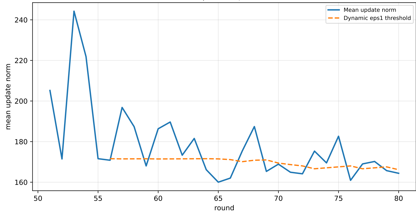
Cluster 3 | Mean update norm
