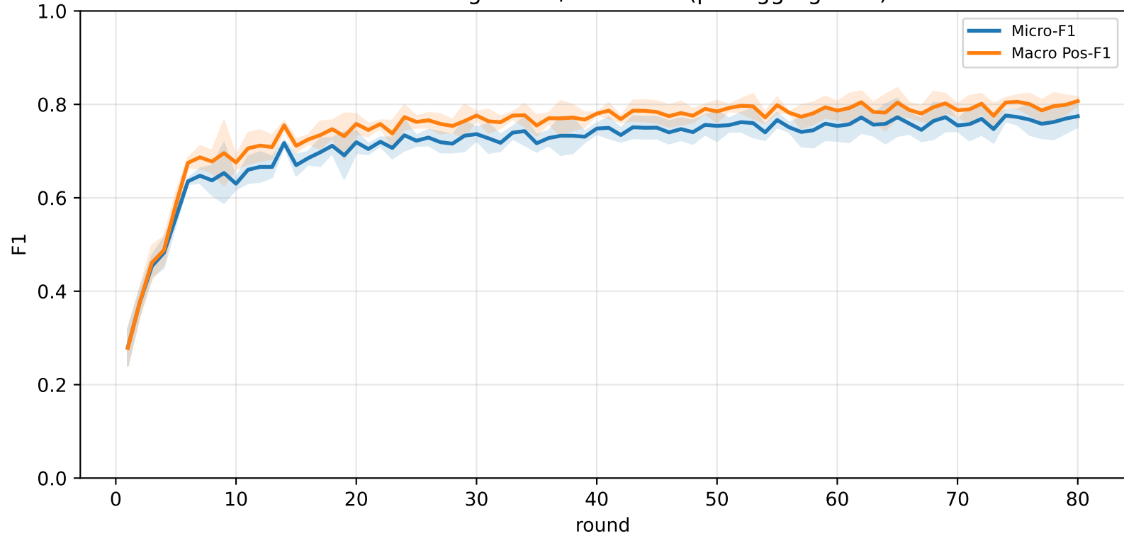
Pooled FedAvg micro / macro F1 (pre-aggregation)
