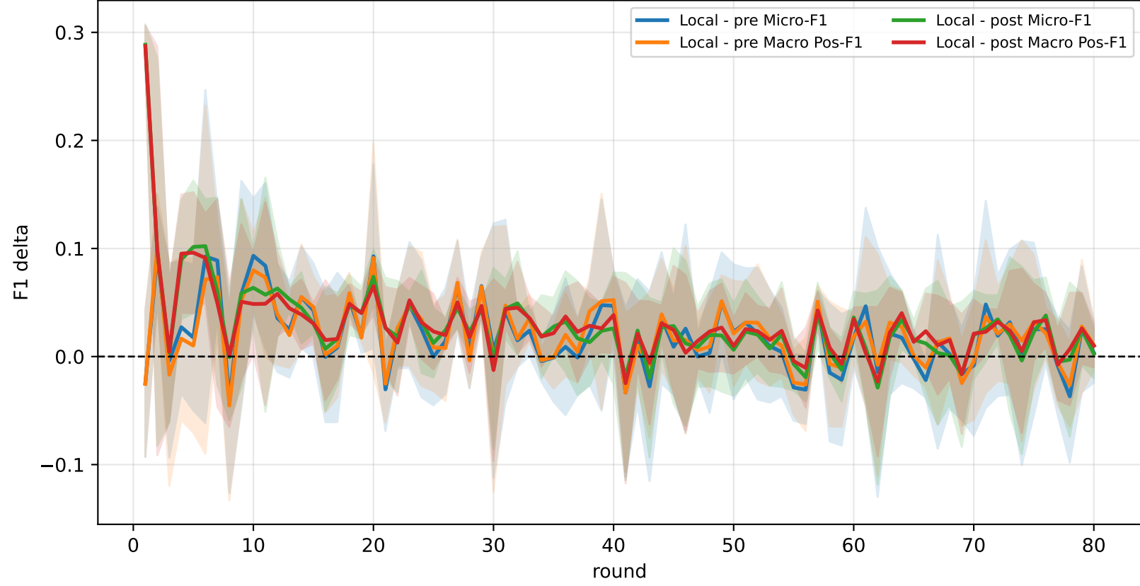
Delta vs FedAvg (local minus pre / post)
