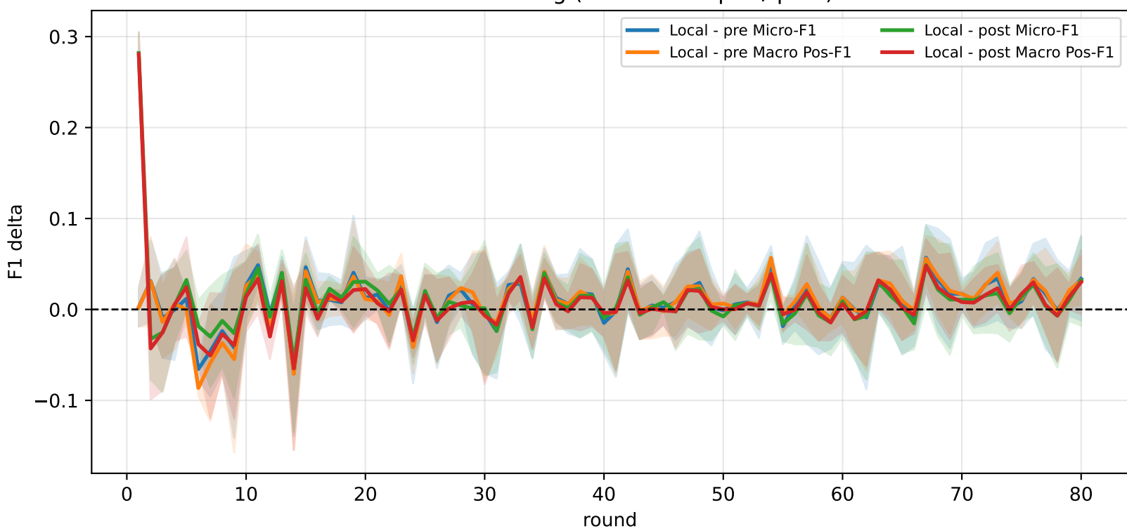
Delta vs FedAvg (local minus pre / post)
