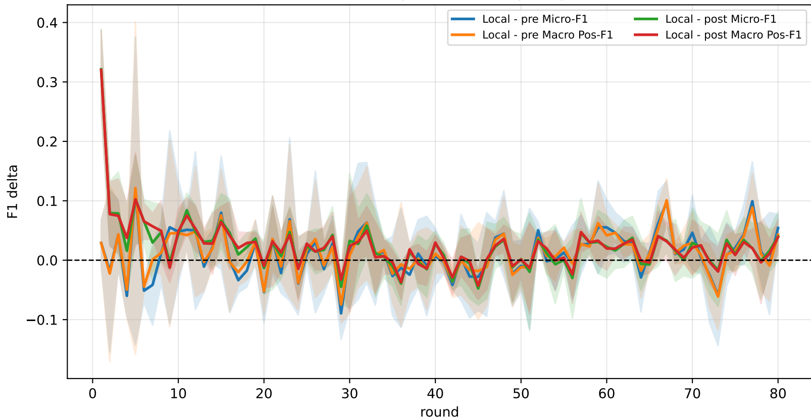
Delta vs FedAvg (local minus pre / post)
