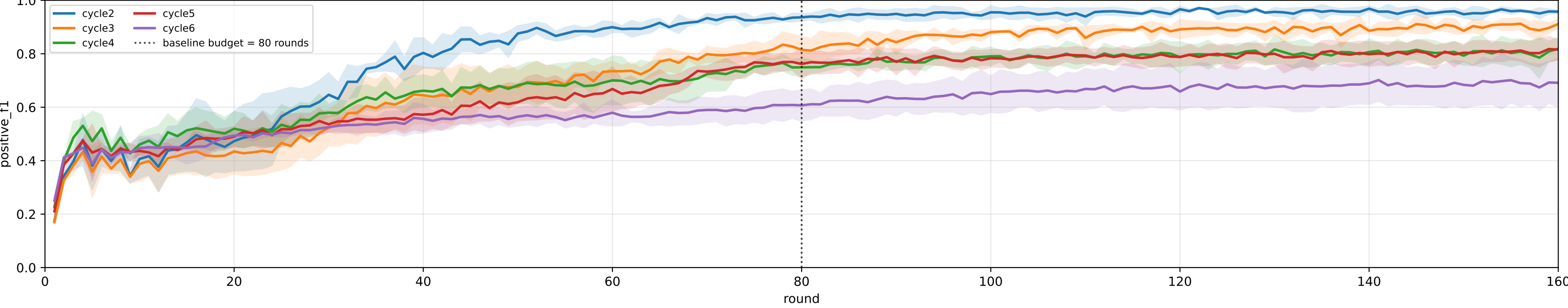
Pooled APPLE positive F1 (after-local selected model, 160-round run)
