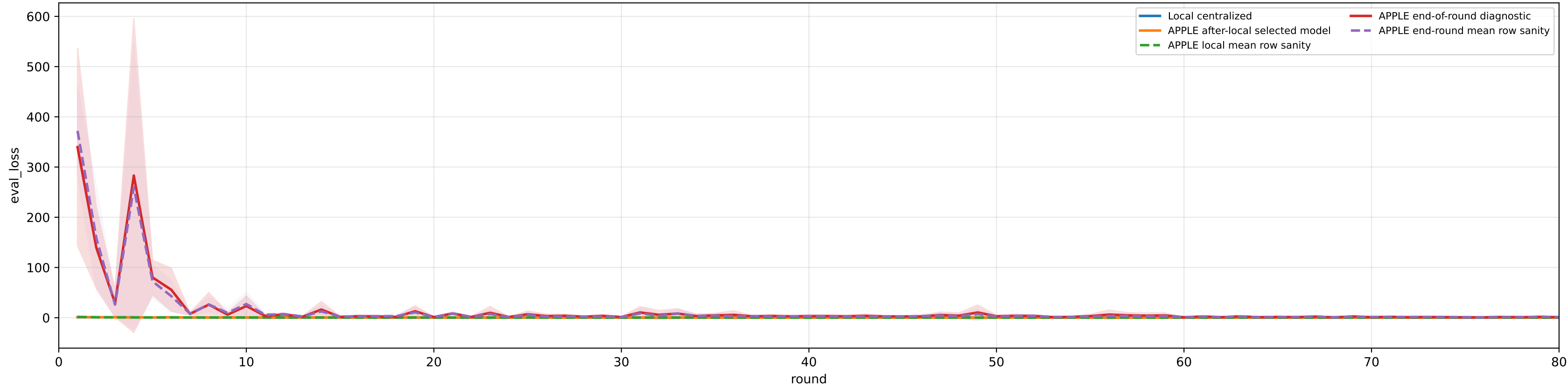
Validation loss: selected APPLE vs end-of-round mismatch (equal 80-round budget)
