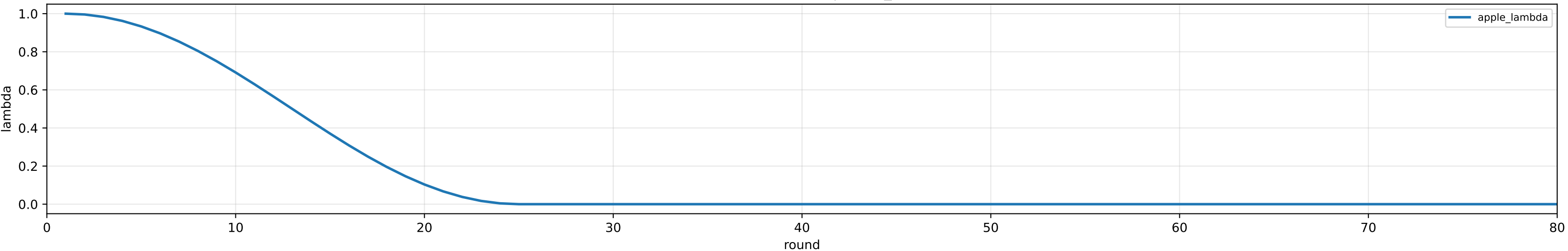
APPLE lambda scheduler | apple_mu=0.01
