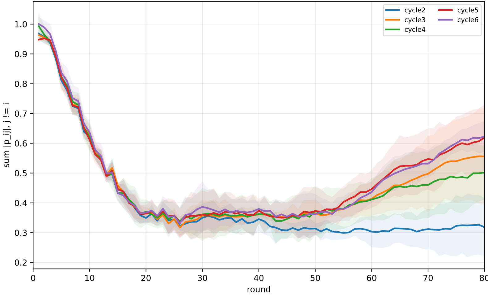
APPLE off-diagonal absolute mass over rounds
