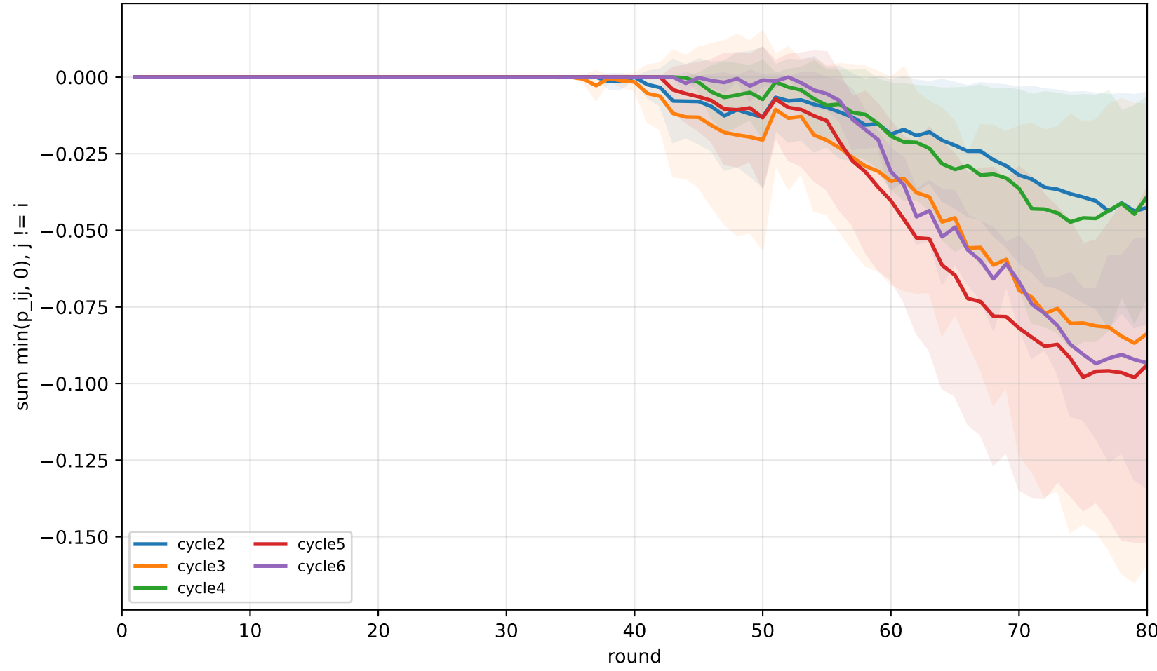
APPLE off-diagonal negative mass over rounds
