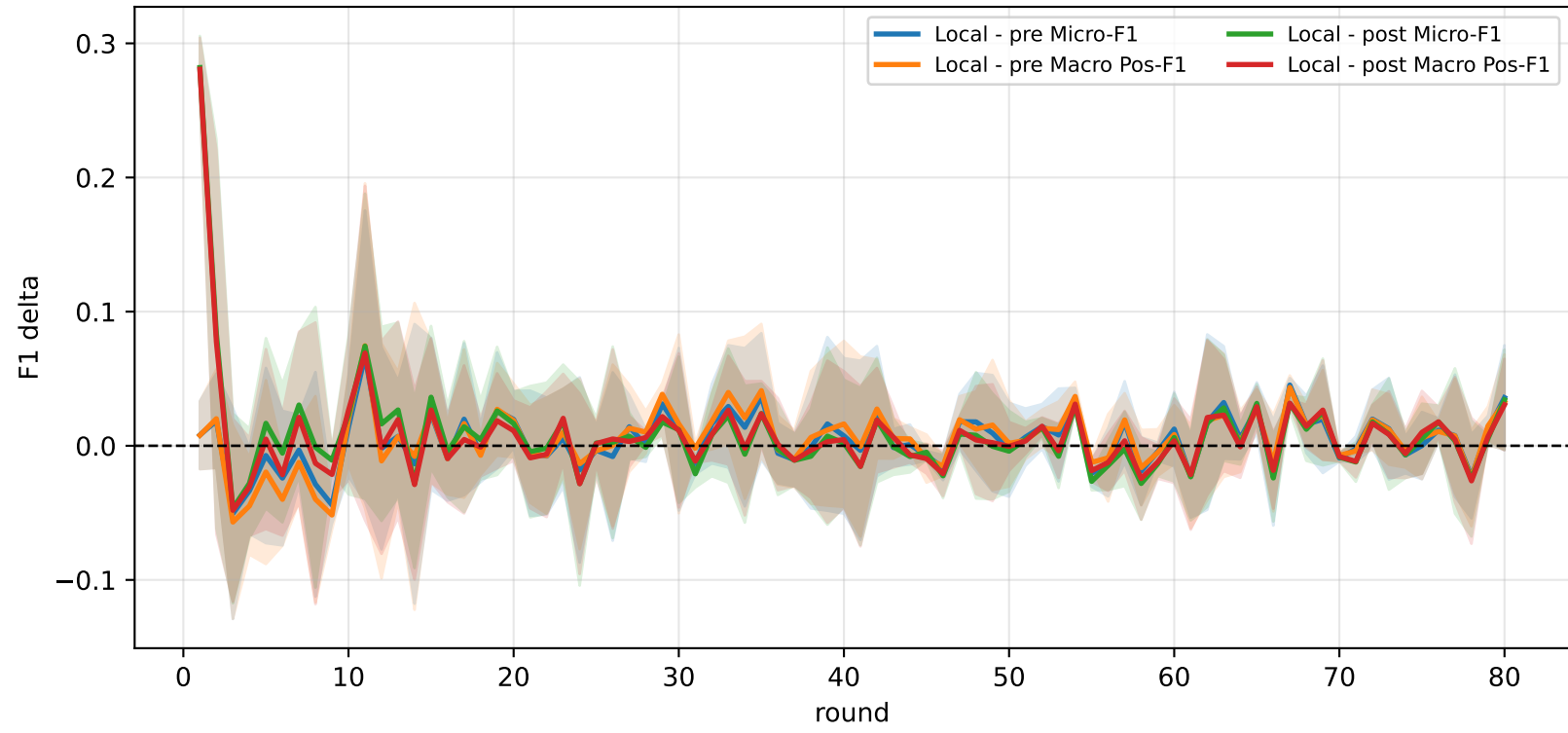
Delta vs GCFL+ (local minus pre / post)
