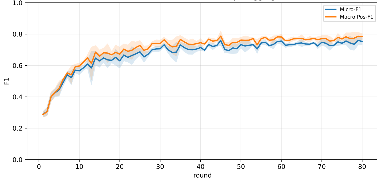
Pooled GCFL+ micro / macro F1 (pre-aggregation)
