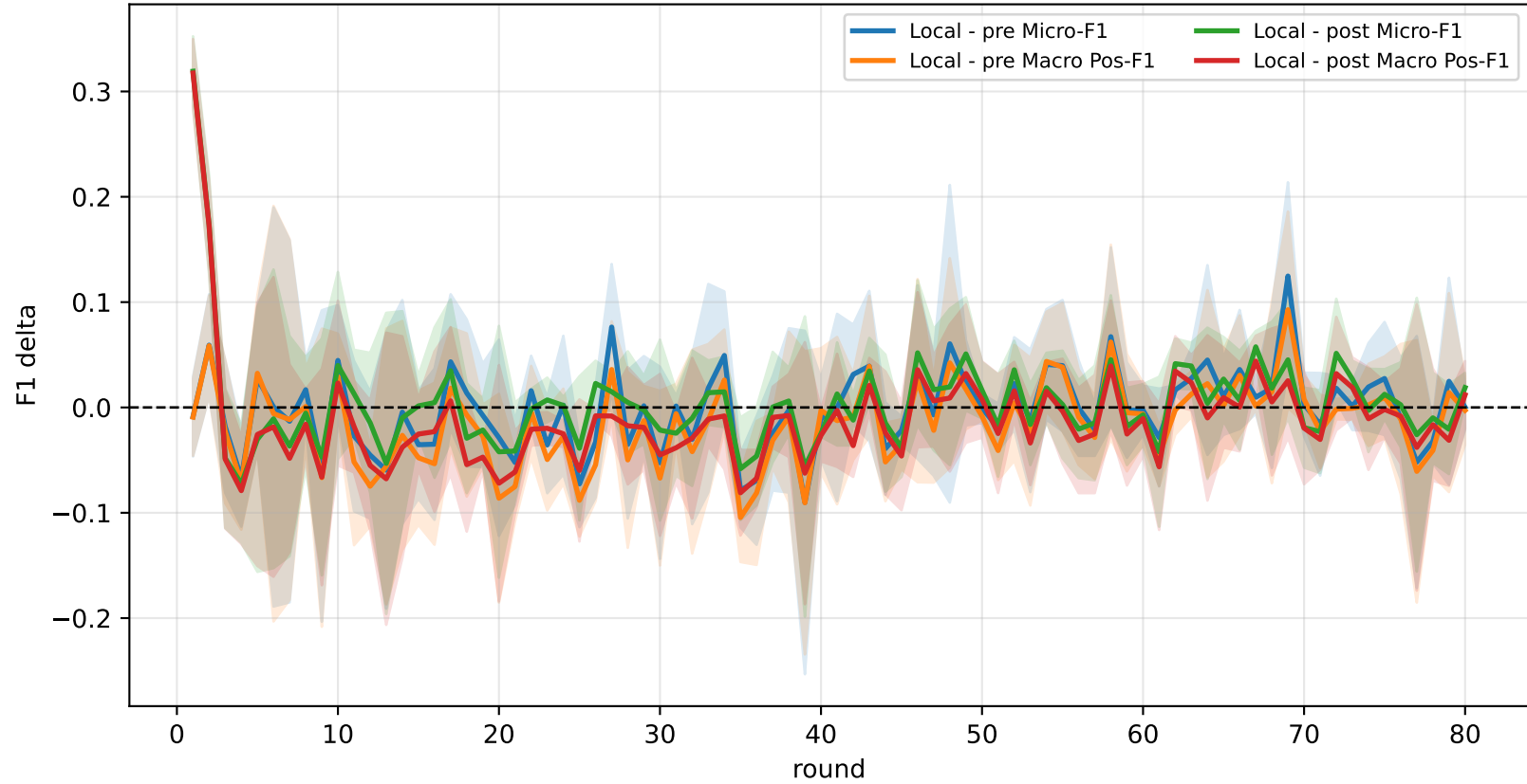
Delta vs GCFL+ (local minus pre / post)
