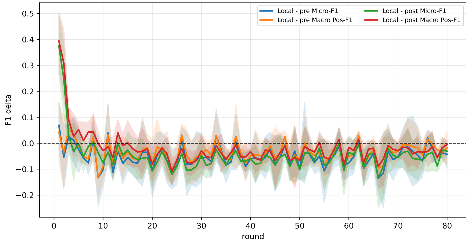
Delta vs GCFL+ (local minus pre / post)
