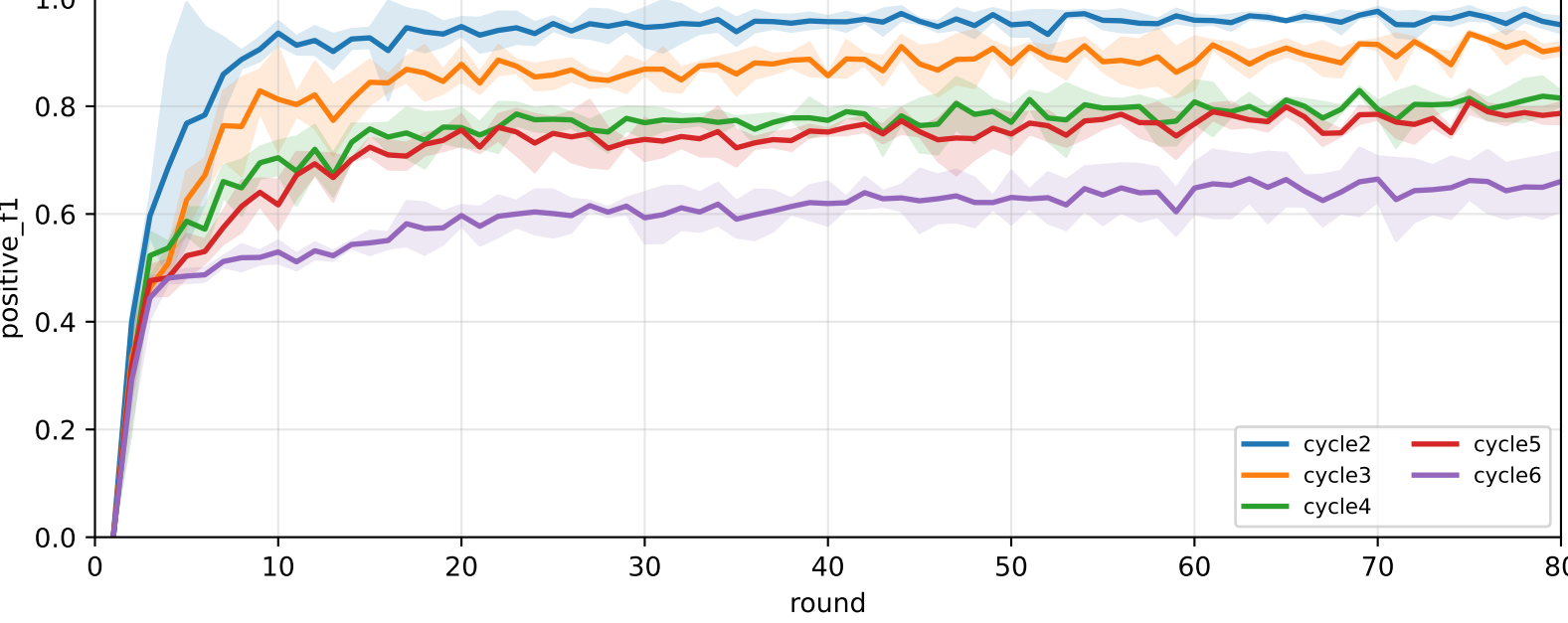
Pooled APPLE positive F1 (after-local selected model, equal 80-round budget)
