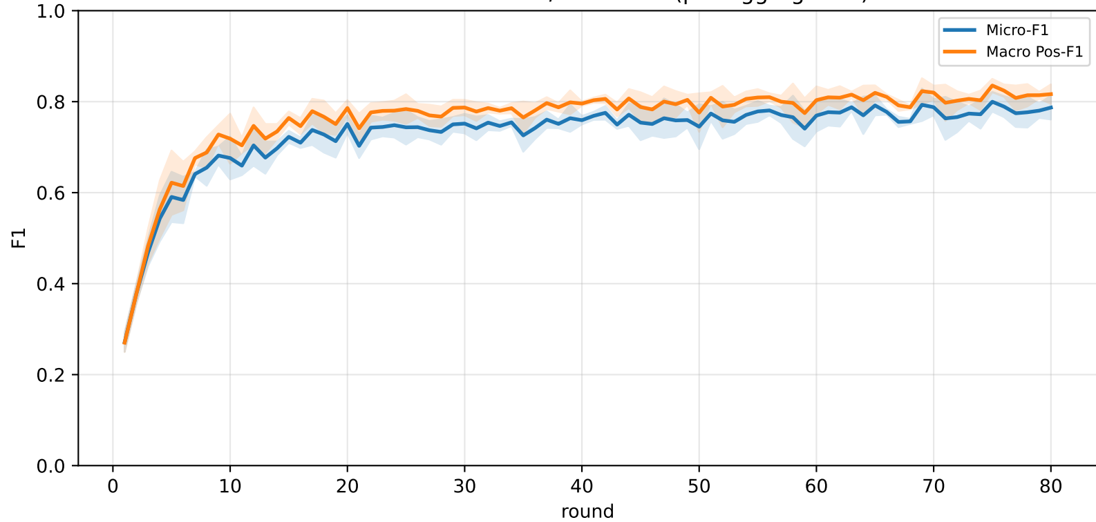
Pooled FedProx micro / macro F1 (pre-aggregation)
