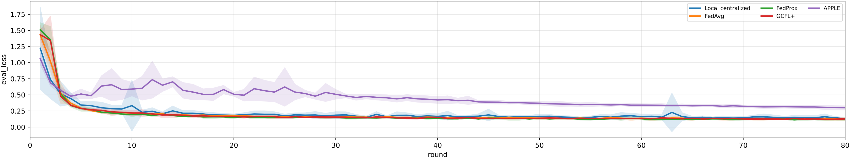
Validation loss comparison (all methods 80 rounds; APPLE dr_lr=0.0003, mu=0.01, Lfrac=0.3)
