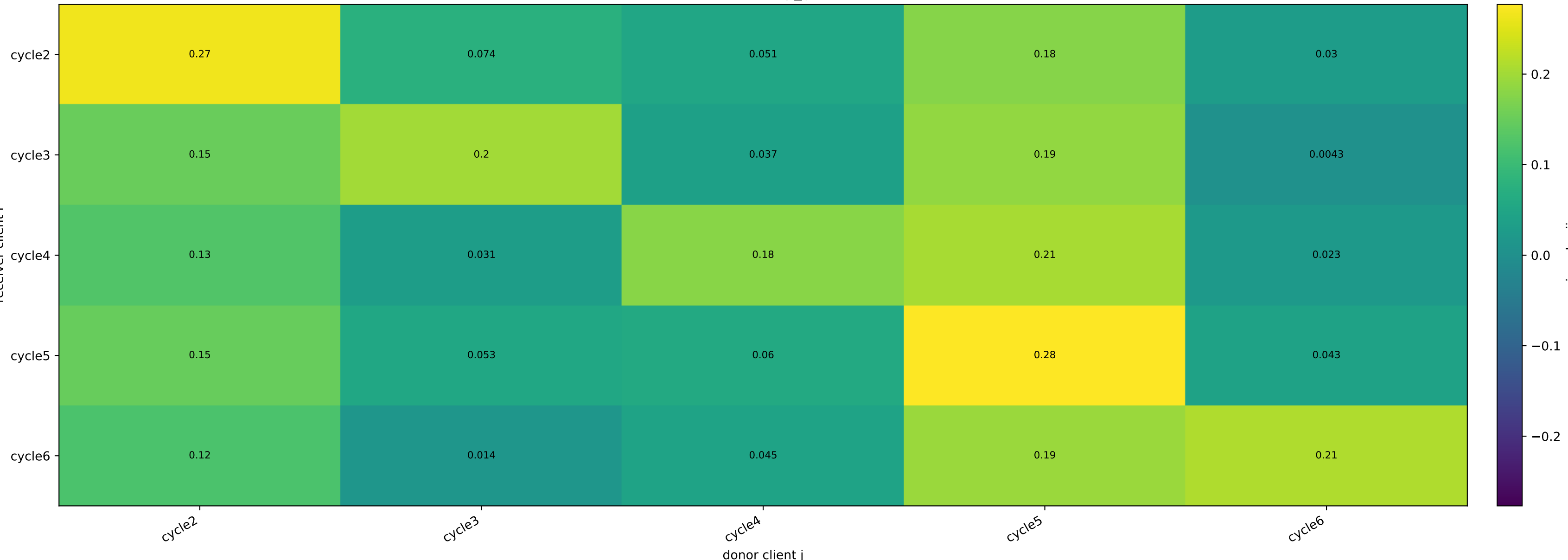
Final APPLE DR coefficients p_{ij} , mean over seeds
