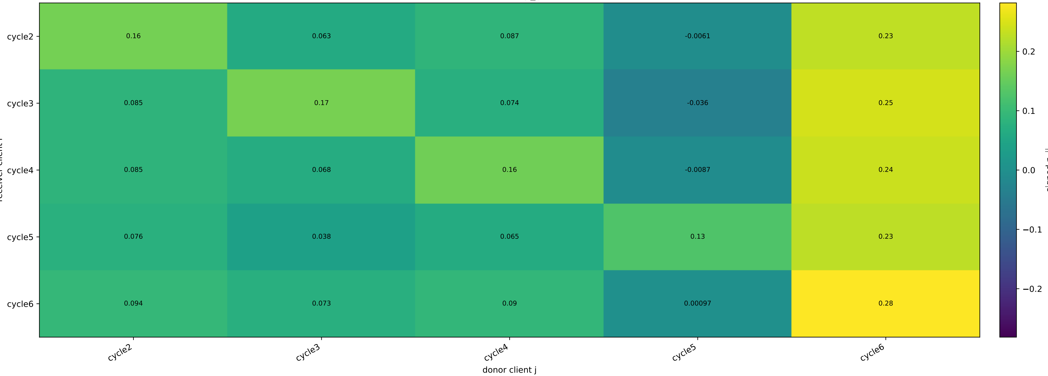
Final APPLE DR coefficients p_{ij} , mean over seeds
