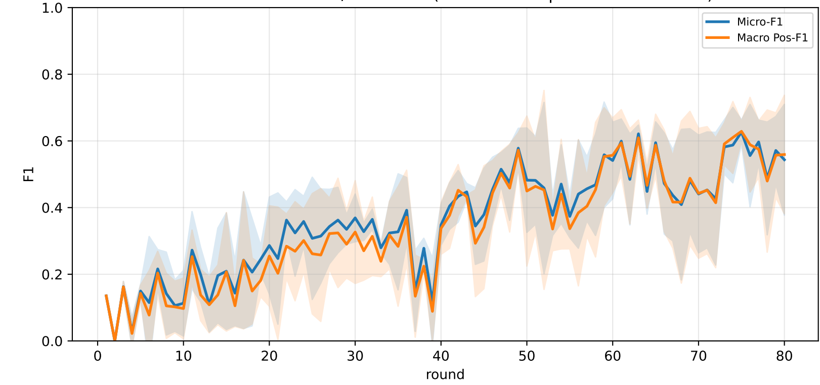
Pooled APPLE micro / macro F1 (end-of-round personalized model)
