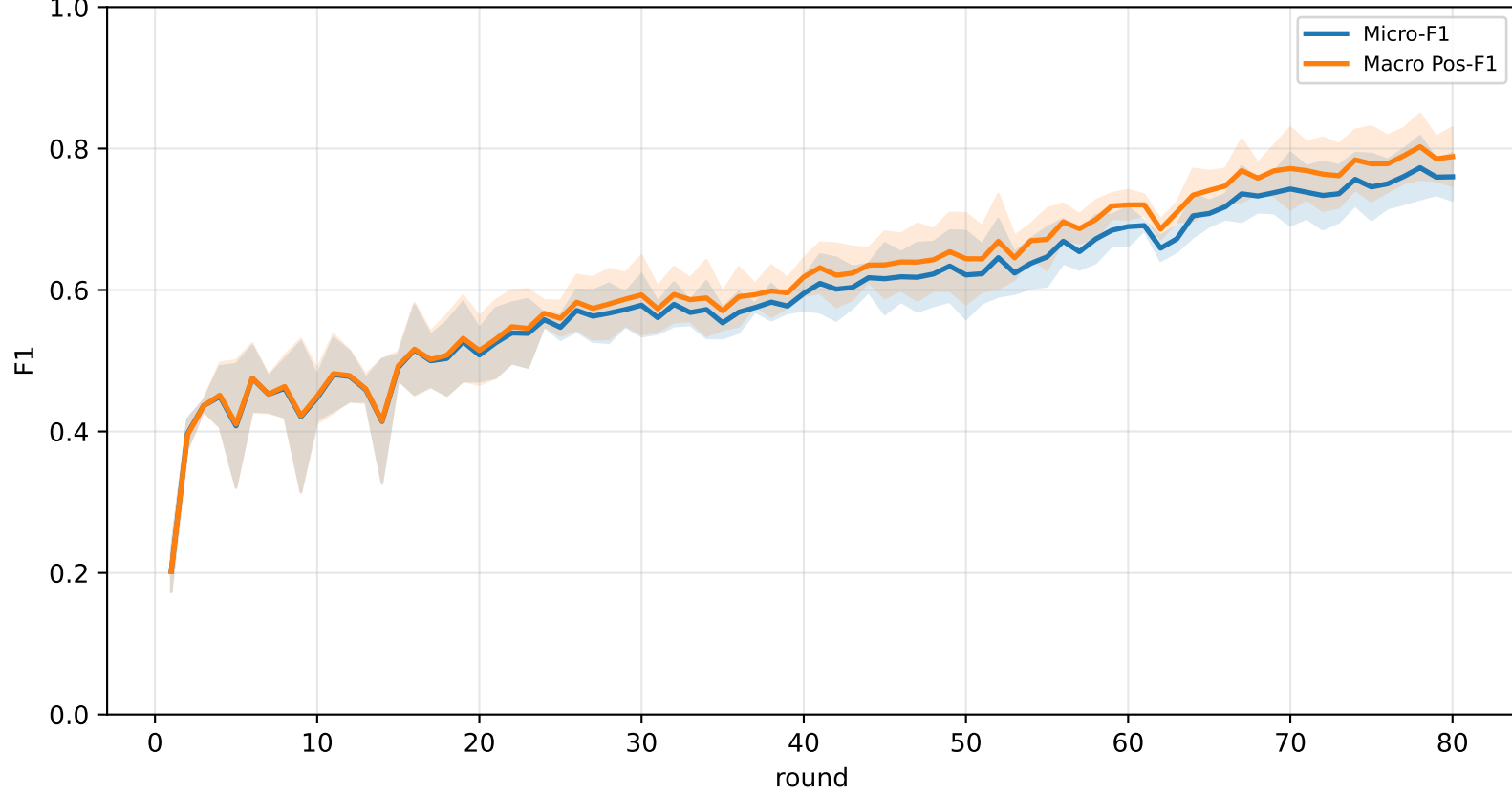
Pooled APPLE micro / macro F1 (after local Apple update)
