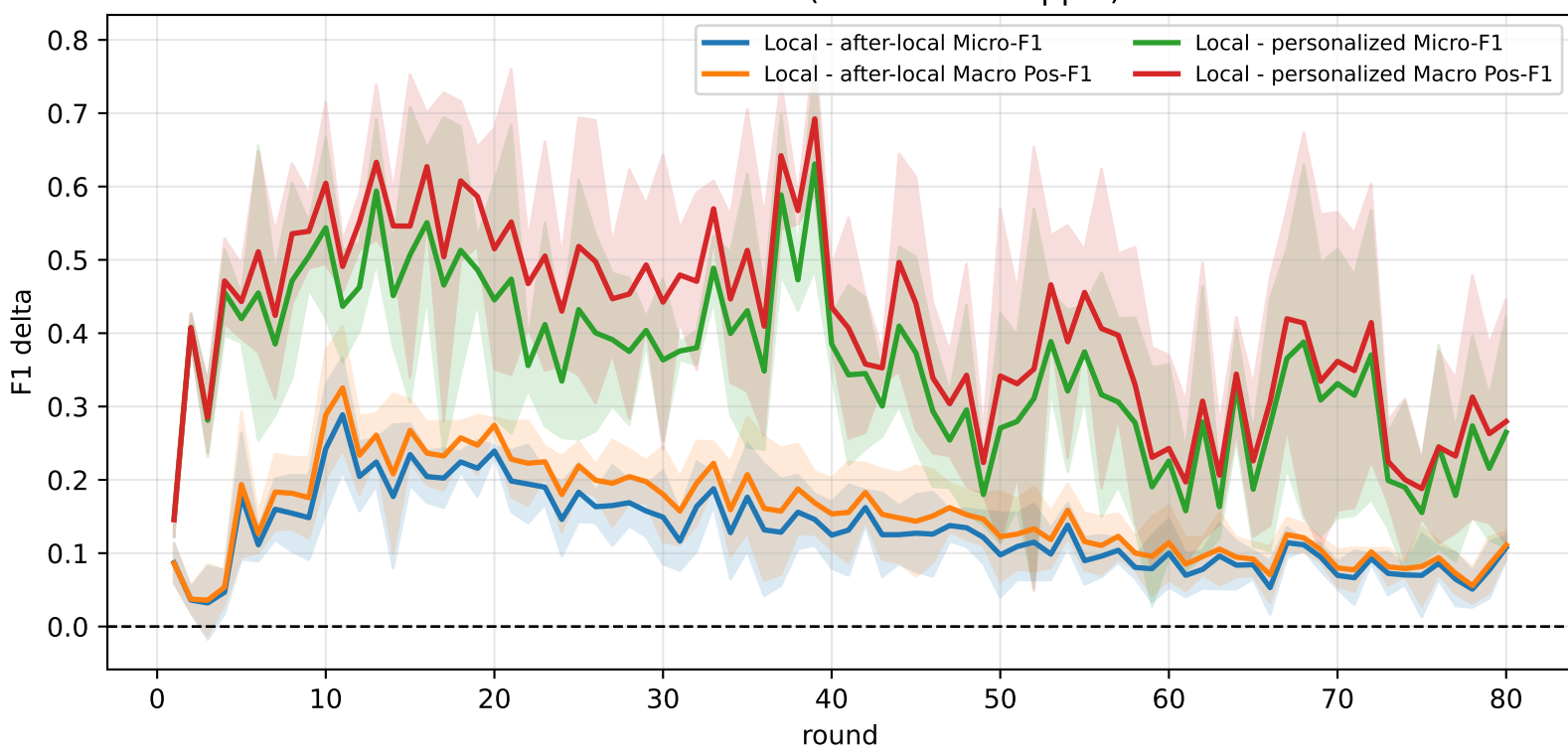
Delta vs APPLE (Local minus Apple)
