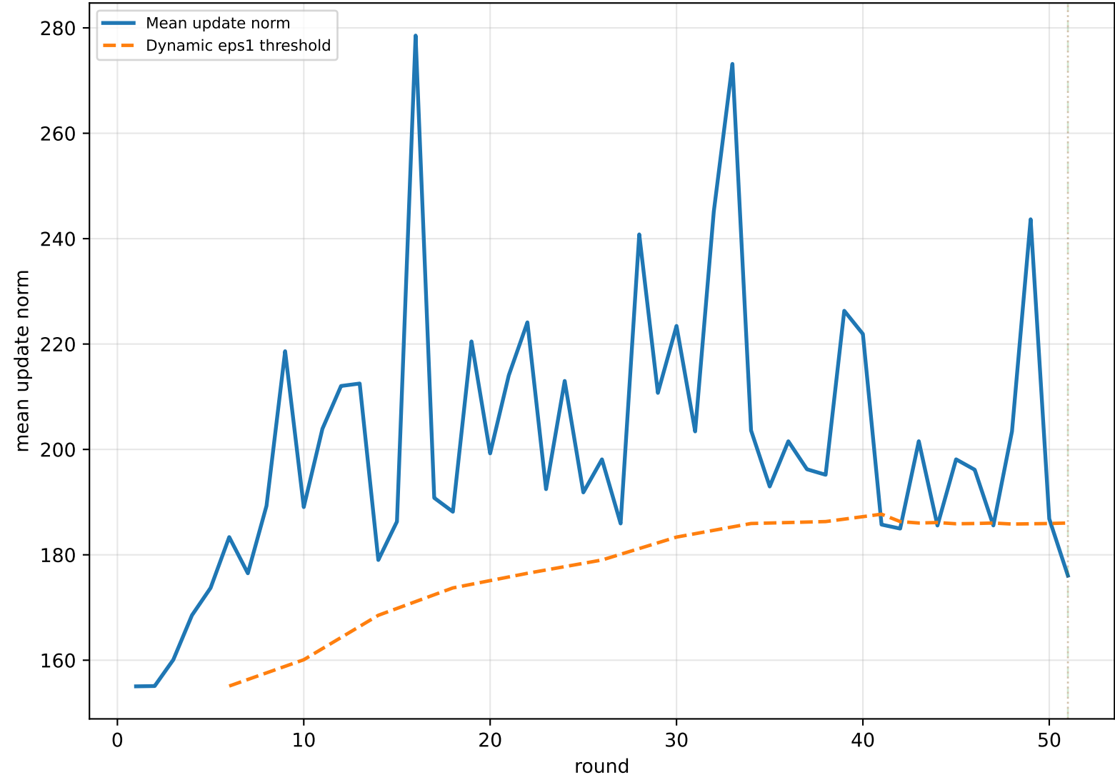
Cluster 0 | Mean update norm
