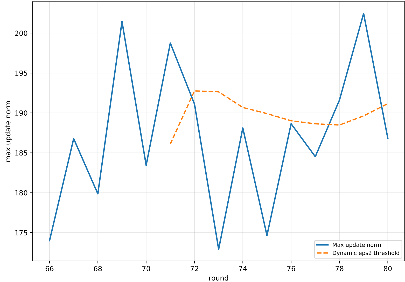
Cluster 6 | Max update norm
