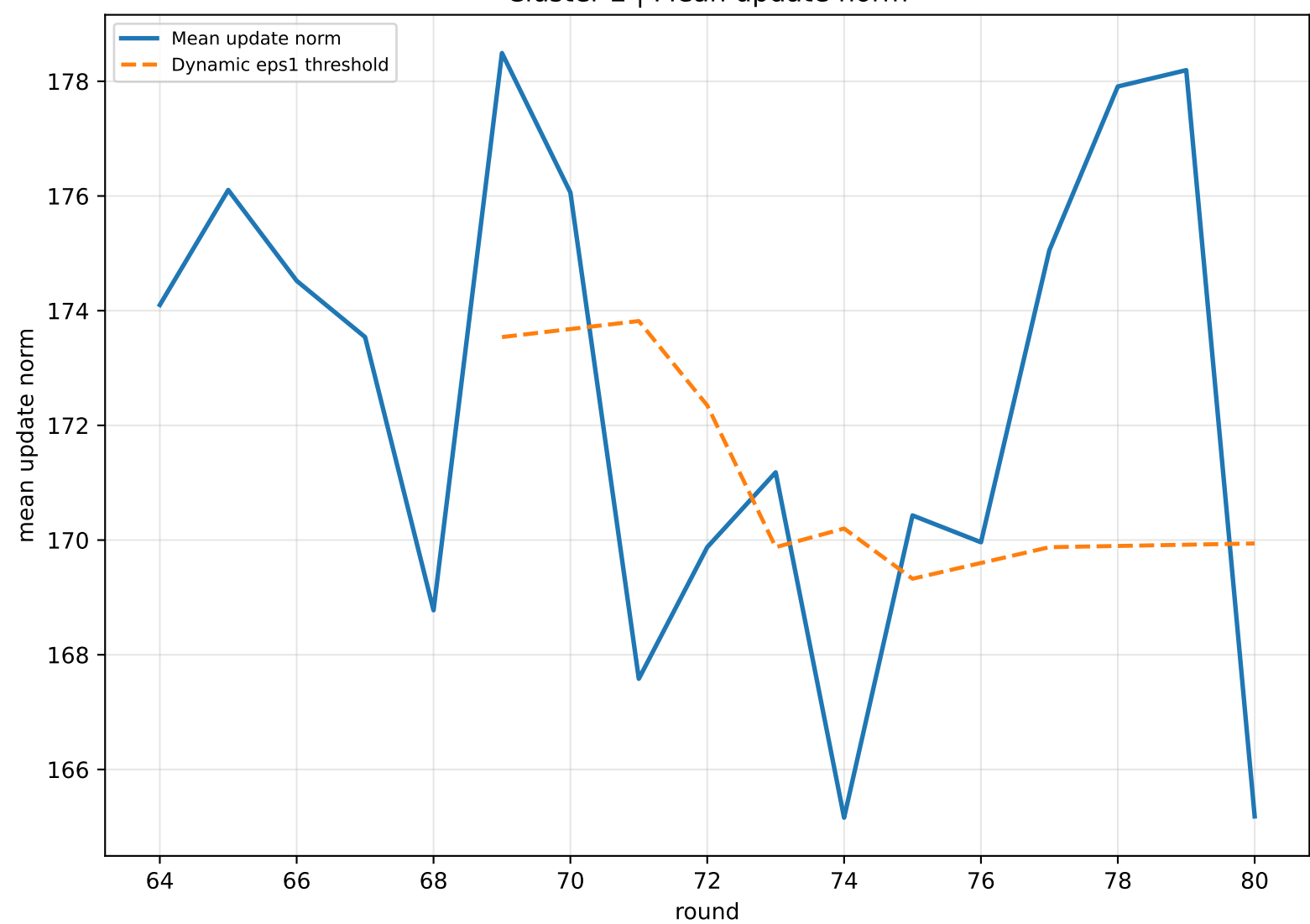
Cluster 2 | Mean update norm
