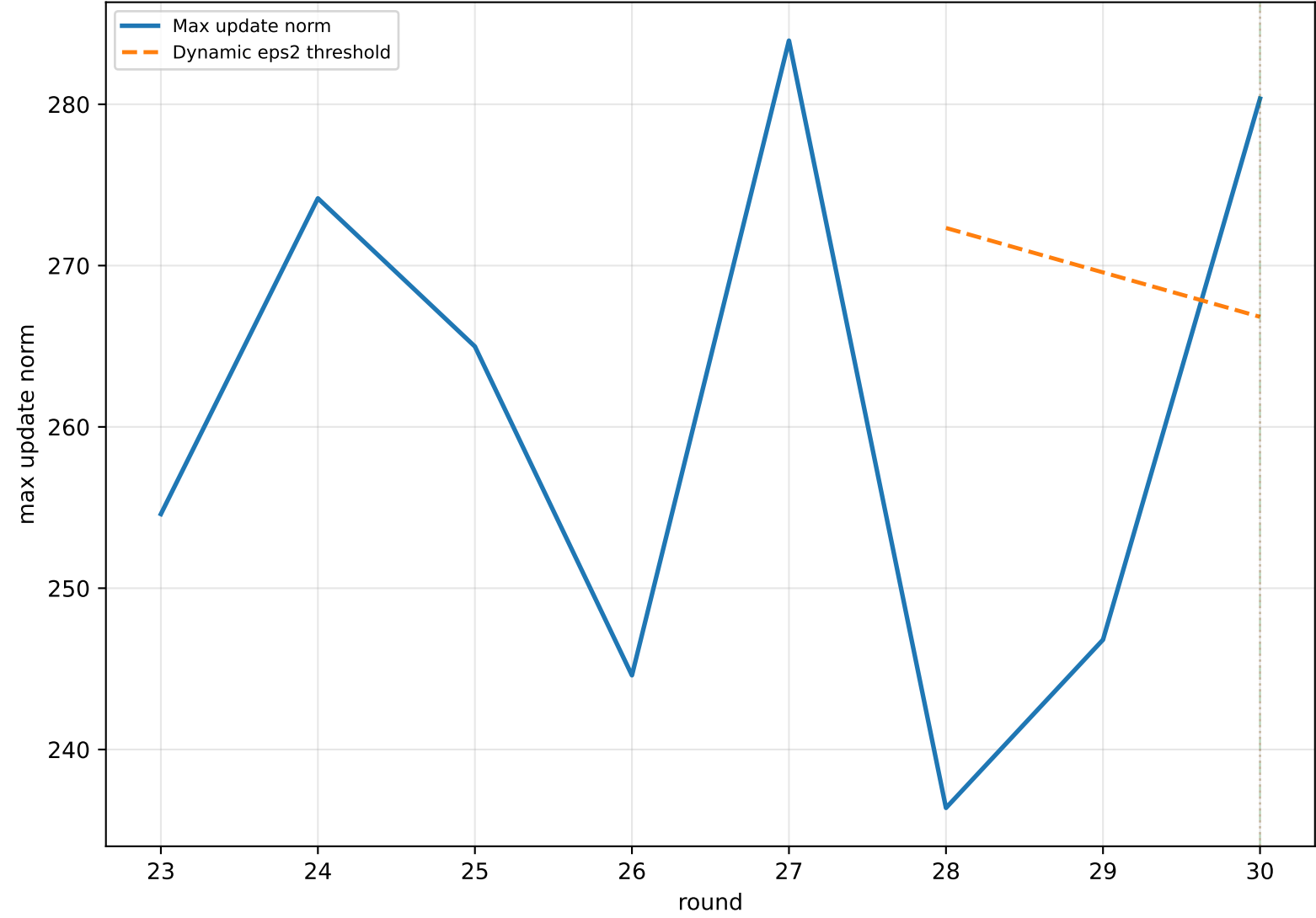
Cluster 1 | Max update norm
