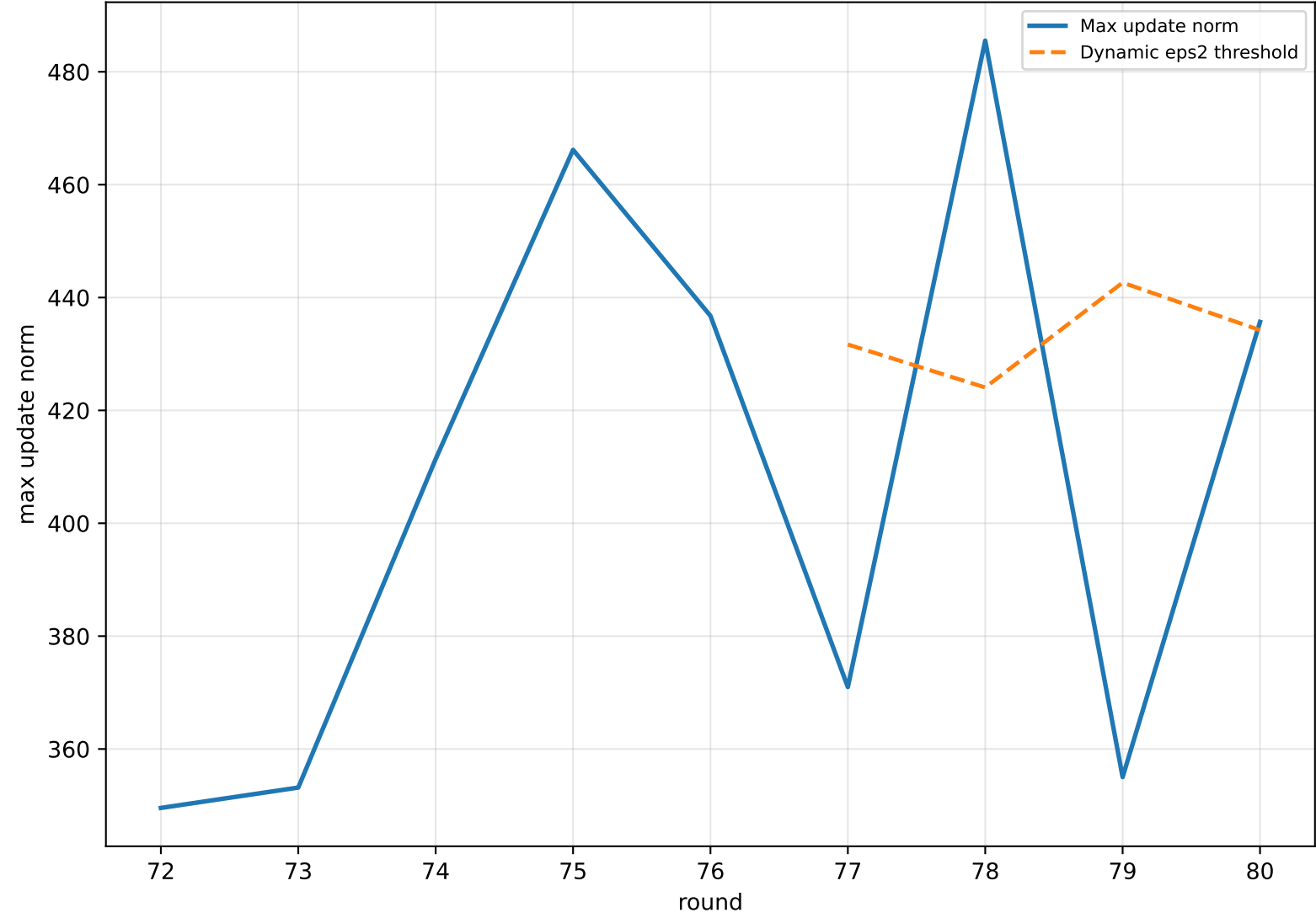
Cluster 2 | Max update norm
