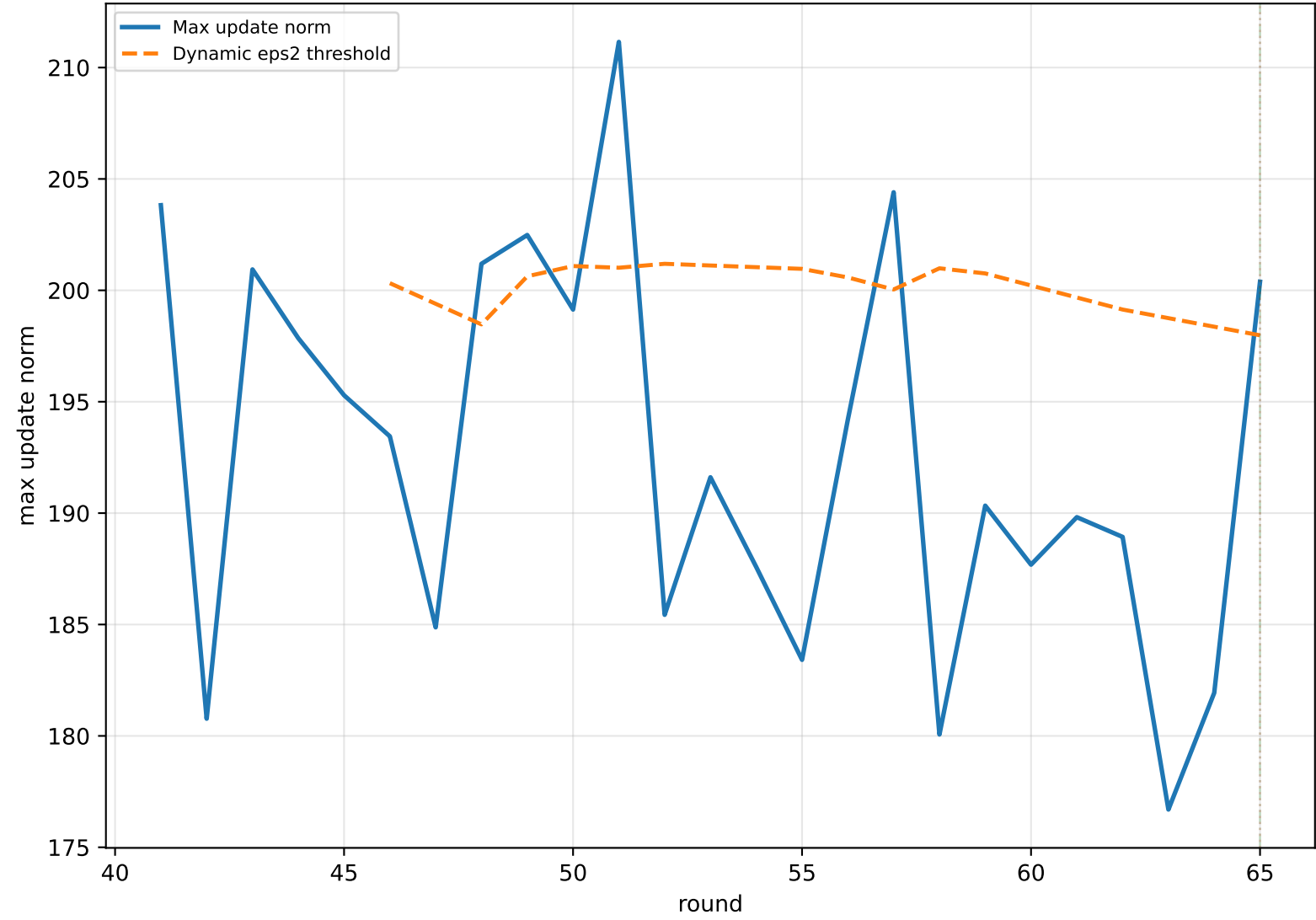
Cluster 4 | Max update norm
