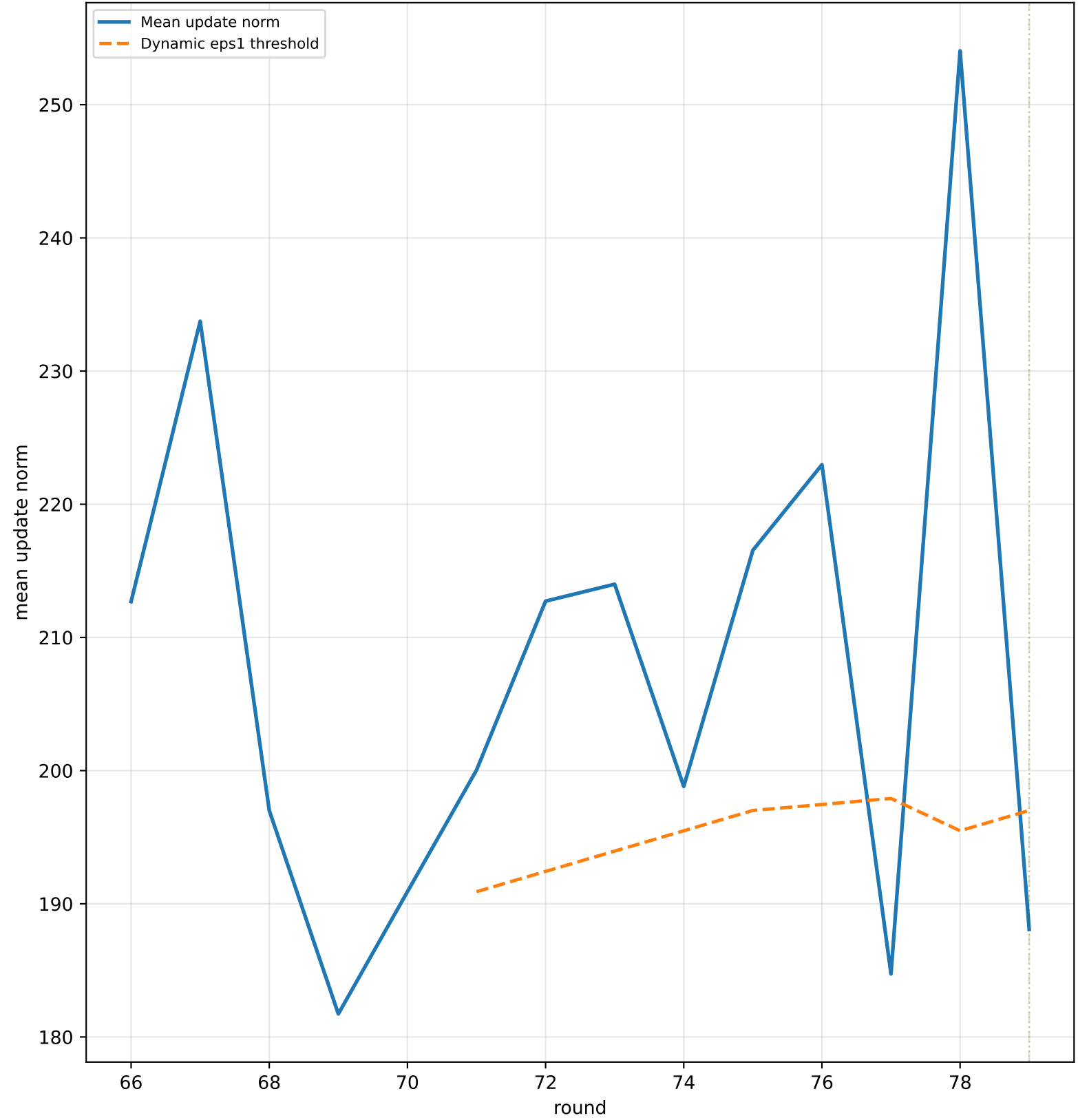
Cluster 4 | Mean update norm
