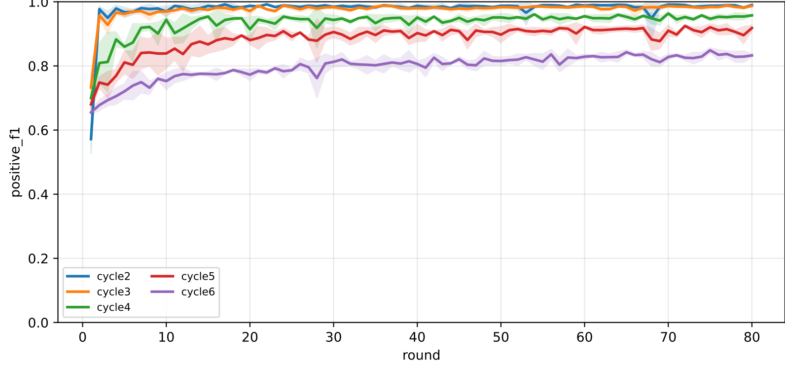
Pooled local centralized positive F1
