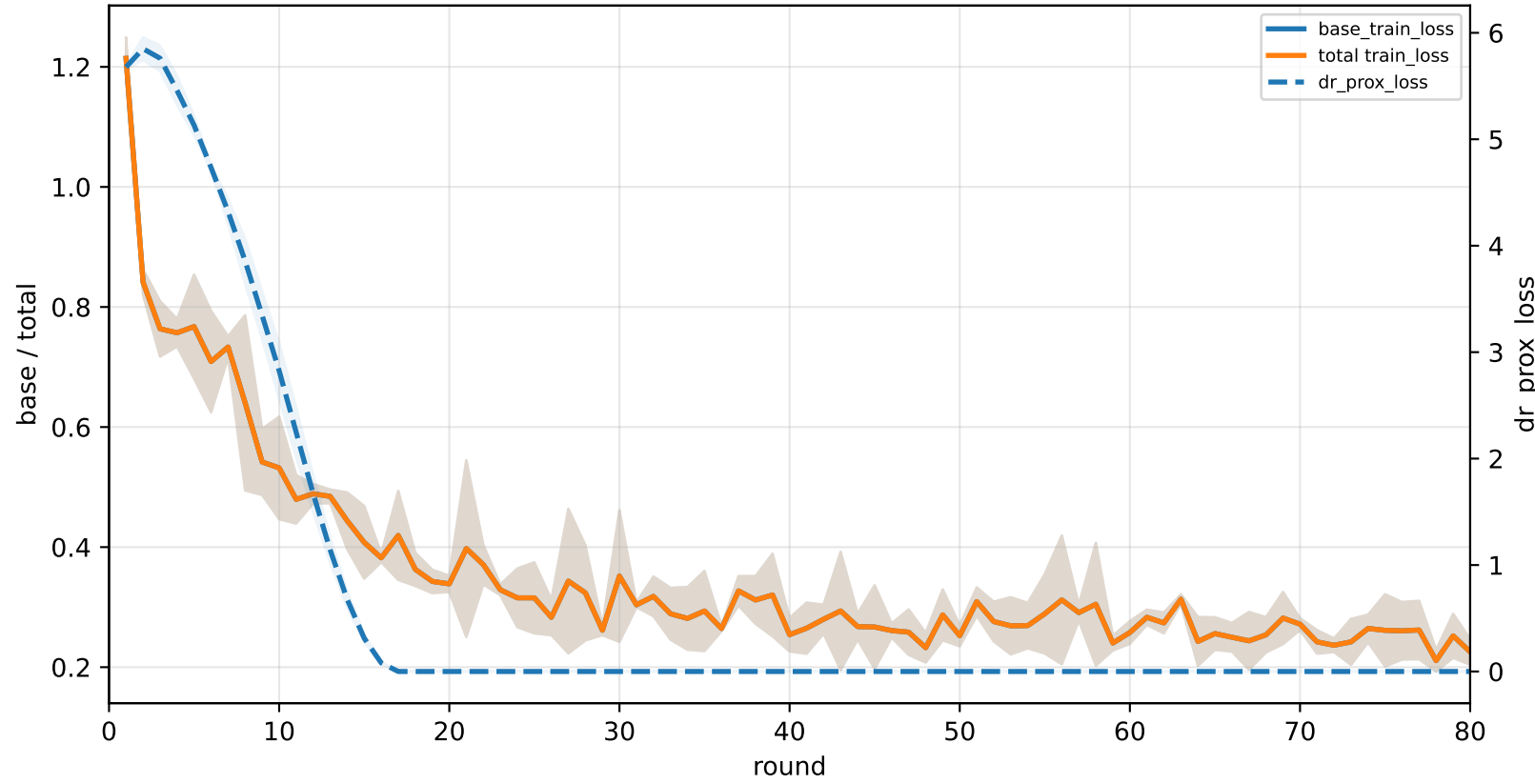
C5-specialist | graph_id=3000008
