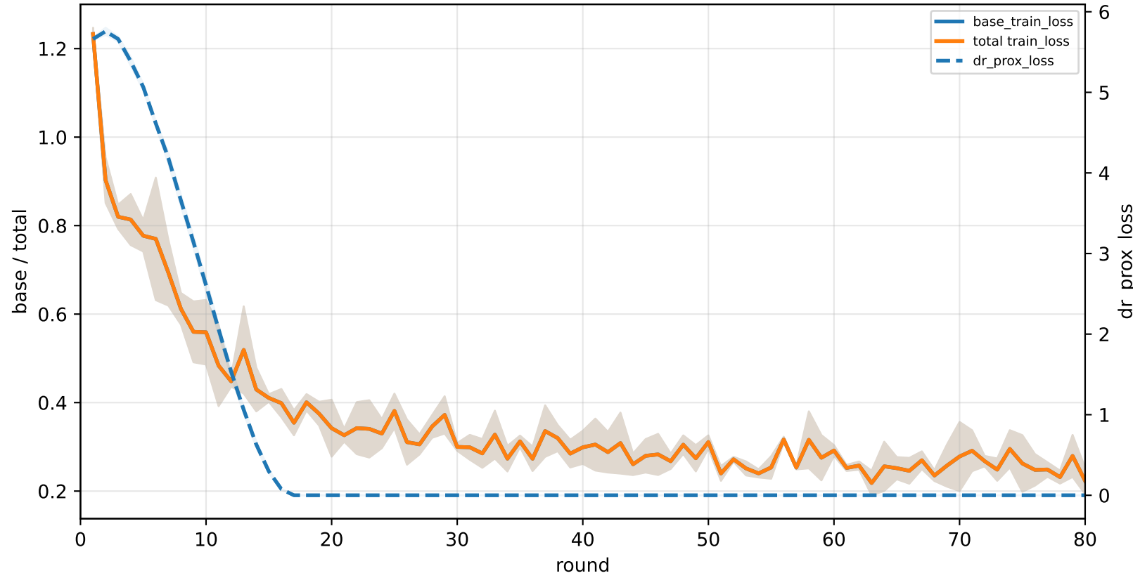
C3-specialist | graph_id=3000006
