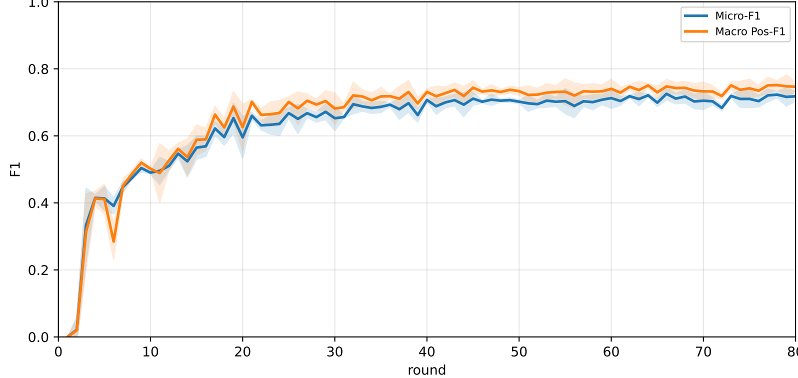
Pooled APPLE-QOracle micro / macro F1 (end-of-round diagnostic only)
