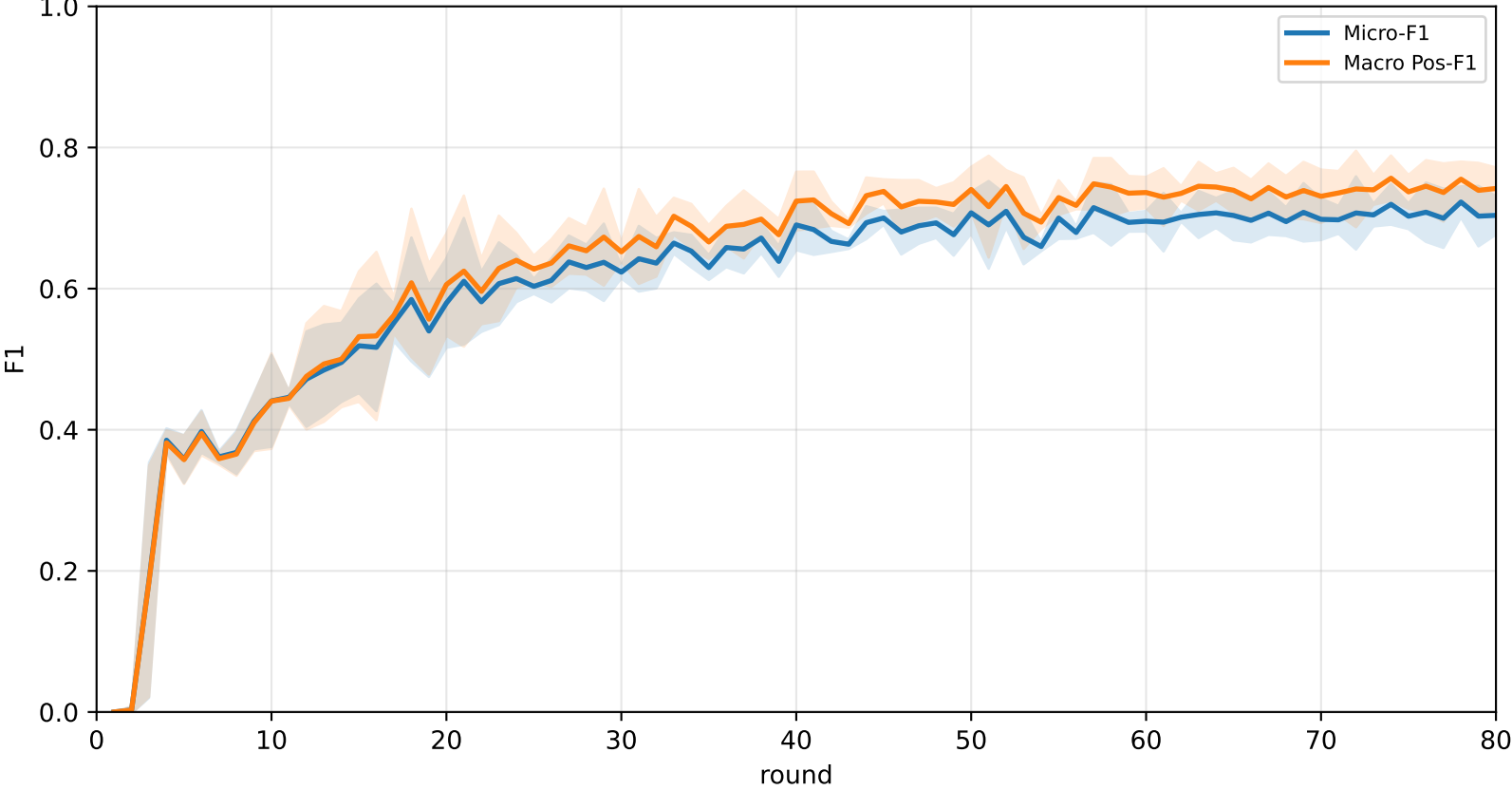
Pooled APPLE-QOracle micro / macro F1 (end-of-round diagnostic only)
