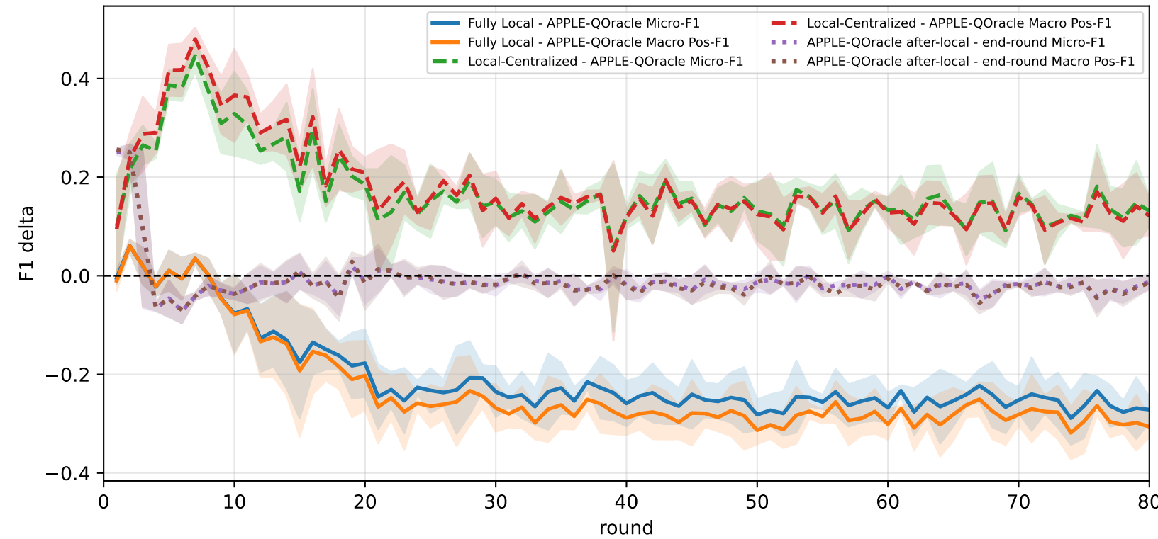
Delta diagnostics: baseline gaps and APPLE-QOracle mismatch gap
