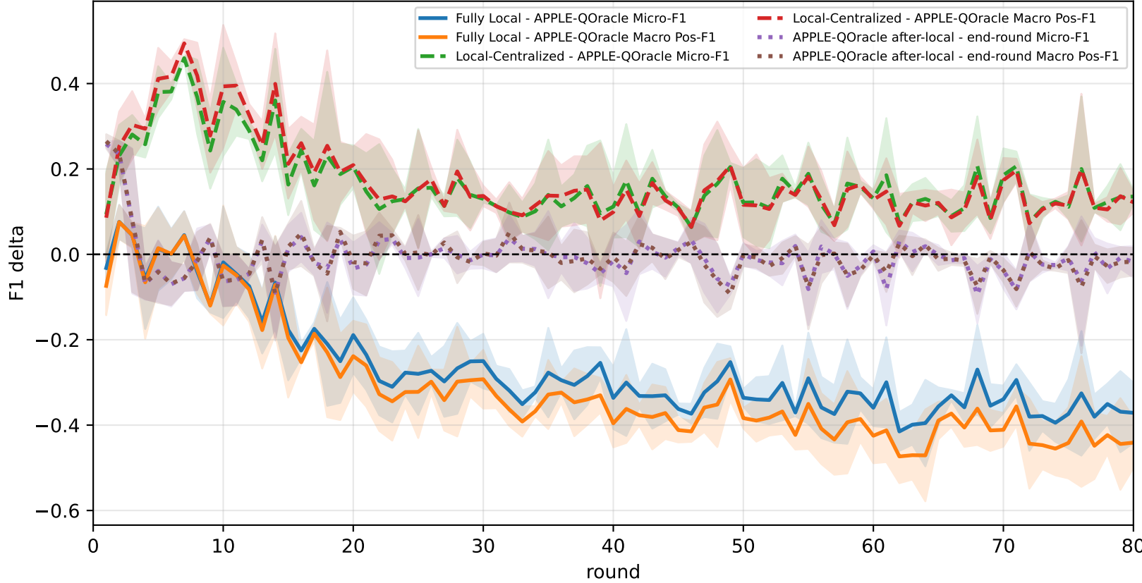
Delta diagnostics: baseline gaps and APPLE-QOracle mismatch gap
