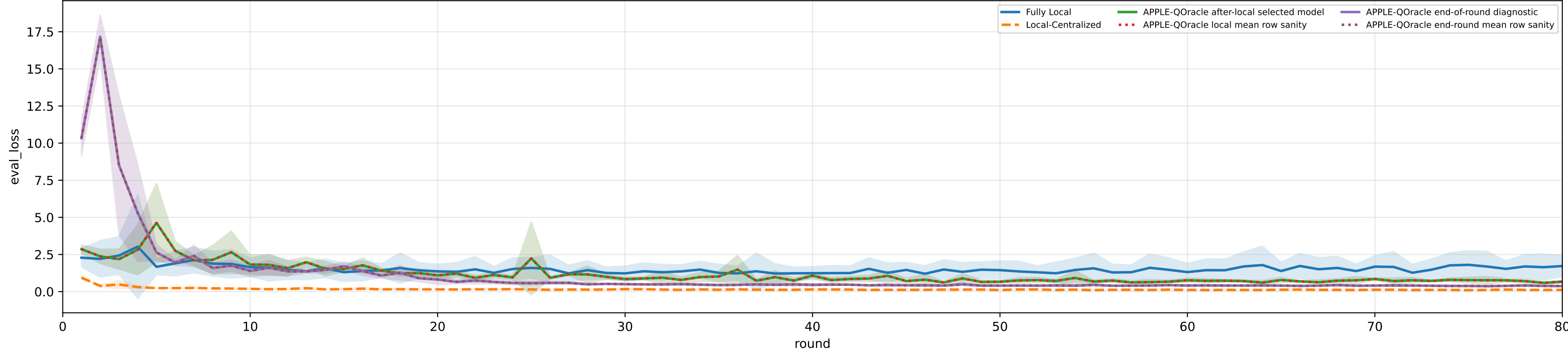
Validation loss: baselines vs selected APPLE-QOracle and end-of-round mismatch (rounds=80)
