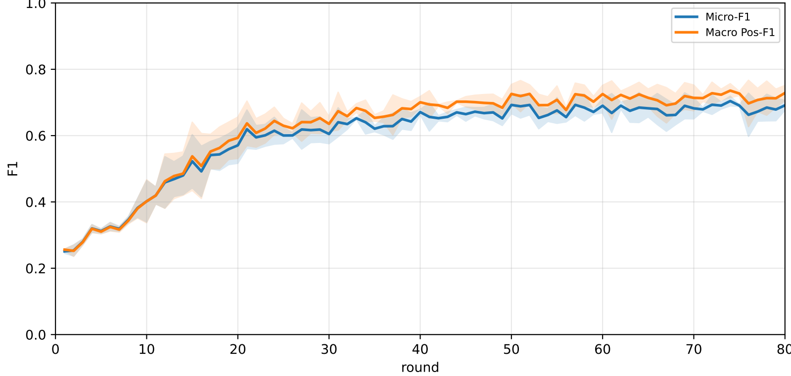
Pooled APPLE-QOracle micro / macro F1 (after-local selected model)
