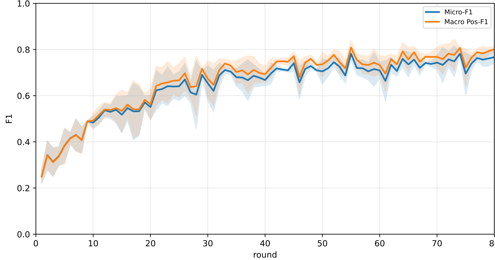
Pooled APPLE-QOracle micro / macro F1 (after-local selected model)
