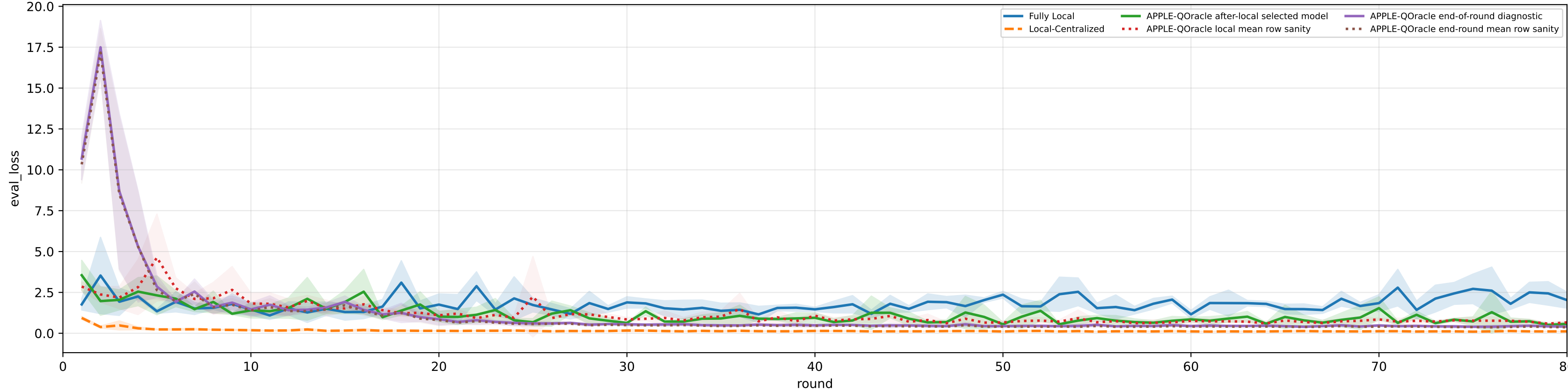
Validation loss: baselines vs selected APPLE-QOracle and end-of-round mismatch (rounds=80)
