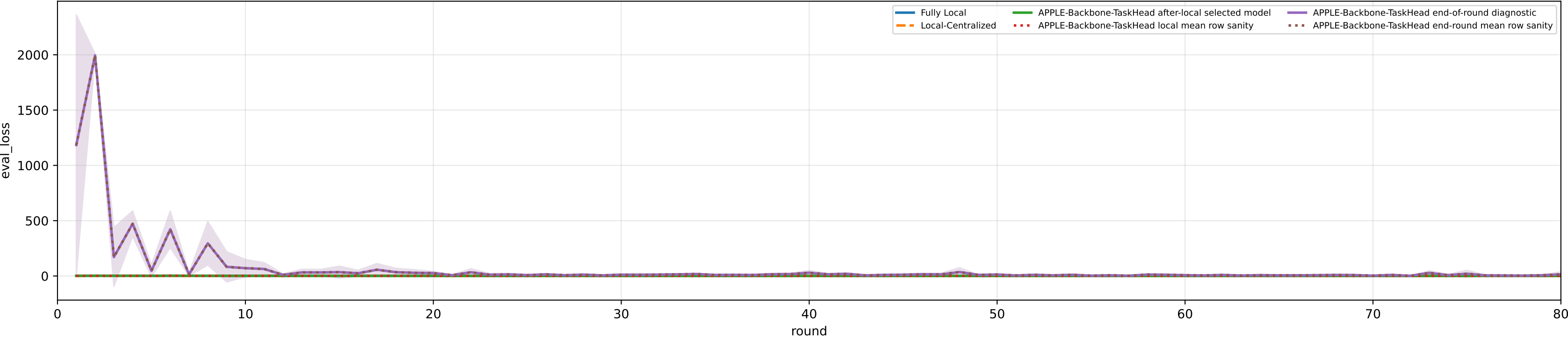
Validation loss: baselines vs selected APPLE-Backbone-TaskHead and end-of-round mismatch (rounds=80)
