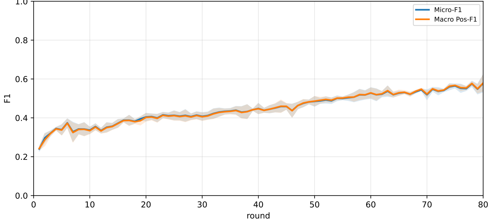
Pooled APPLE-Backbone-TaskHead micro / macro F1 (after-local selected model)
