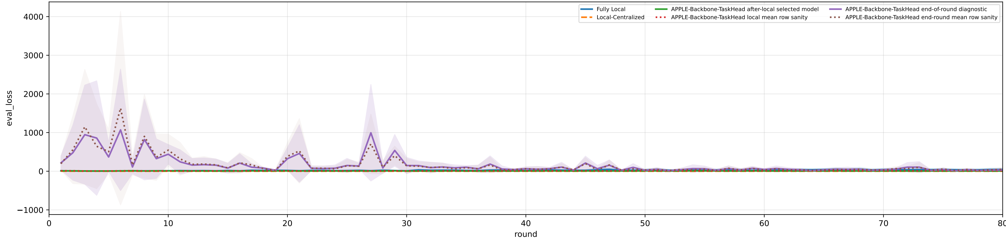
Validation loss: baselines vs selected APPLE-Backbone-TaskHead and end-of-round mismatch (rounds=80)
