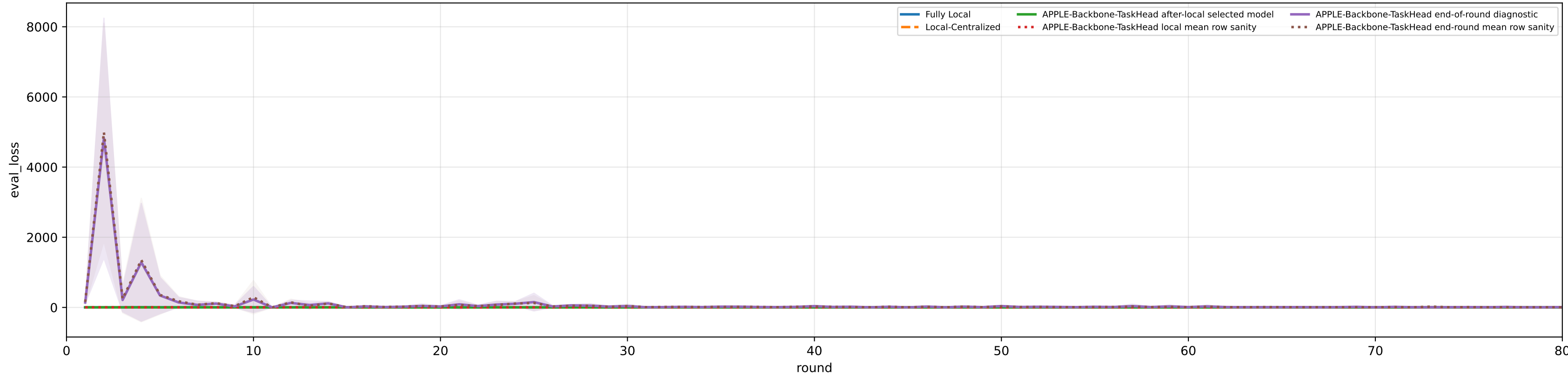
Validation loss: baselines vs selected APPLE-Backbone-TaskHead and end-of-round mismatch (rounds=80)
