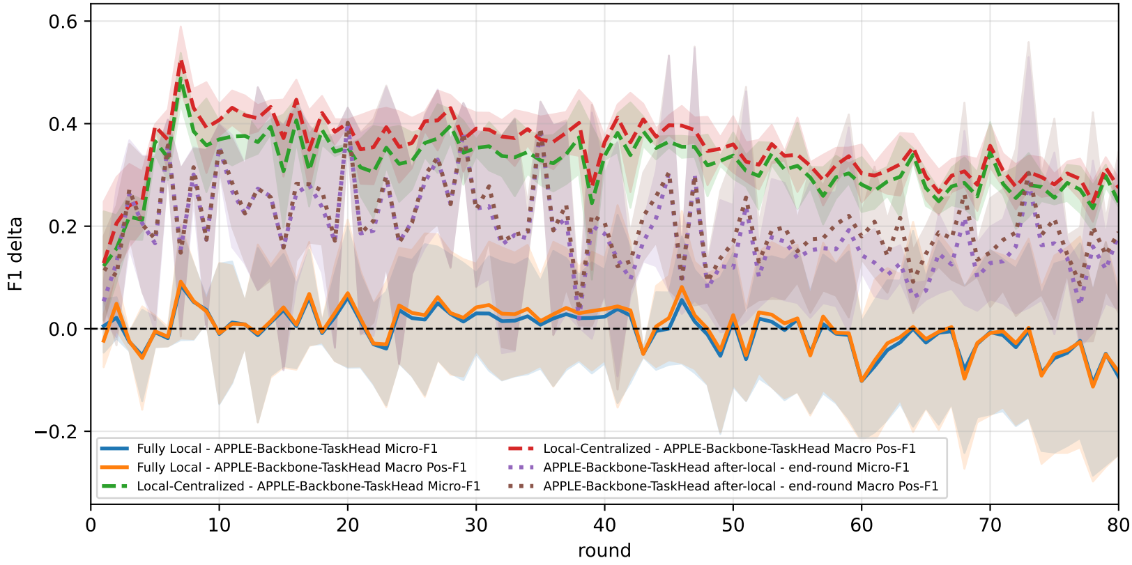
Delta diagnostics: baseline gaps and APPLE-Backbone-TaskHead mismatch gap
