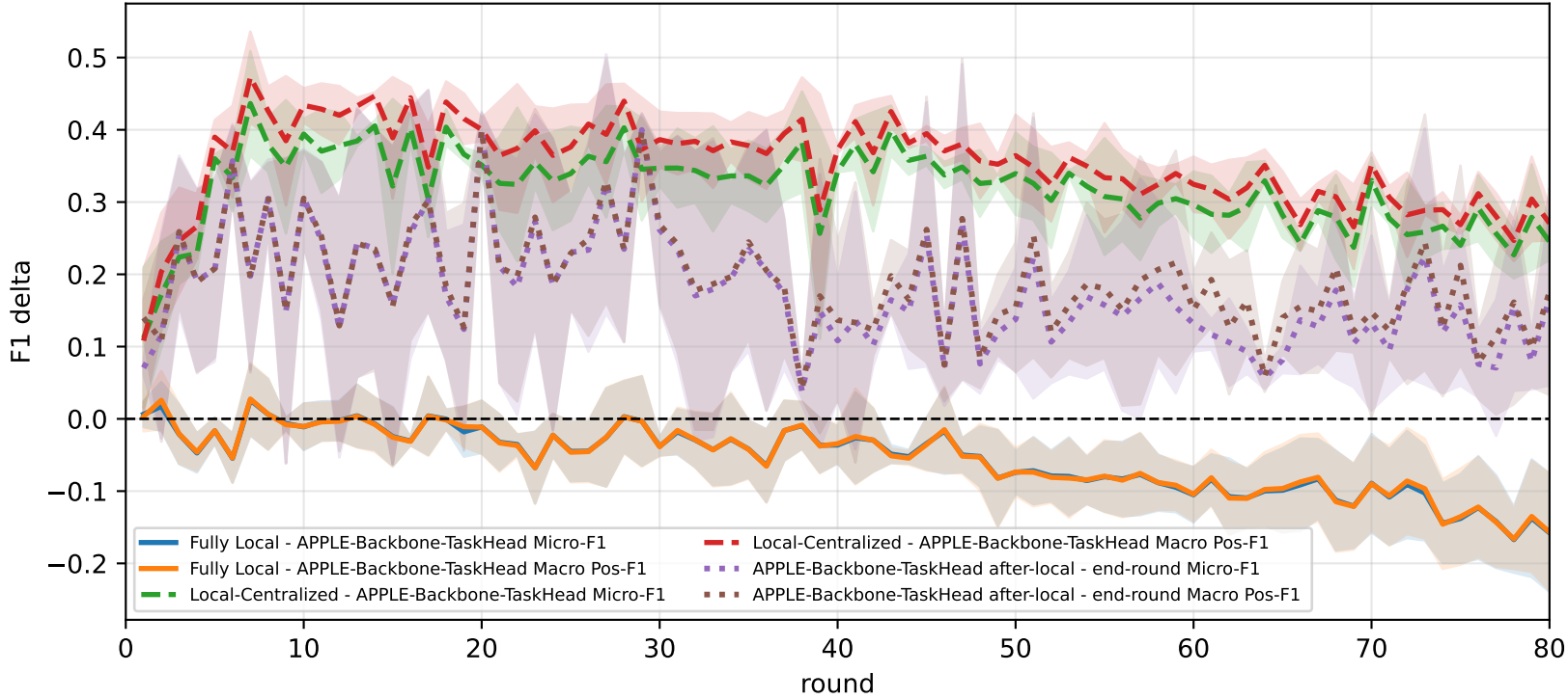
Delta diagnostics: baseline gaps and APPLE-Backbone-TaskHead mismatch gap
