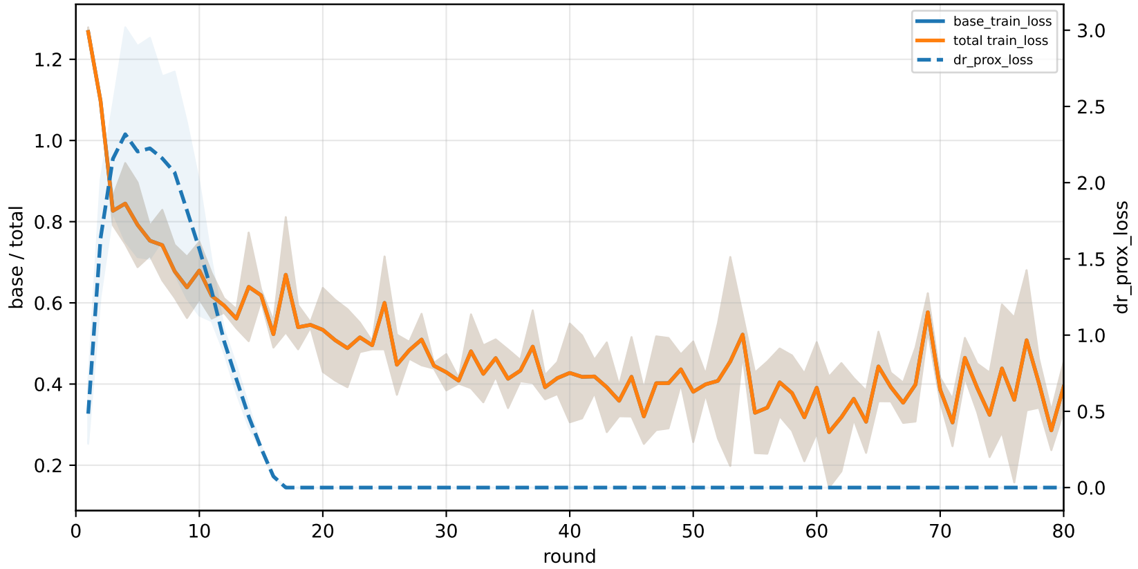
C3-specialist | graph_id=3000011
