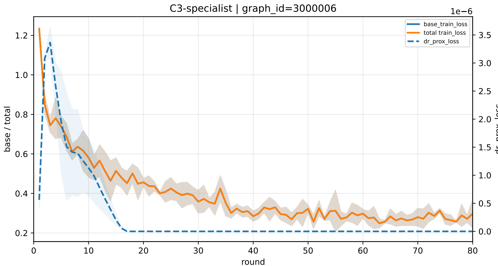
C3-specialist | graph_id=3000006
