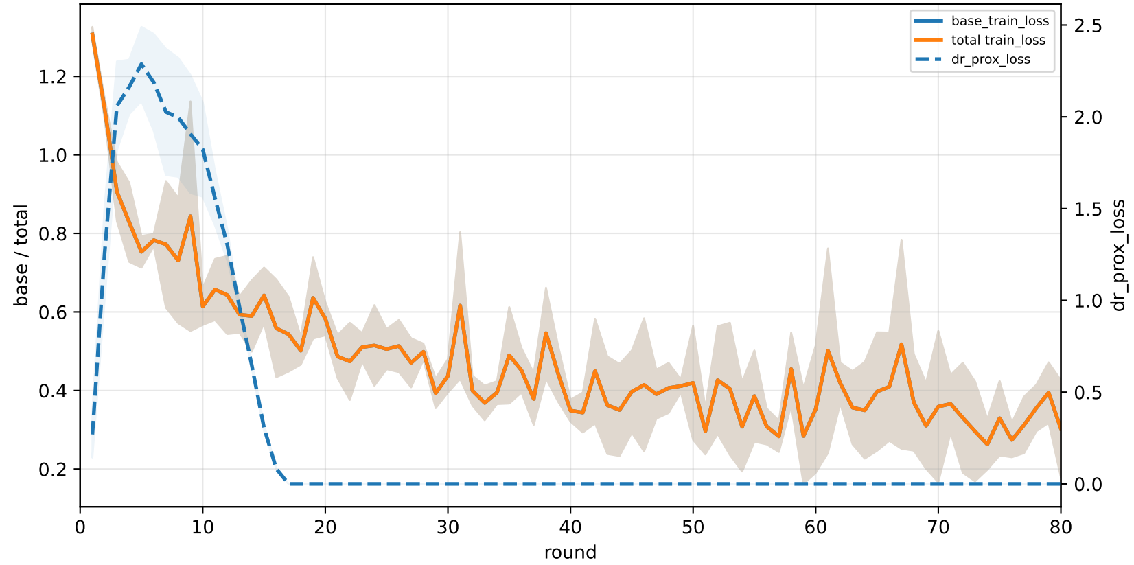
C4-specialist | graph_id=3000012
