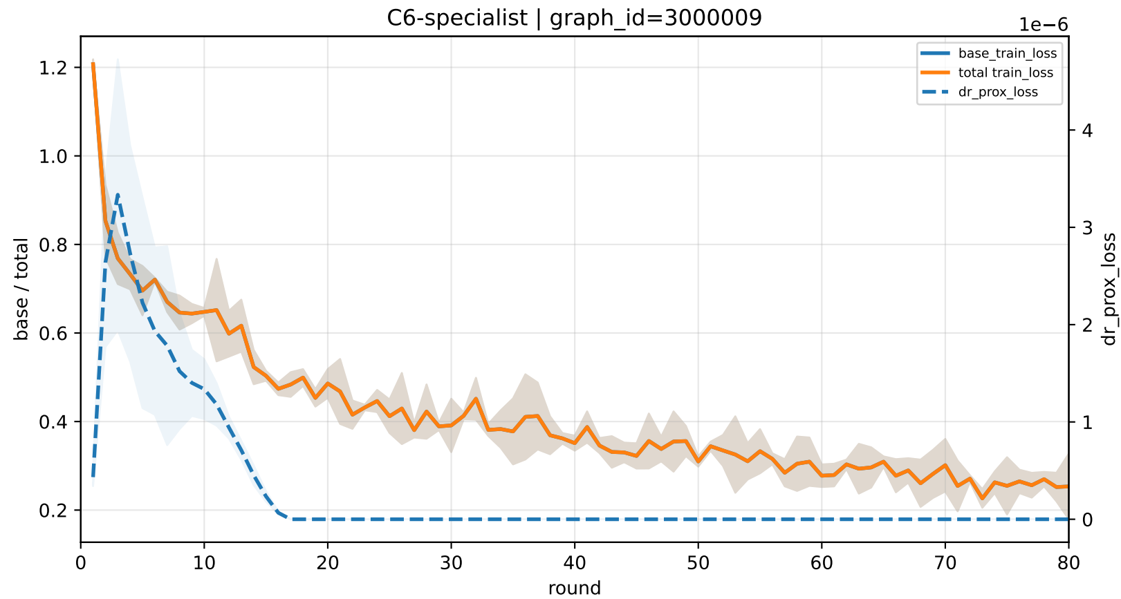
C6-specialist | graph_id=3000009
