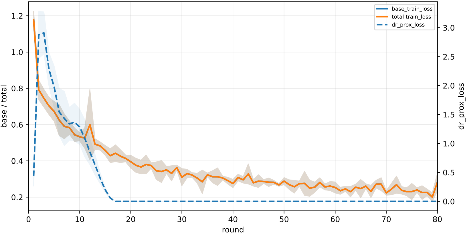
C2-specialist | graph_id=3000000
