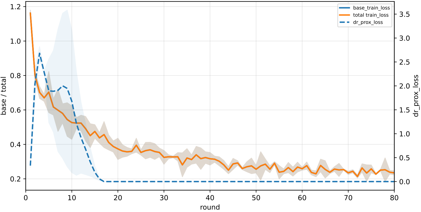
C4-specialist | graph_id=3000002
