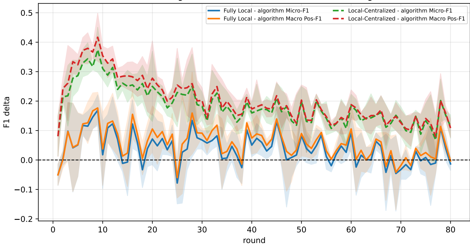
Delta diagnostics: baselines minus FedALA-FedAvg
