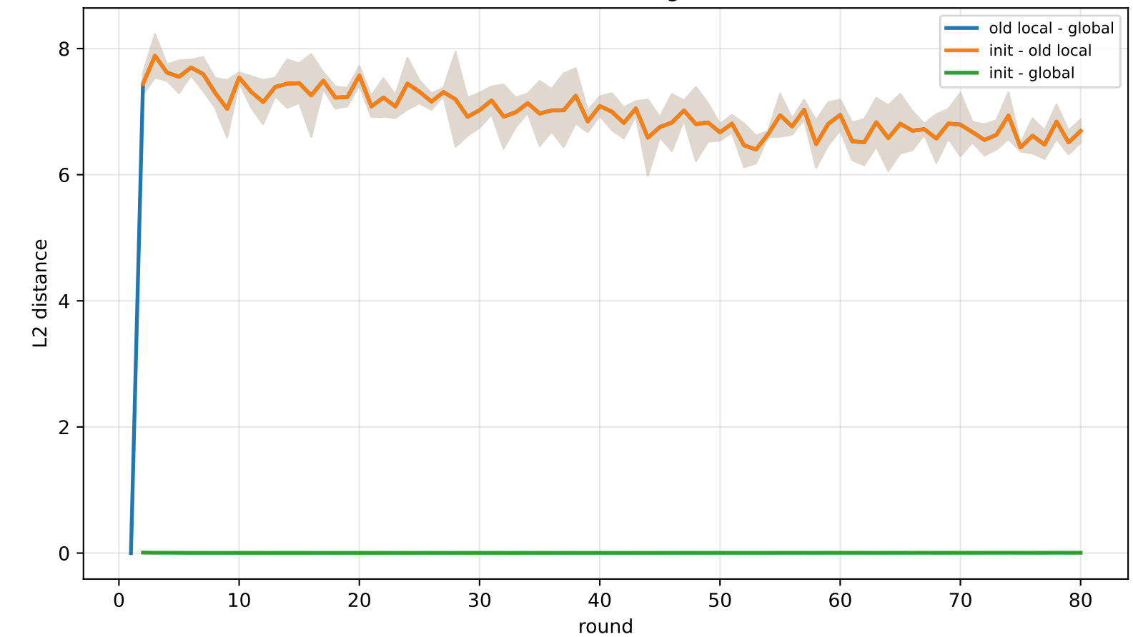
Model distance diagnostics
