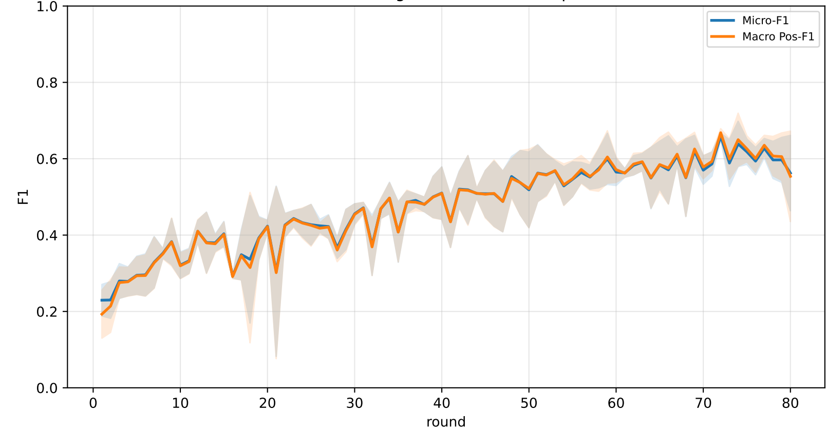
Pooled FedALA-FedAvg micro / macro F1 (personalized)
