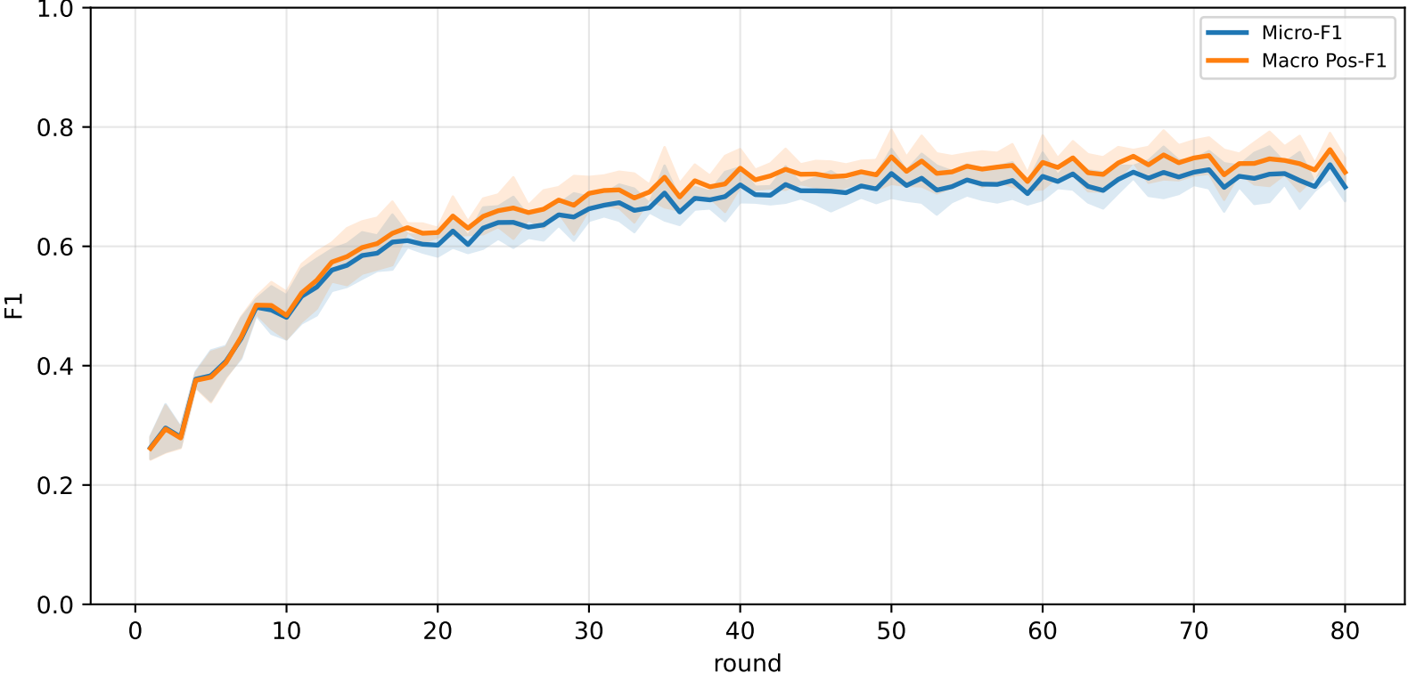
Pooled FedALA-HeadOnly micro / macro F1 (personalized)
