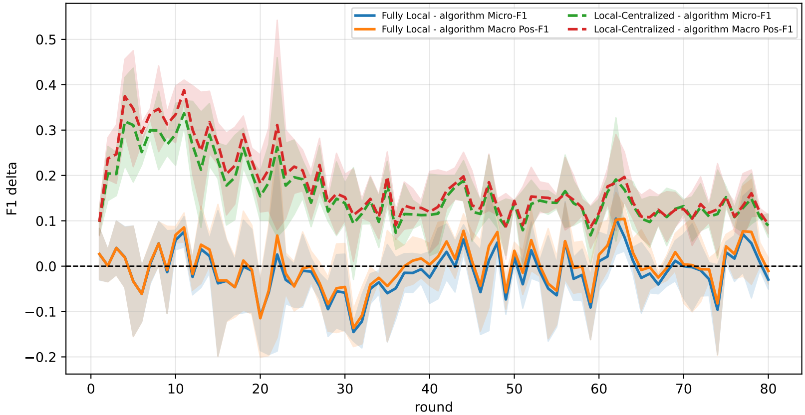
Delta diagnostics: baselines minus FedALA-HeadOnly
