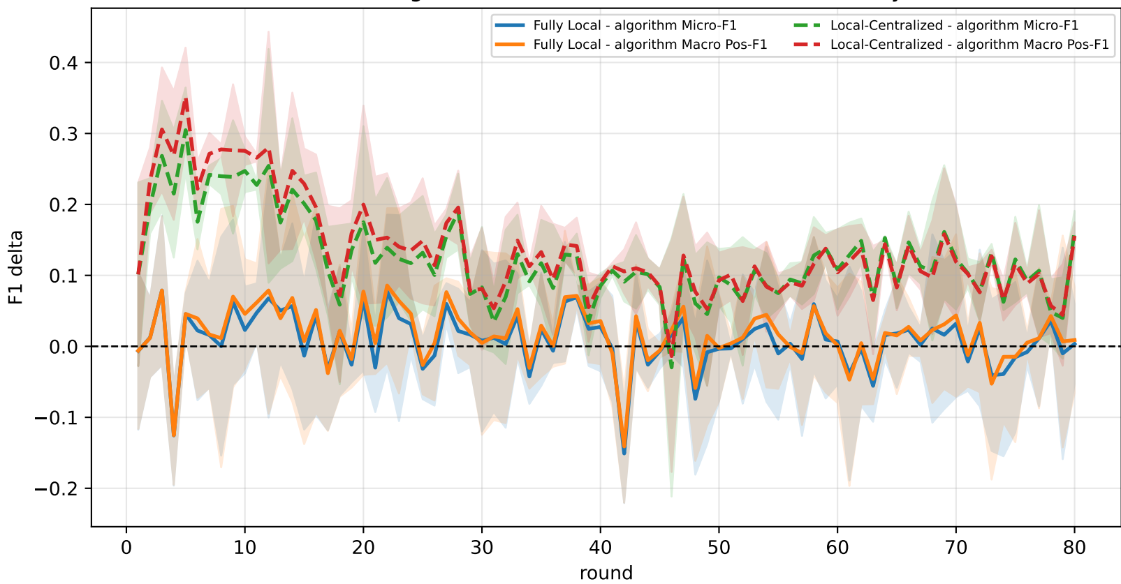
Delta diagnostics: baselines minus FedALA-HeadOnly
