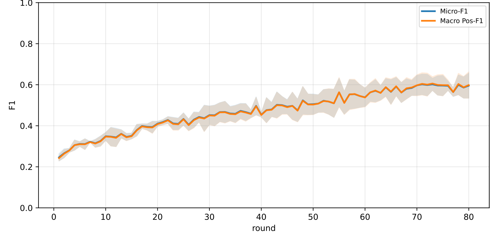
Pooled FedALA-HeadOnly micro / macro F1 (personalized)
