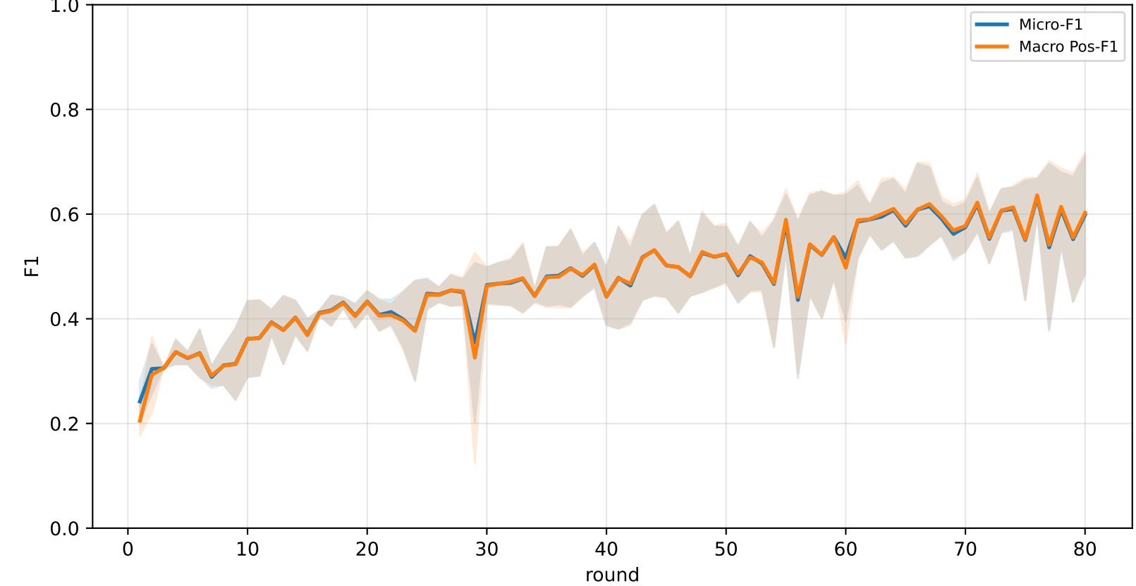
Pooled FedALA-HeadOnly micro / macro F1 (personalized)
