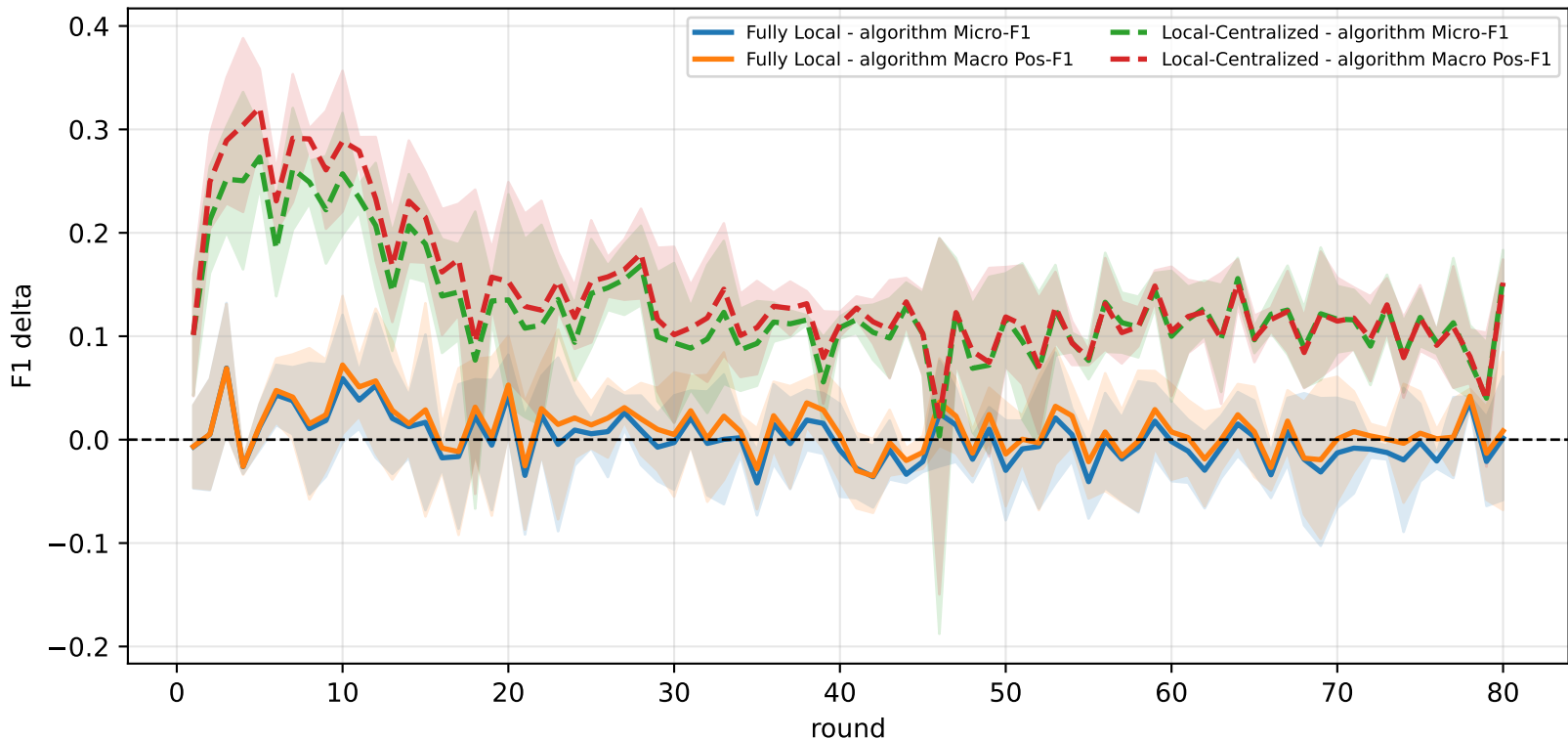
Delta diagnostics: baselines minus FedALA-HeadOnly
