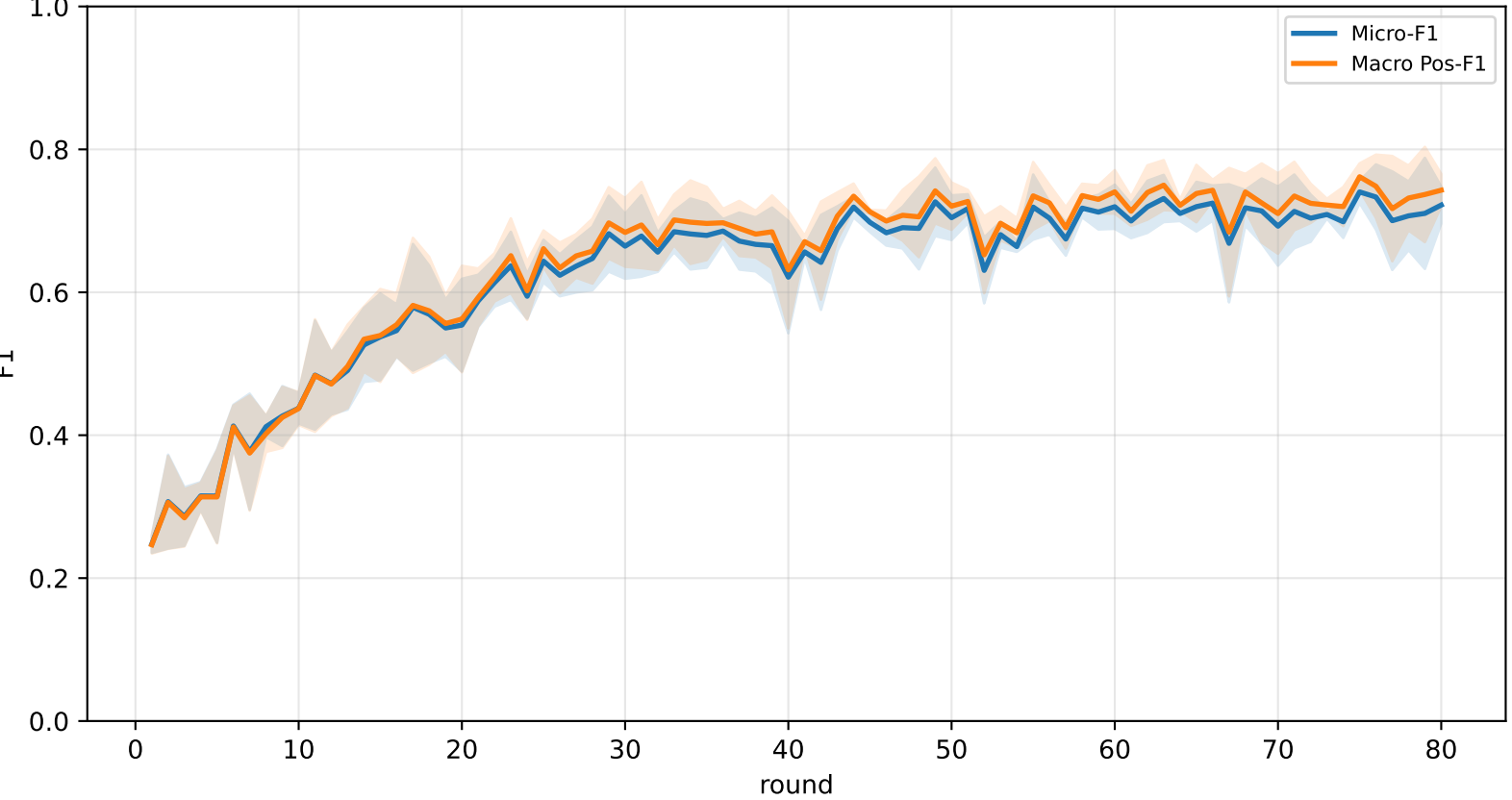
Pooled FedALA-HeadOnly micro / macro F1 (personalized)
