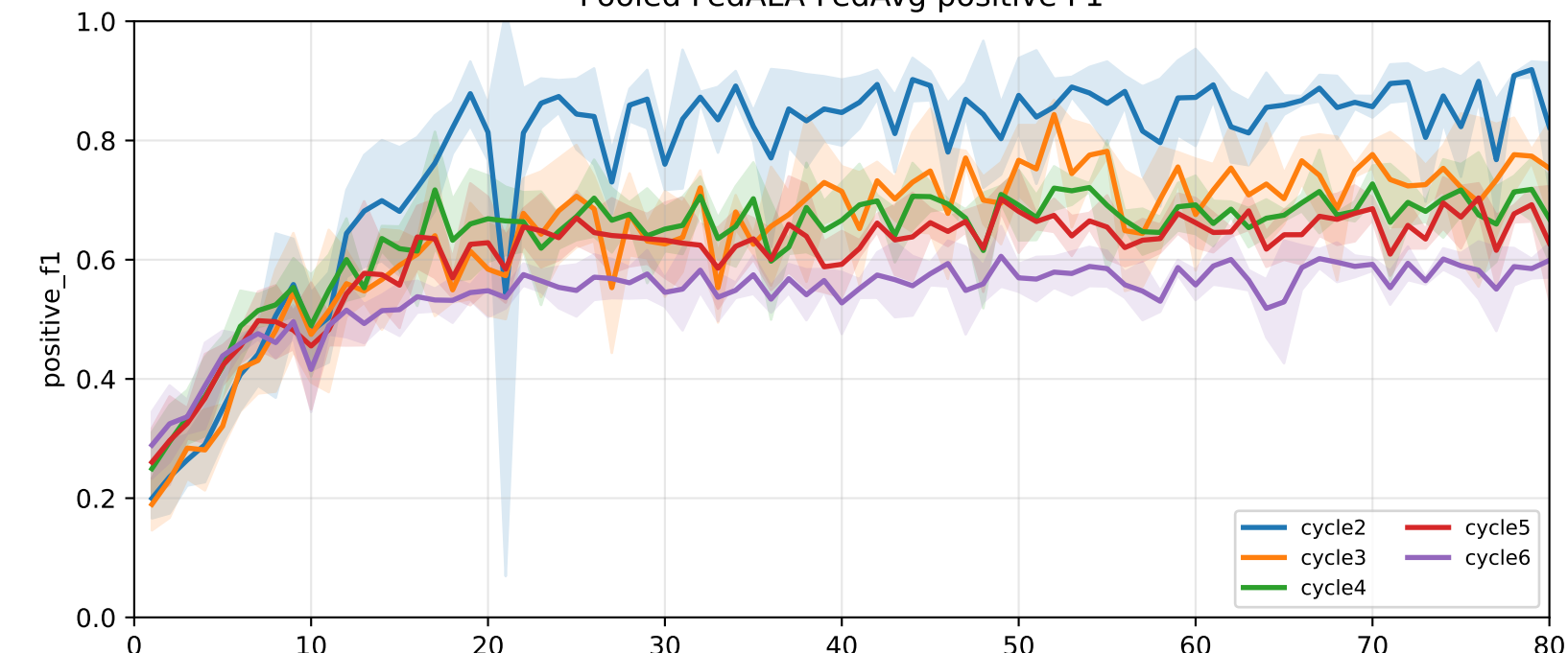
Pooled FedALA-FedAvg positive F1
