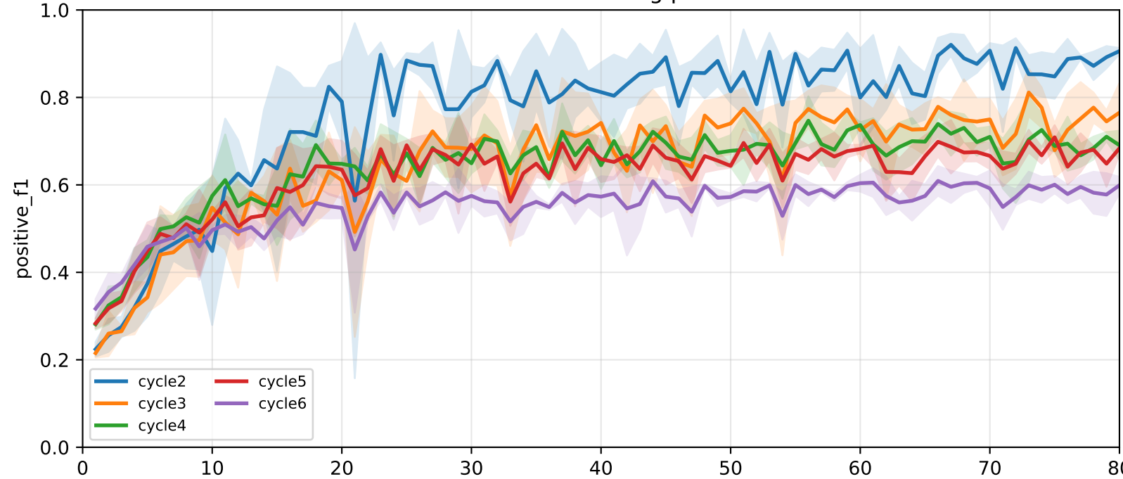
Pooled FedALA-FedAvg positive F1
