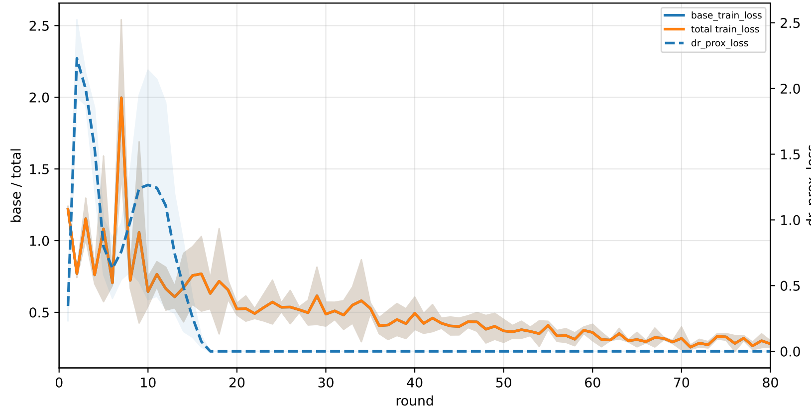
C3-specialist | graph_id=3000001
