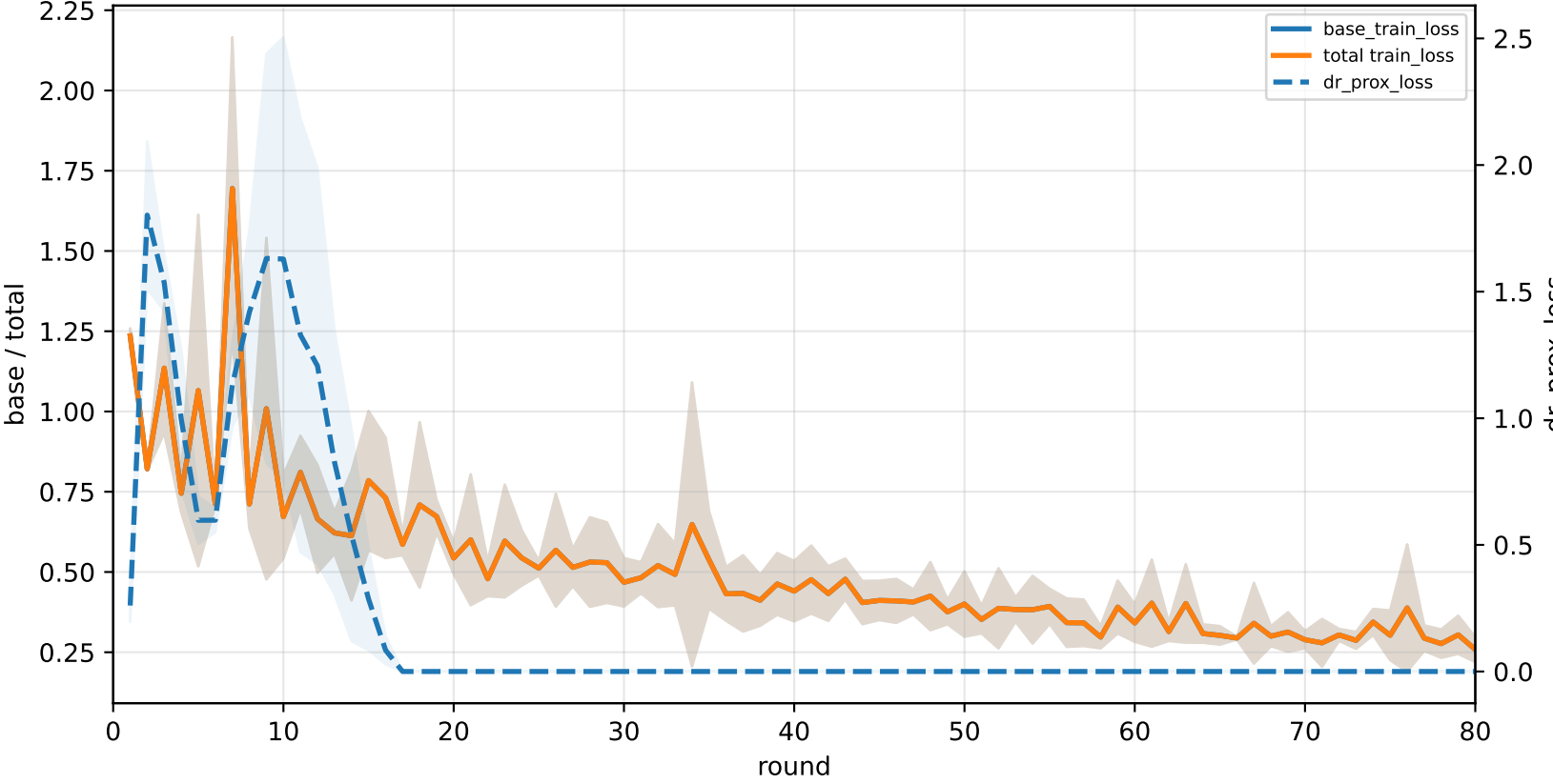
C5-specialist | graph_id=3000003
