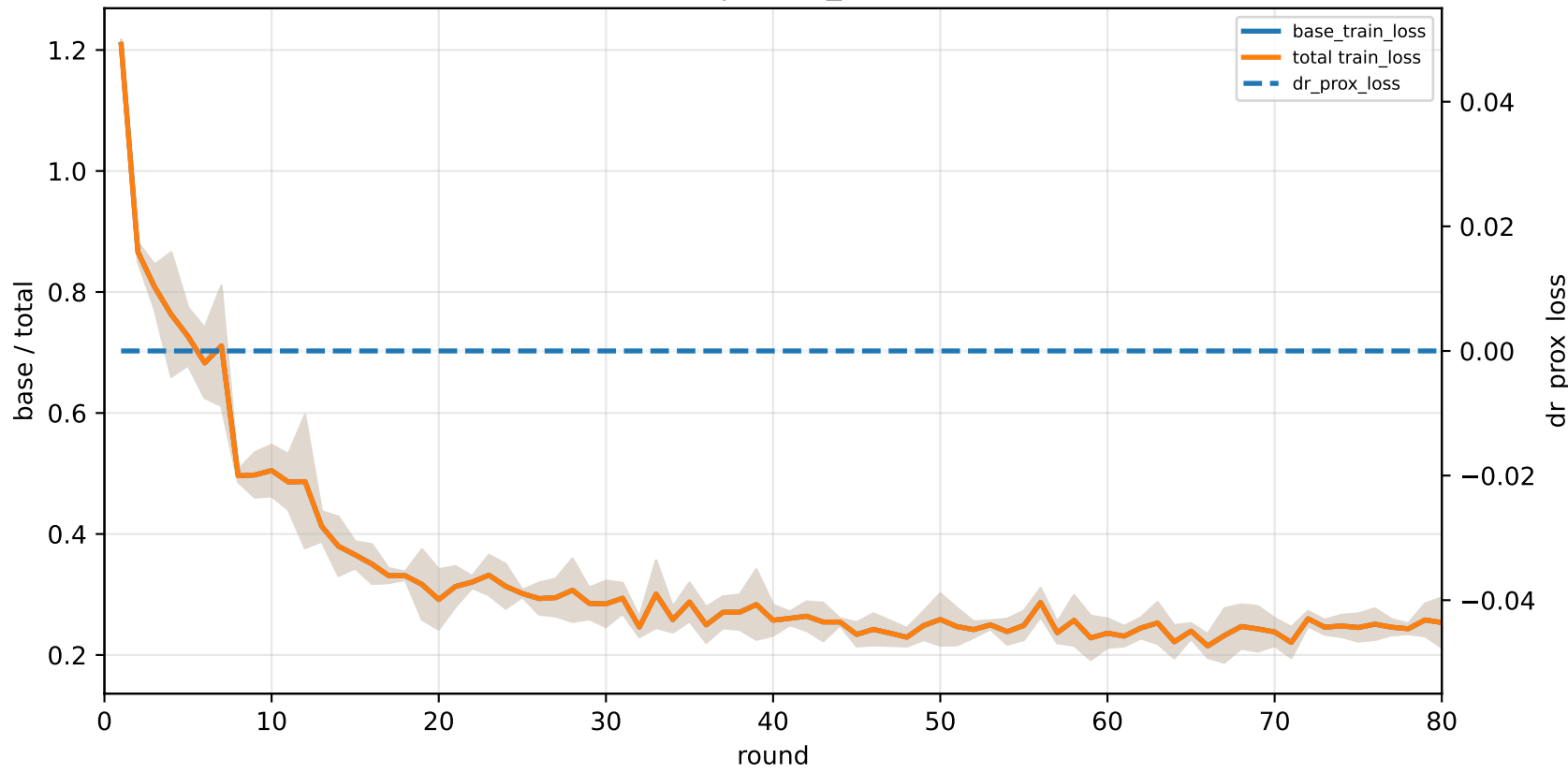
C5-specialist | graph_id=3000003
