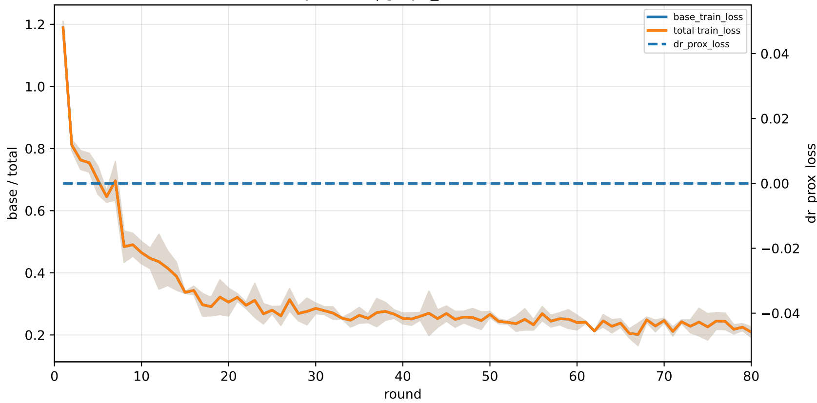
C3-specialist | graph_id=3000001
