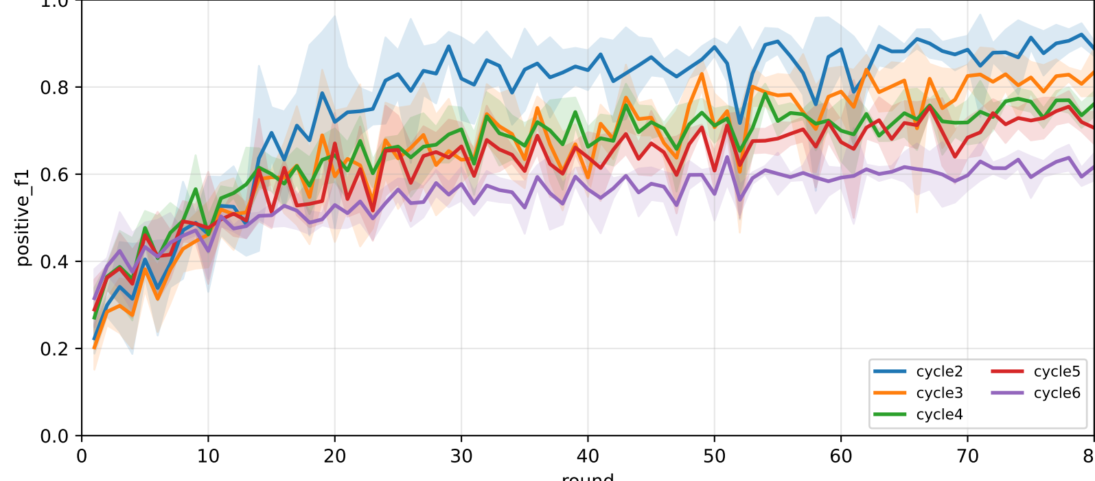
Pooled APPLE-Qinit positive F1 (after-local selected model, rounds=80)
