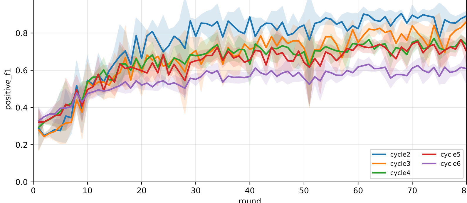
Pooled APPLE-QInit positive F1 (after-local selected model, rounds=80)
