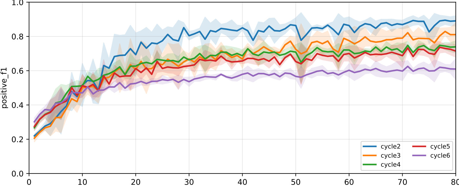
Pooled APPLE-QInit positive F1 (after-local selected model, rounds=80)
